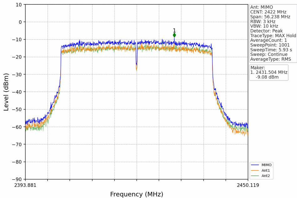
802.11ax(HEW40)_LCH_2422MHz_RU484_Left_MIMO_NTNV
