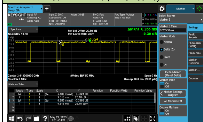
802.11n-HT20 (T = 5.430ms)
