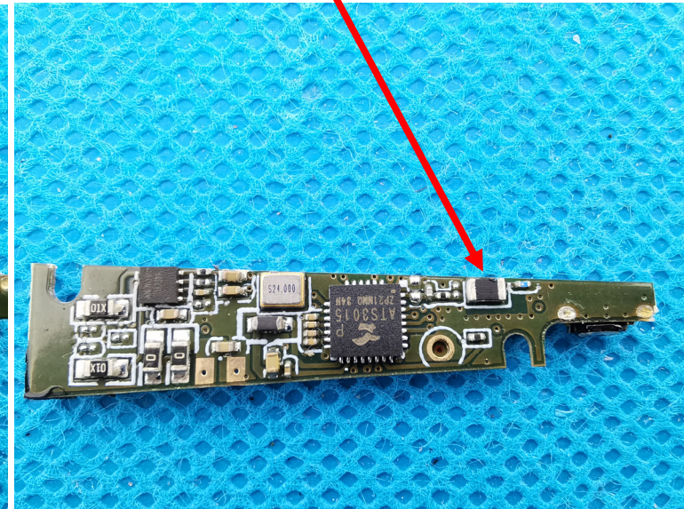
Chip Antenna
