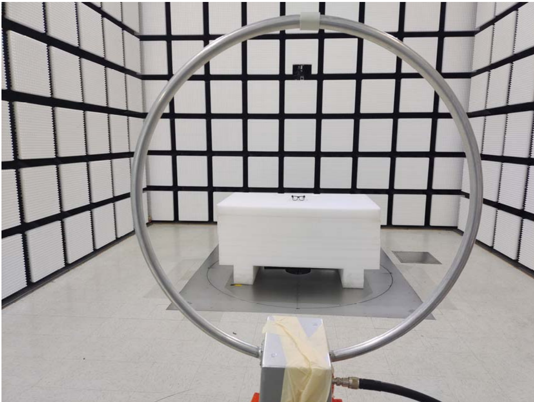
Radiated Emission 9kHz to 30MHz Parallel
