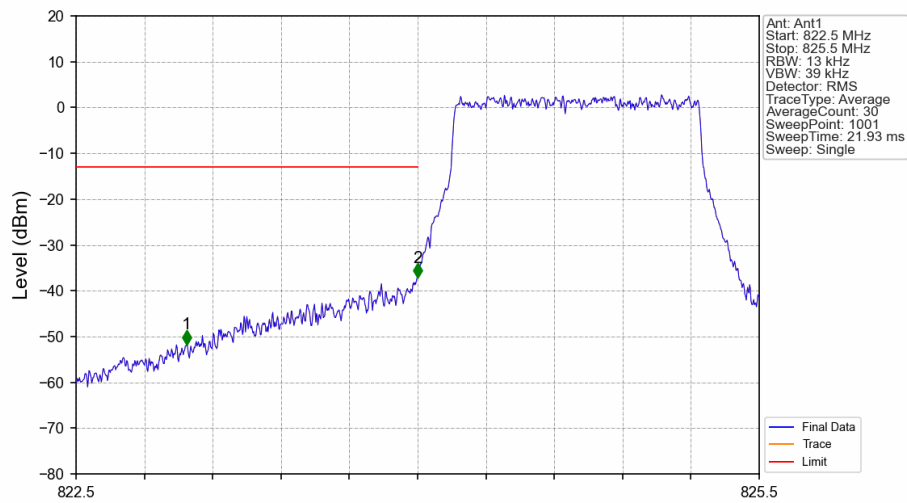
Band5_1.4MHz_16QAM_LCH_824.7MHz_RB_6_0_NTNV
