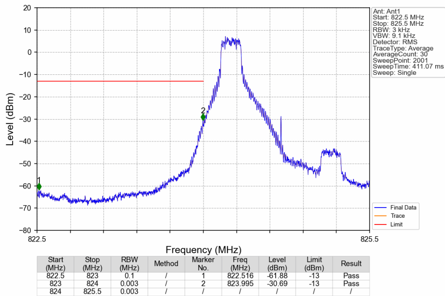
Band5_1.4MHz_QPSK_LCH_824.7MHz_RB_1_0_NTNV
