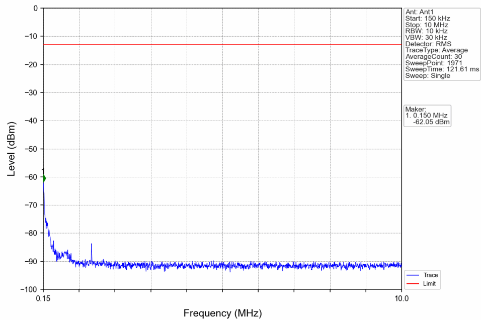
Band5_1.4MHz_16QAM_LCH_824.7MHz_RB_6_0_NTNV
