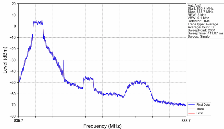
Band5_1.4MHz_16QAM_MCH_836.5MHz_RB_1_0_NTNV
