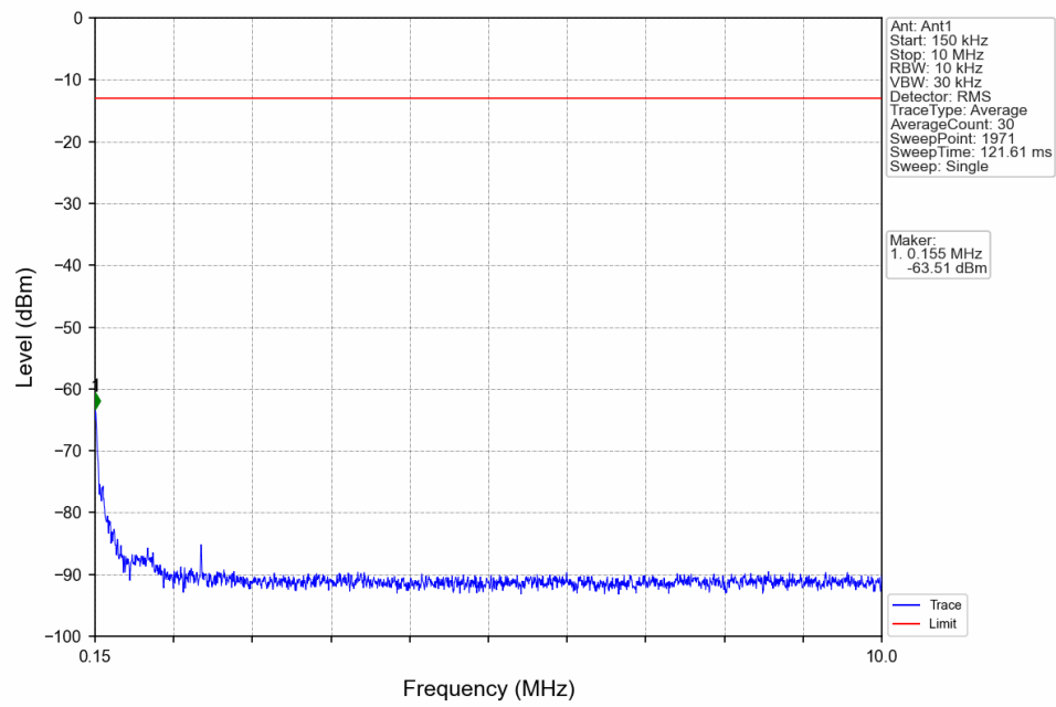
Band5_1.4MHz_QPSK_MCH_836.5MHz_RB_1_0_NTNV
