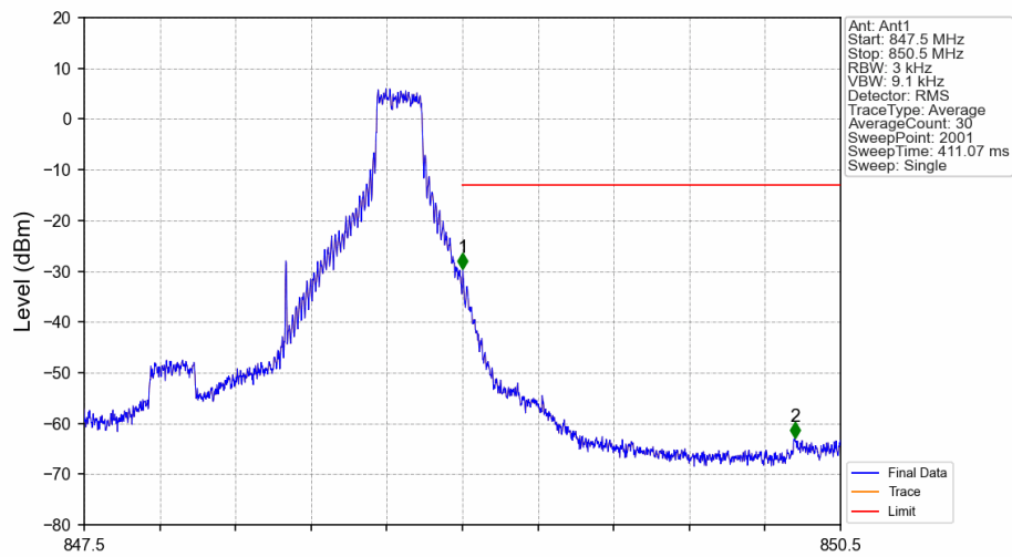
Band5_1.4MHz_QPSK_HCH_848.3MHz_RB_1_5_NTNV
