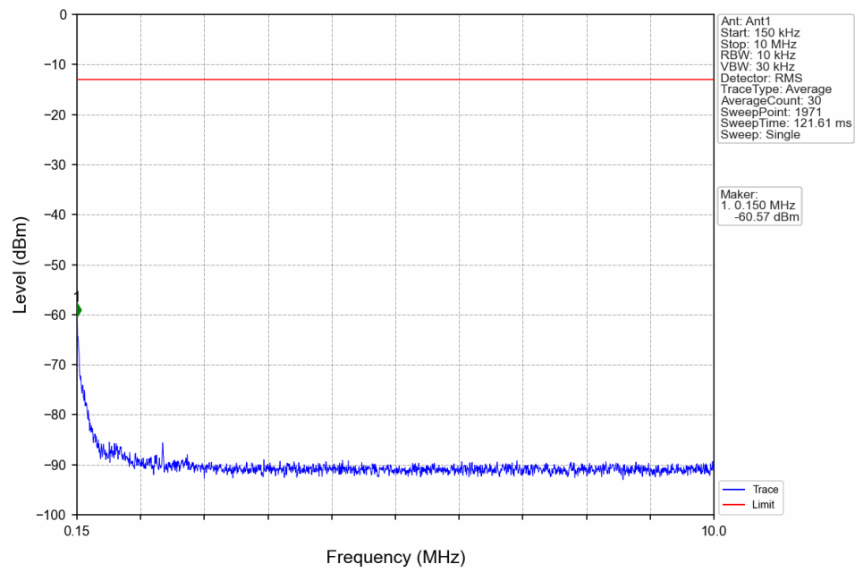
Band5_1.4MHz_QPSK_LCH_824.7MHz_RB_1_0_NTNV
