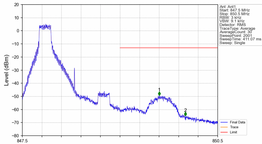
Band5_1.4MHz_16QAM_HCH_848.3MHz_RB_1_0_NTNV
