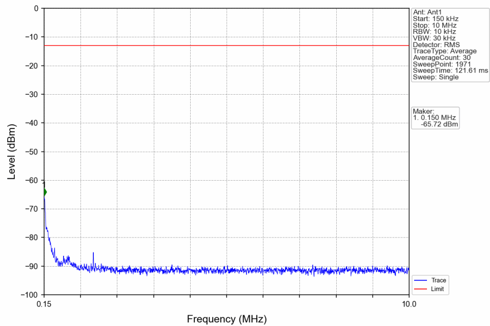
Band5_1.4MHz_QPSK_HCH_848.3MHz_RB_1_5_NTNV
