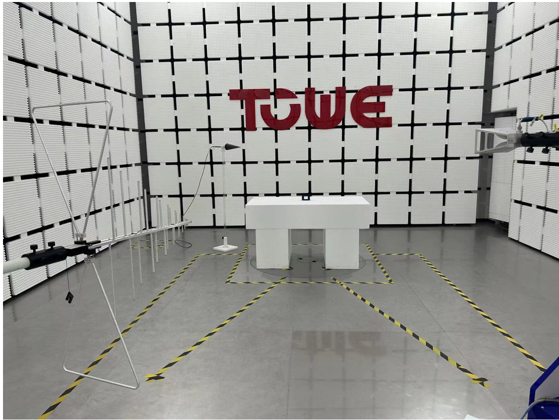
Radiated Spurious Emissions (GSM/WCDMA/LTE) Below1G
