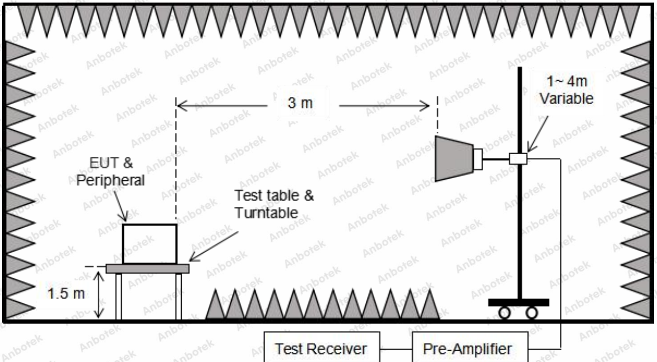
Figure 3. Above 1 GHz
