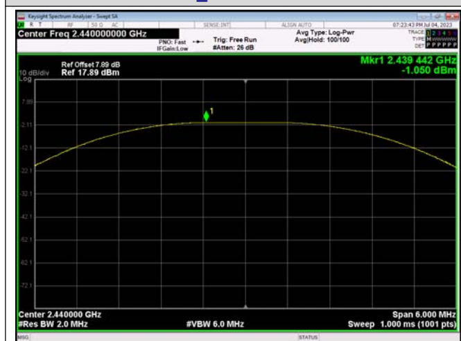
Peak Output Power 2LE_Channel 19
