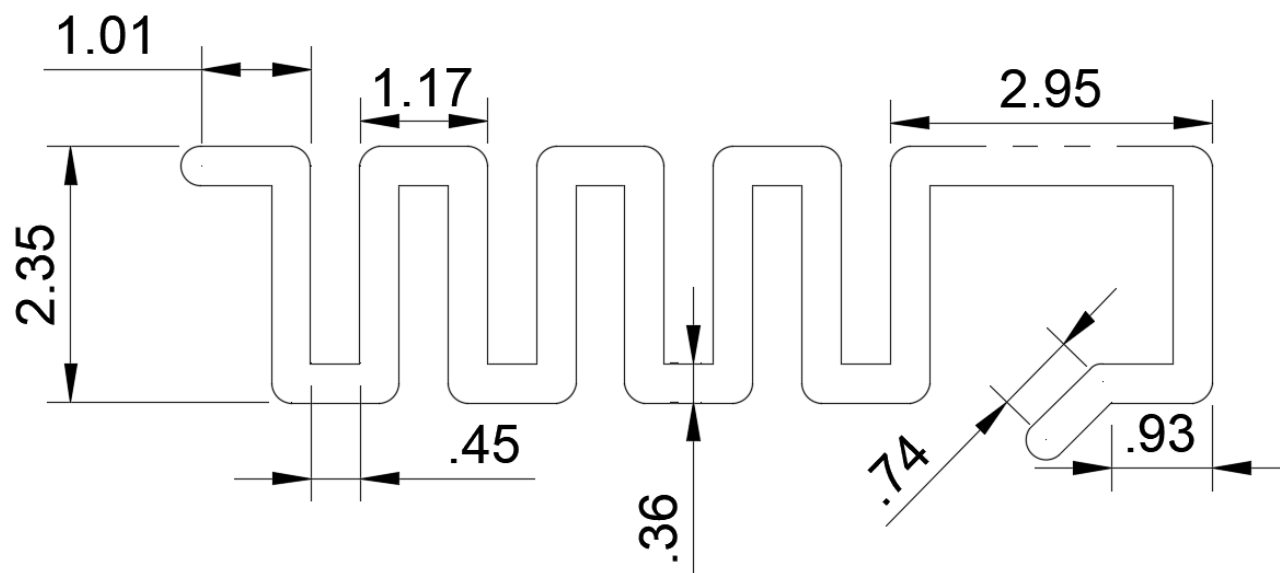
Fig 5.1.1 PCB trace Antenna dimensions
