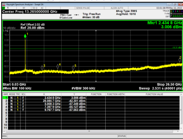
802.11b-Middle channel
