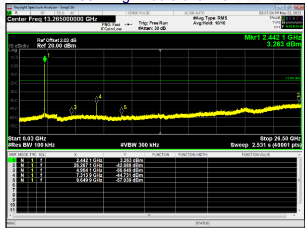
802.11g-Middle channel
