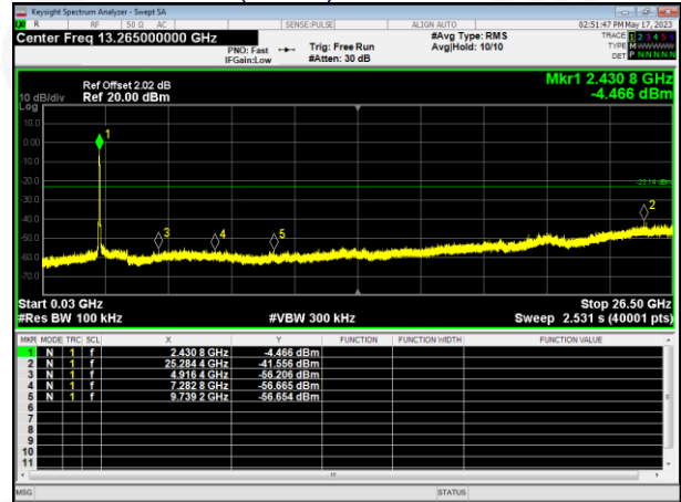
802.11n(HT40)-Lowest channel
