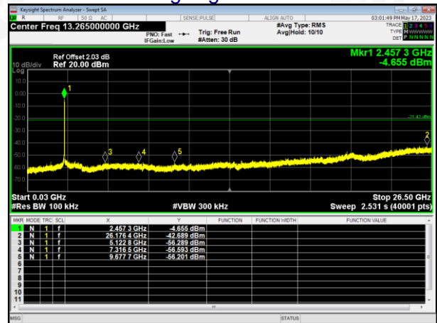
802.11g-Highest channel
