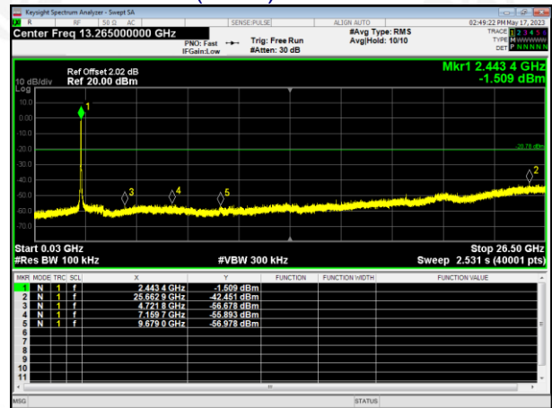
802.11n(HT40)-Middle channel
