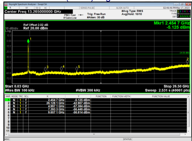
802.11n(HT40)-Highest channel
