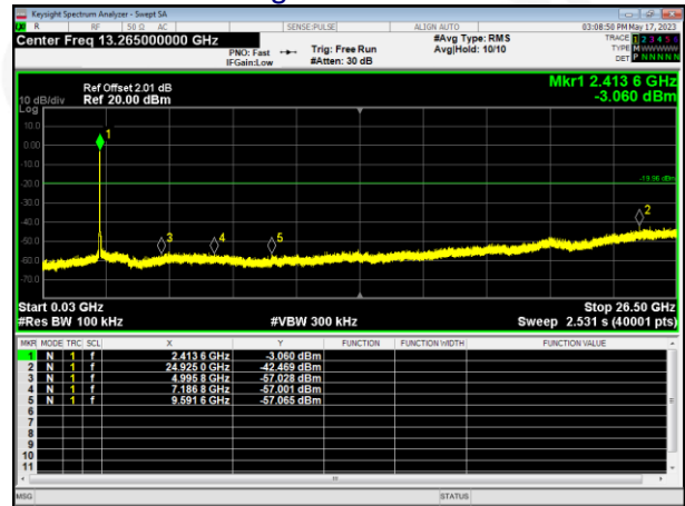
802.11g-Lowest channel
