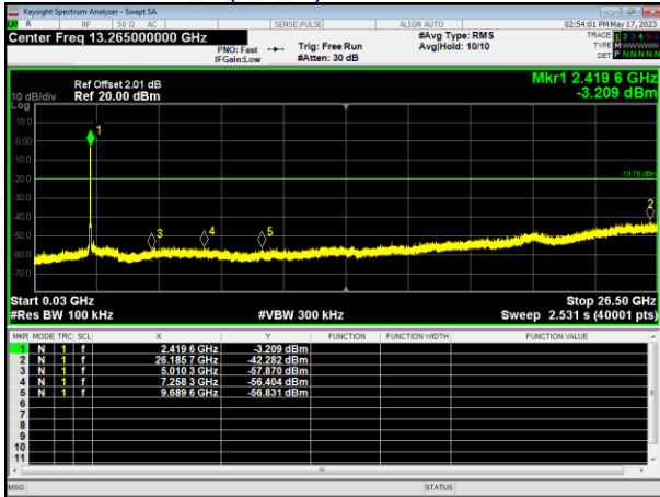
802.11n(HT20)-Lowest channel
