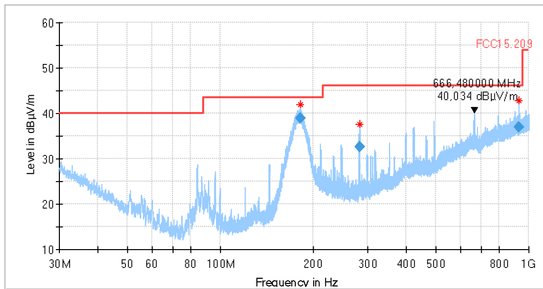
Plot 2: 30 MHz – 1 GHz, horizontal / vertical polarization
