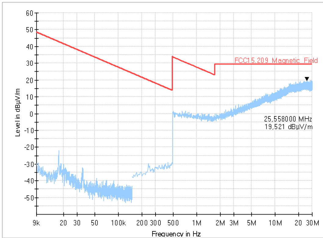
Plot 1: 9 kHz – 30 MHz, horizontal / vertical polarization
