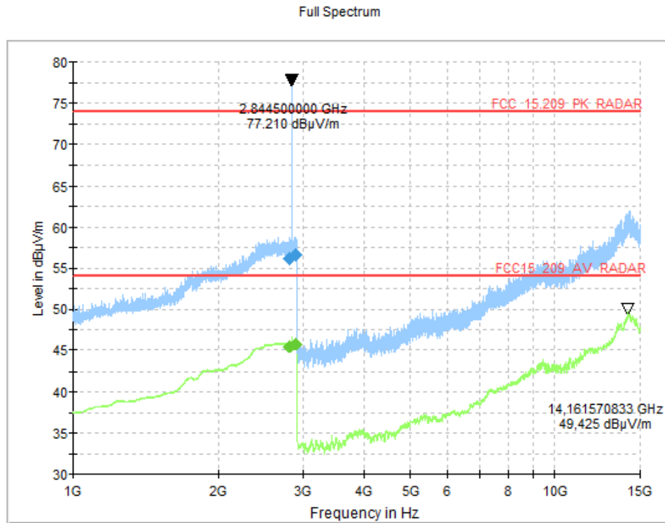
Plot 3: 1 GHz – 15 GHz, horizontal / vertical polarization
