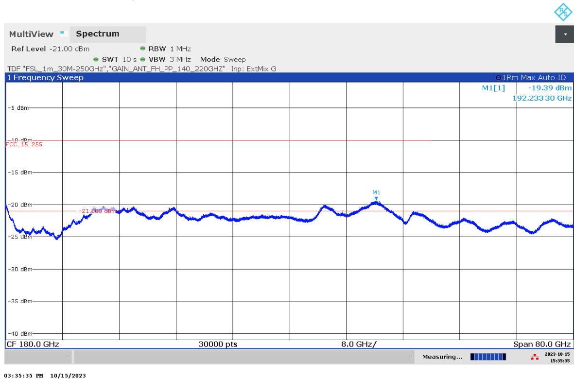
Plot 10: 140 GHz – 220 GHz, antenna vertical / horizontal
