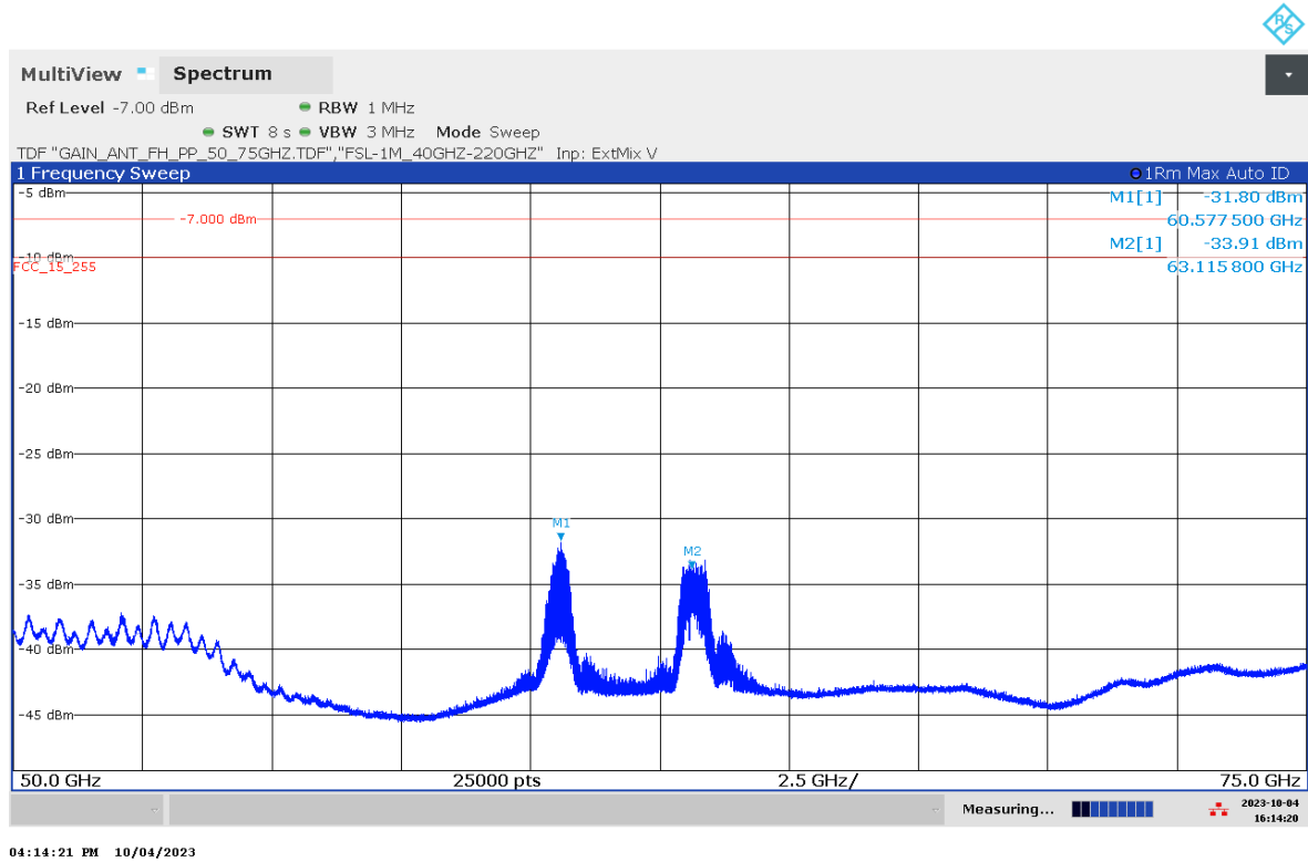
Plot 7: Out of Band 50 GHz – 75 GHz, antenna vertical / horizontal, final scan with RMS detector
