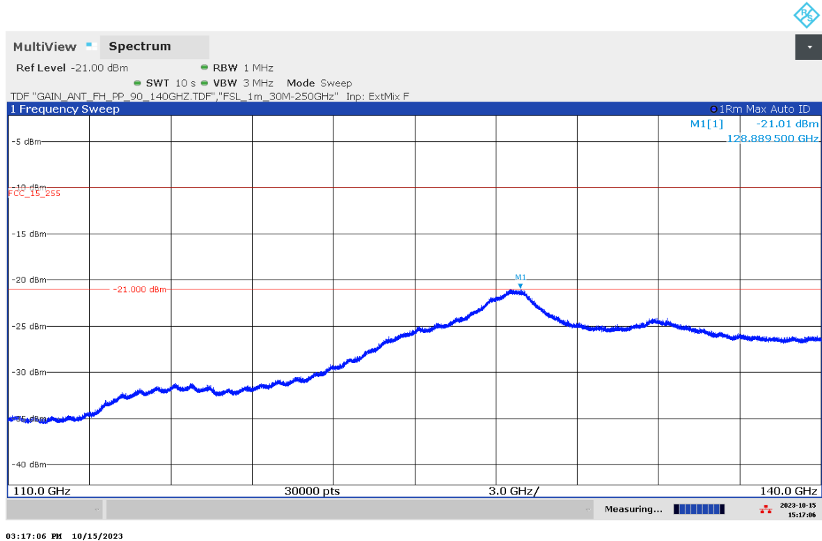
Plot 9: 110 GHz – 140 GHz, antenna vertical / horizontal
