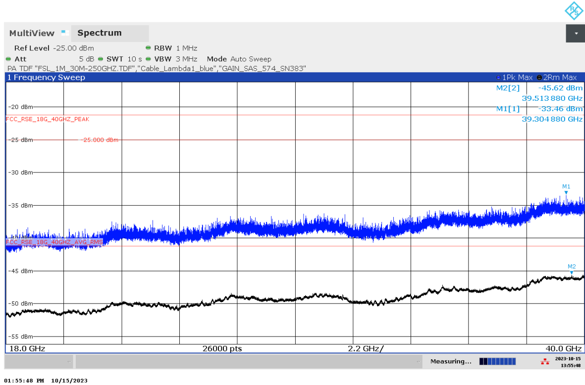
Plot 5: 18 GHz – 40 GHz, horizontal / vertical polarization
