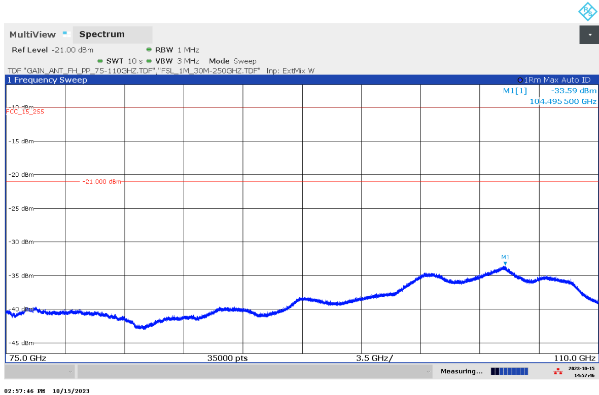
Plot 8: 75 GHz – 110 GHz, antenna vertical / horizontal
