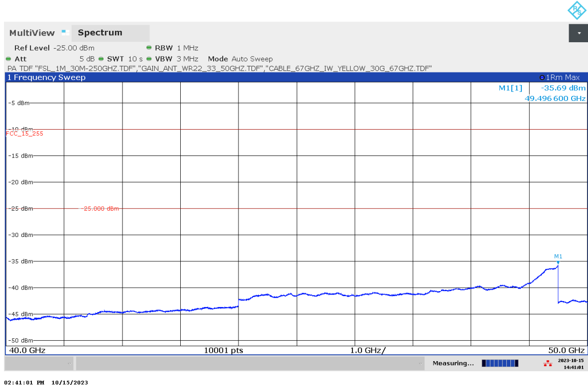
Plot 6: 40 GHz – 50 GHz, antenna vertical / horizontal
