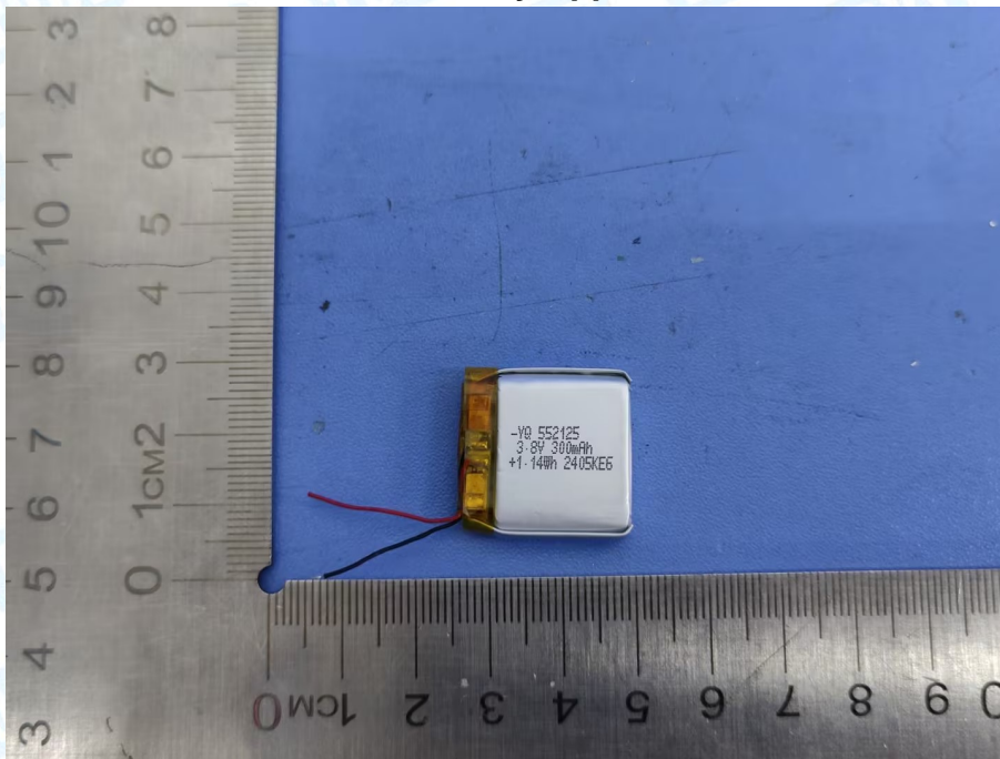
Photo 10 Battery Appearance
