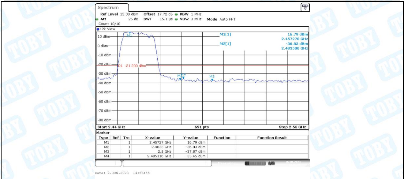
11G-CDD_Ant2_High_2462_Peak
