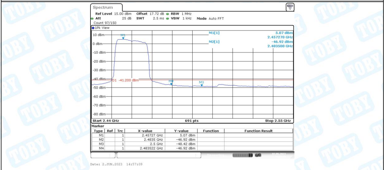
11G-CDD_Ant2_High_2462_AV
