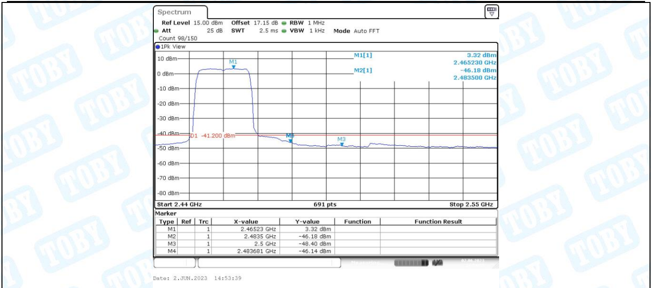
11G-CDD_Ant1_High_2462_AV
