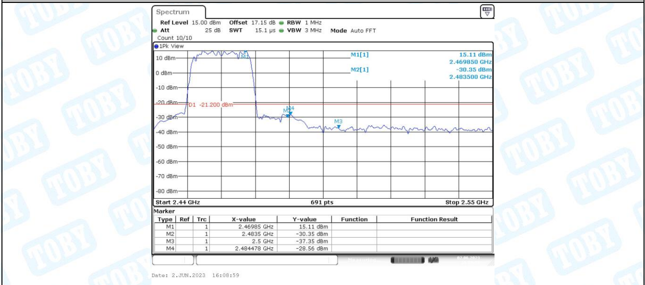
11AX20MIMO_Ant1_High_2462_Peak
