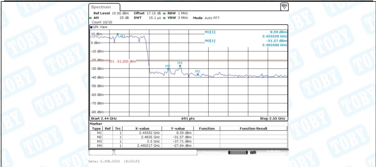
11AX40MIMO_Ant1_High_2452_Peak
