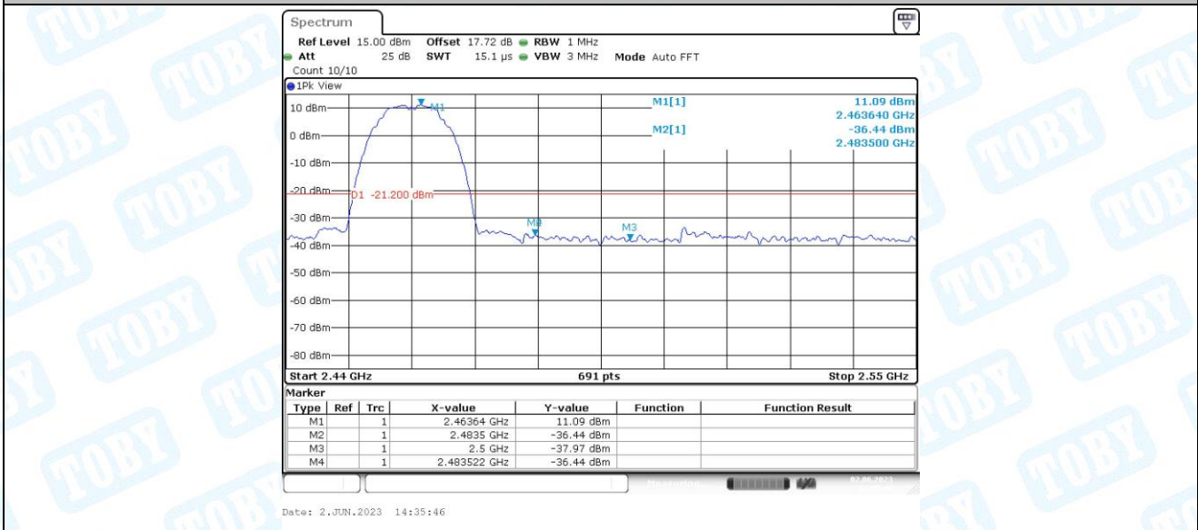
11B-CDD_Ant2_High_2462_Peak
