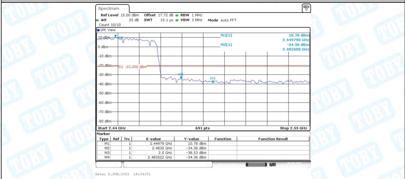
11AX40MIMO_Ant2_High_2452_Peak
