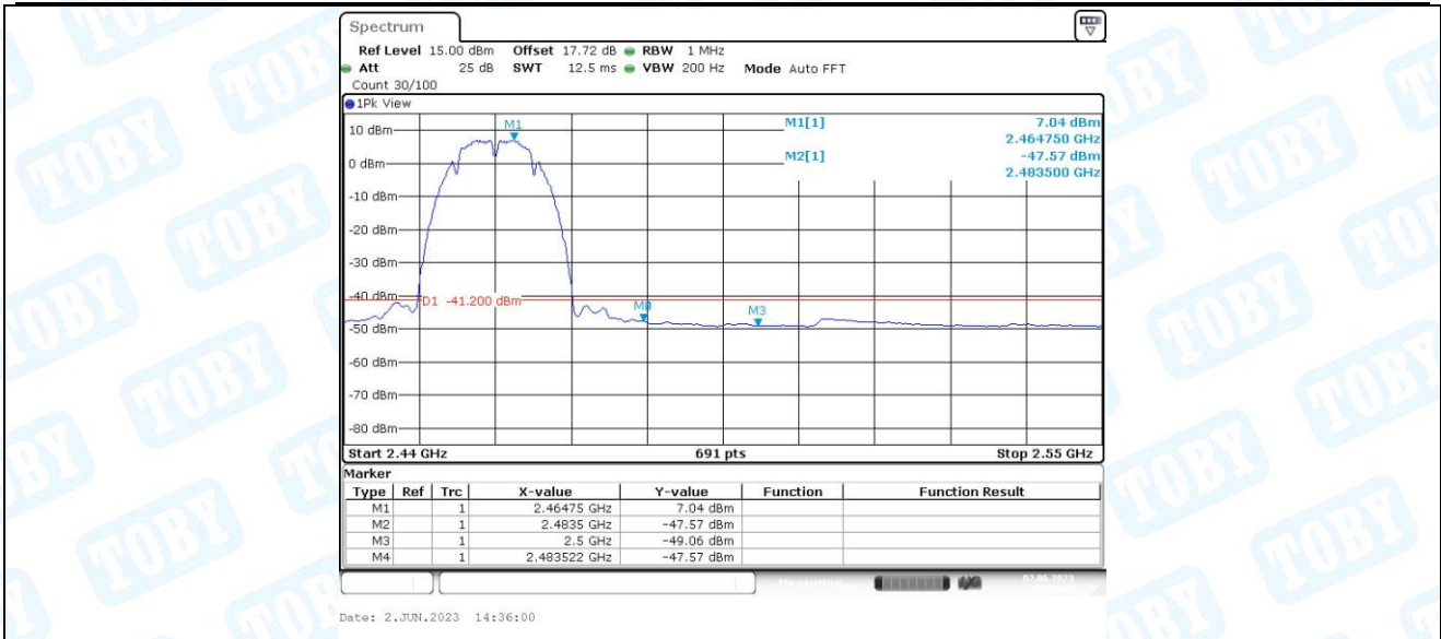
11B-CDD_Ant2_High_2462_AV
