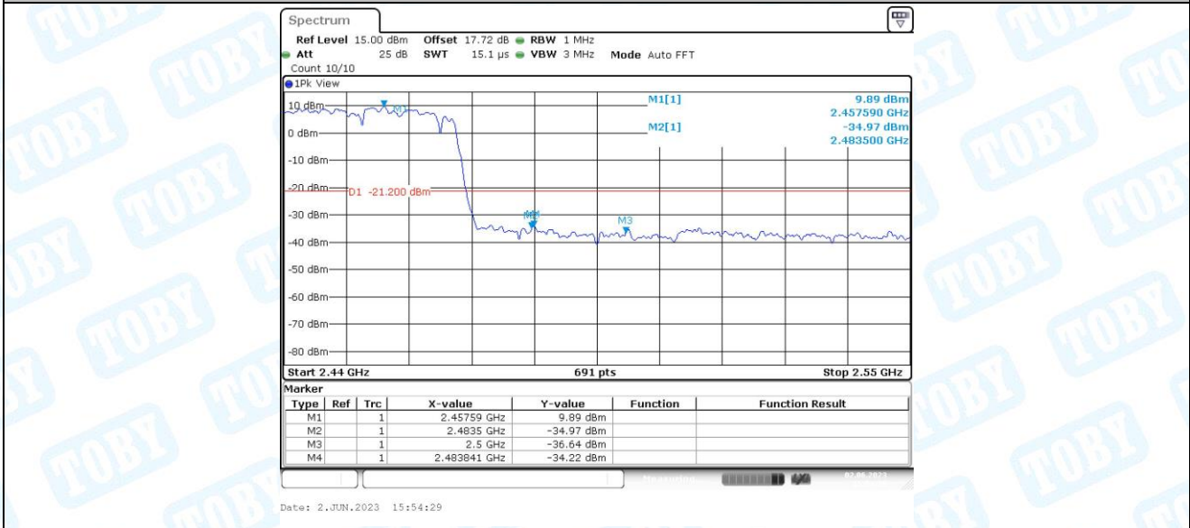
11N40MIMO_Ant2_High_2452_Peak
