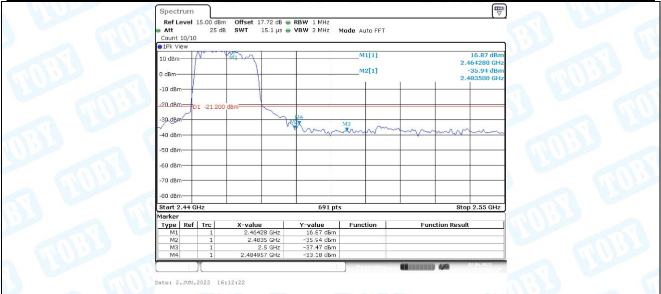
11AX20MIMO_Ant2_High_2462_Peak
