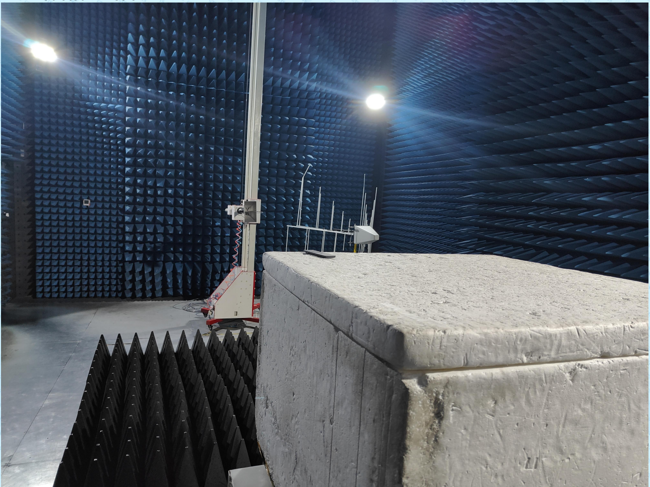
Radiated Emission
