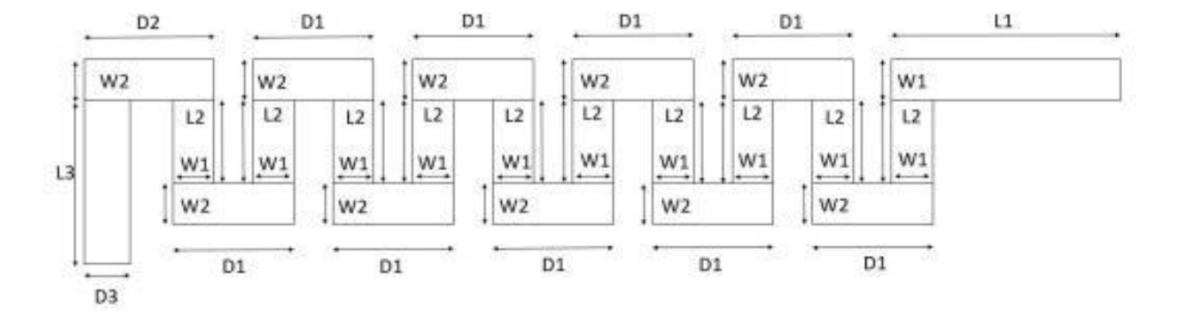
Antenna Dimensions
