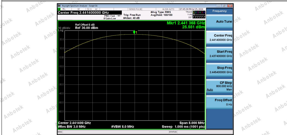
2.4G-Ant2-2441.4-PASS
