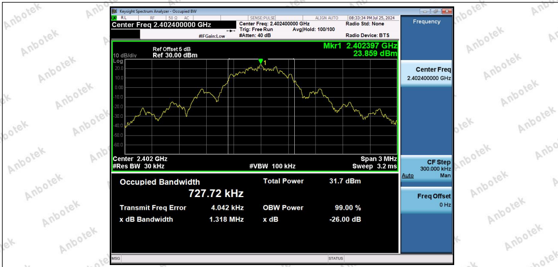
2.4G-Ant2-2402.4
