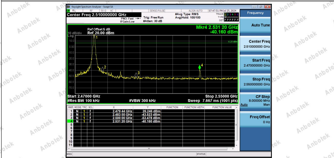
2.4G-Ant2-2479.4-PASS
