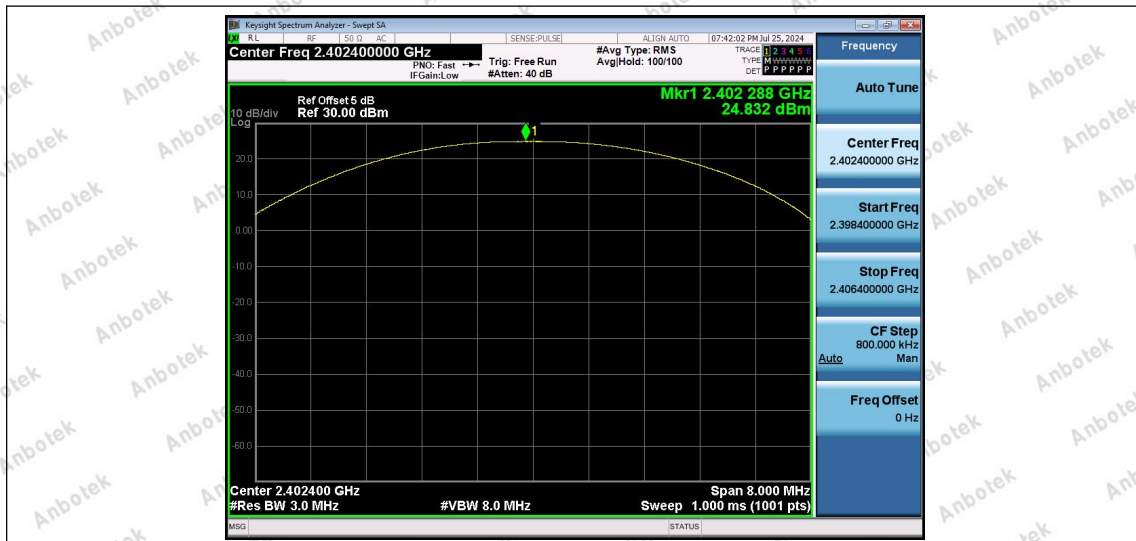
2.4G-Ant2-2402.4-PASS
