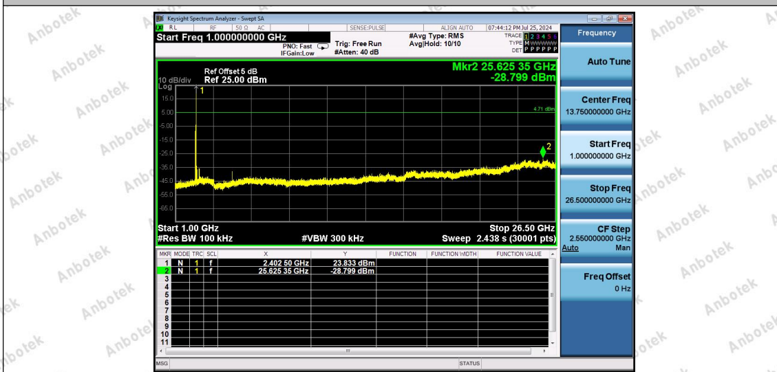
2.4G-Ant2-2402.4-1000~26500-PASS
