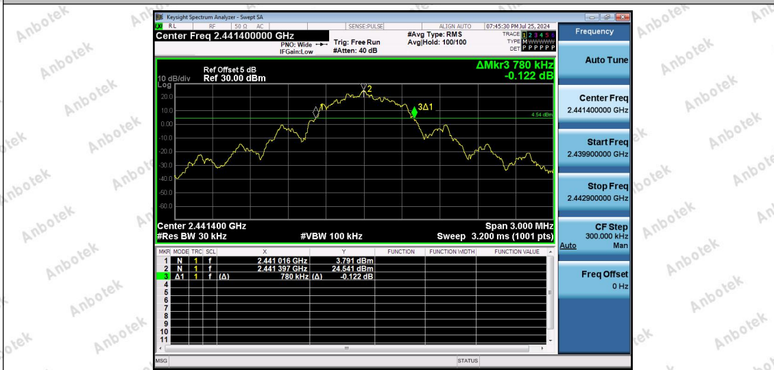
2.4G-Ant2-2441.4
