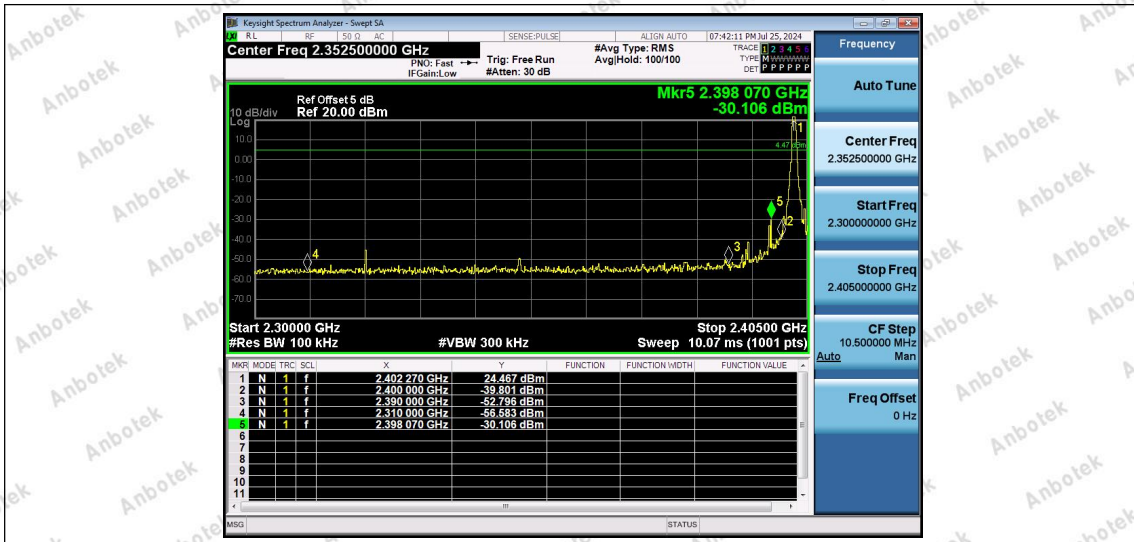
2.4G-Ant2-2402.4-PASS
