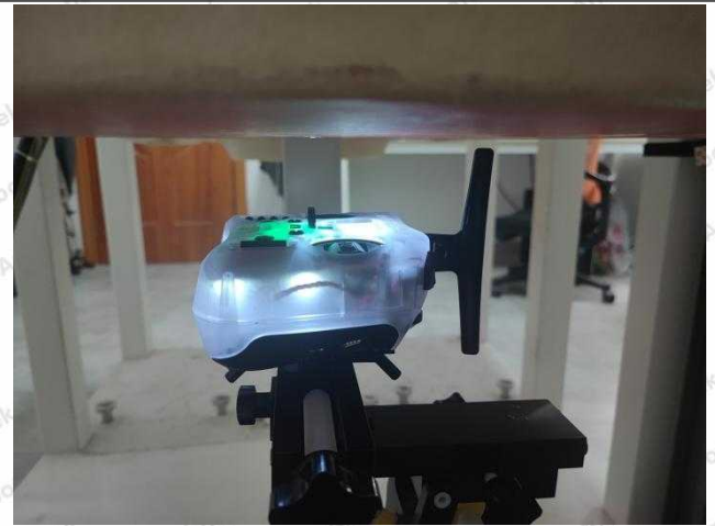
Body Back(10mm) Antenna Horizontal
