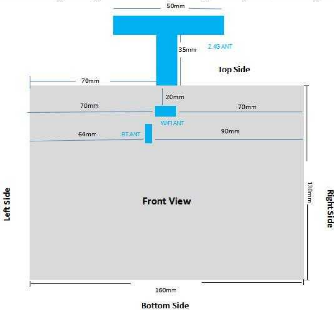
Distance of The Antenna vertical to the EUT surface and edge
