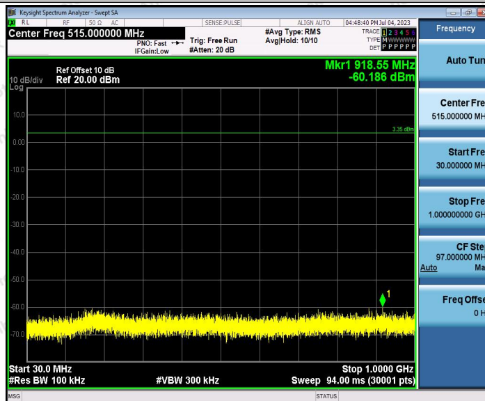
2.4G_Ant1_2441.4_30~1000
