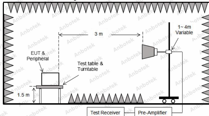
Figure 3. Above 1 GHz
