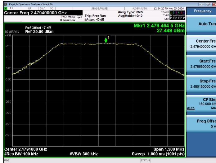
2.4G-Ant2-2479.4-0~Reference-PASS
