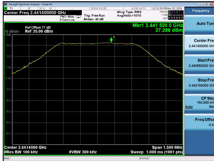
2.4G-Ant2-2441.4-0~Reference-PASS
