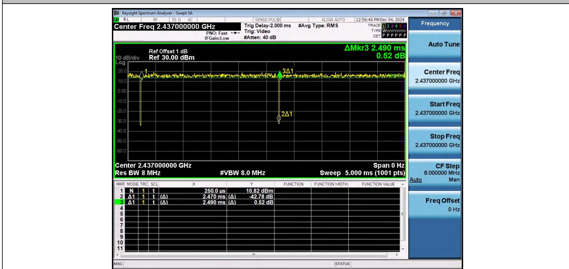
NTVN-11N40SISO-Ant1-2437
