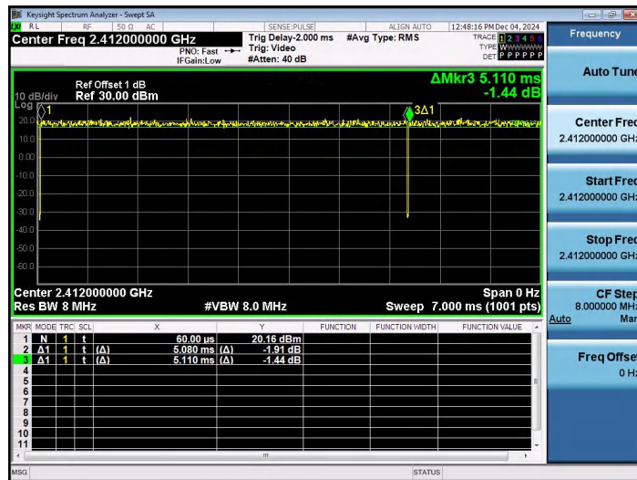
NTVN-11N20SISO-Ant1-2412
