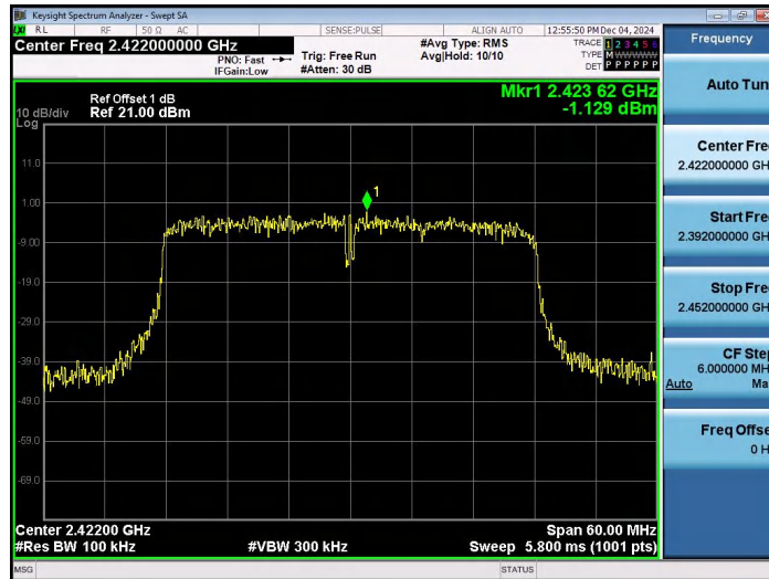
11N40SISO-Ant1-2422-0~Reference-PASS
