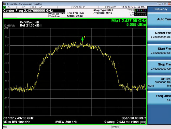
11B-Ant1-2437-0~Reference-PASS
