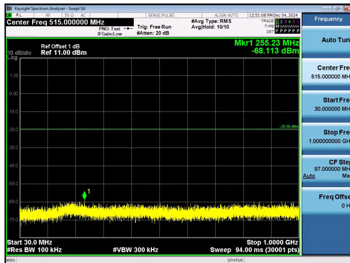
11N20SISO-Ant1-2437-30~1000-PASS
