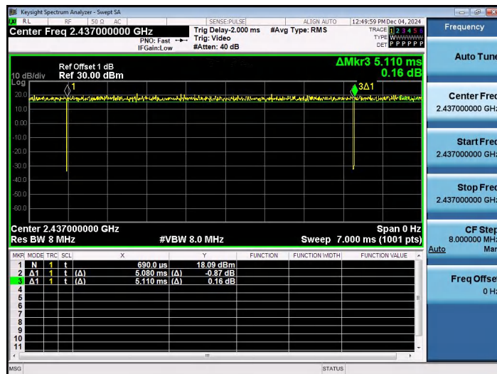
NTVN-11N20SISO-Ant1-2437
