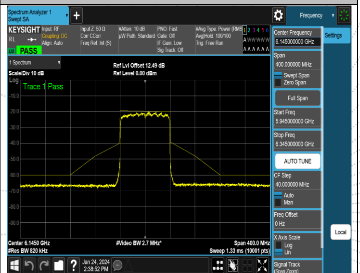
NTNV-11AX80MIMO-Ant4-6145-PASS
