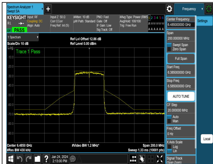
NTNV-11AX40MIMO-Ant3-6485-PASS
