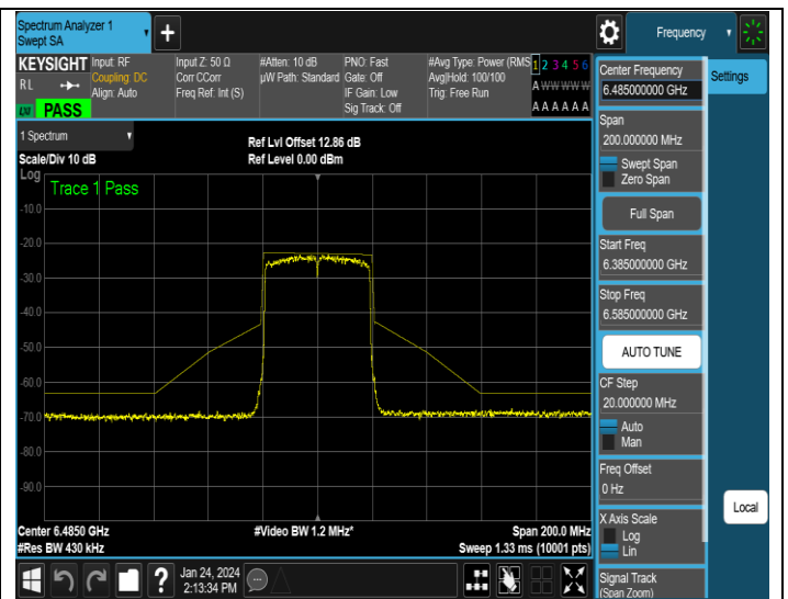
NTNV-11AX40MIMO-Ant4-6485-PASS
