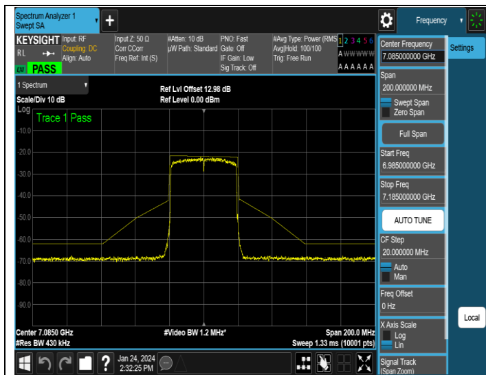
NTNV-11AX40MIMO-Ant1-7085-PASS
