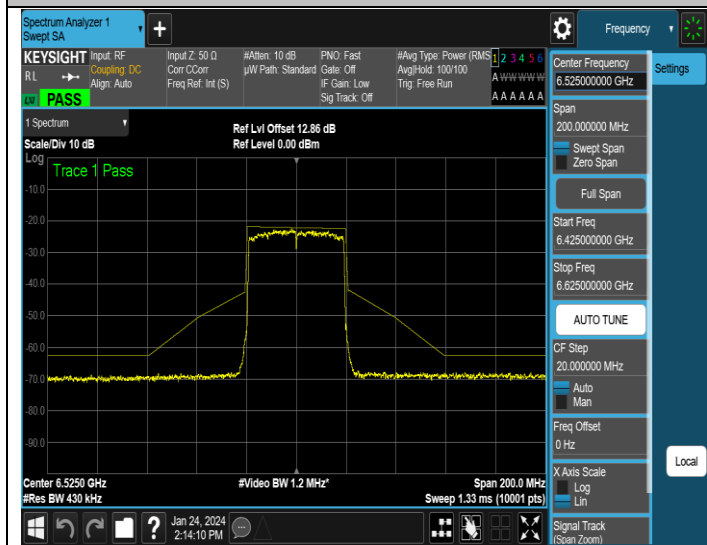
NTNV-11AX40MIMO-Ant1-6525-PASS
