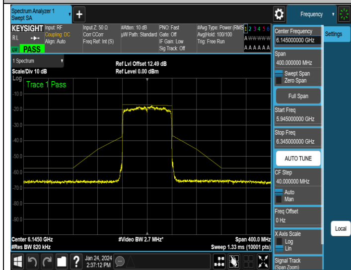
NTNV-11AX80MIMO-Ant1-6145-PASS
