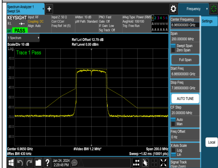
NTNV-11AX40MIMO-Ant1-6965-PASS
