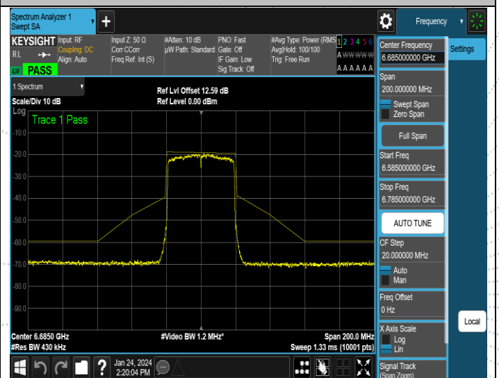
NTNV-11AX40MIMO-Ant2-6685-PASS
