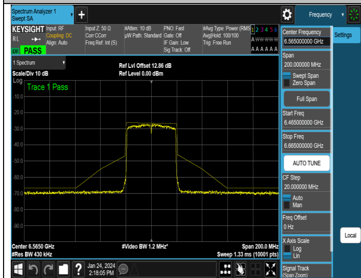
NTNV-11AX40MIMO-Ant3-6565-PASS
