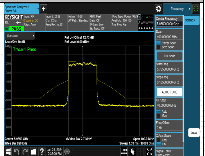
NTNV-11AX80MIMO-Ant2-5985-PASS
