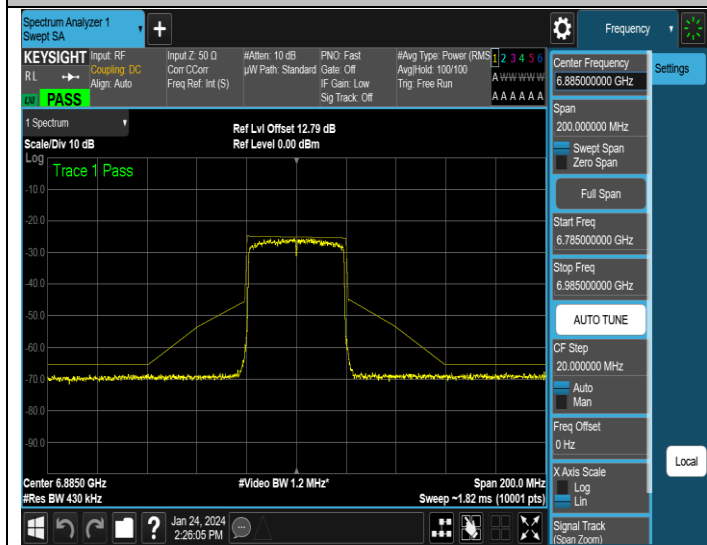
NTNV-11AX40MIMO-Ant3-6885-PASS
