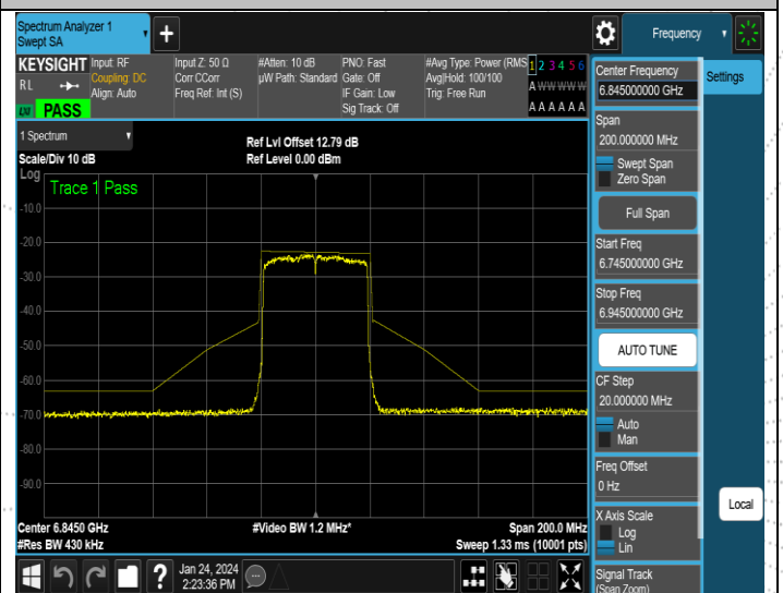
NTNV-11AX40MIMO-Ant4-6845-PASS
