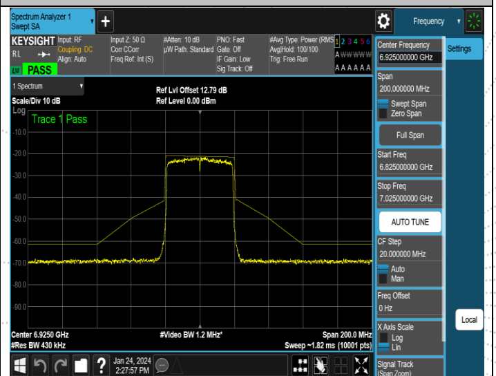
NTNV-11AX40MIMO-Ant2-6925-PASS
