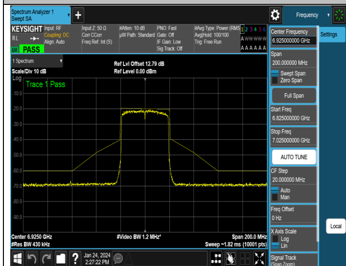
NTNV-11AX40MIMO-Ant1-6925-PASS
