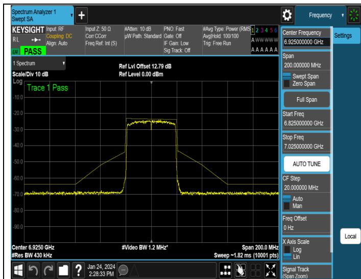
NTNV-11AX40MIMO-Ant3-6925-PASS
