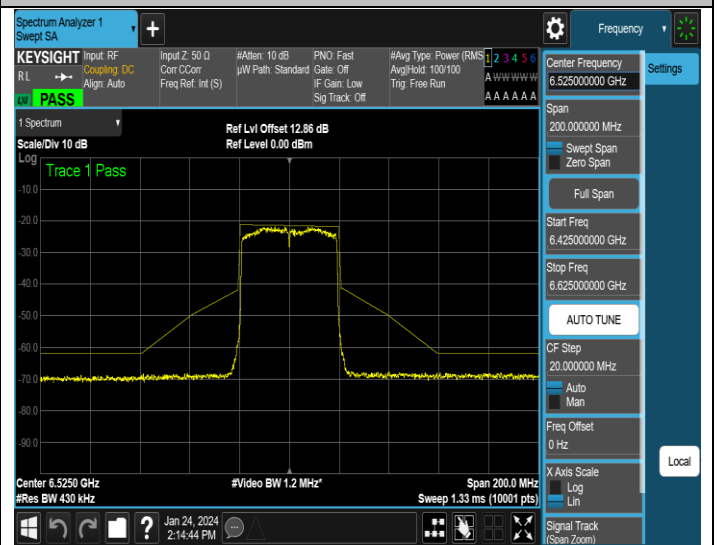
NTNV-11AX40MIMO-Ant2-6525-PASS
