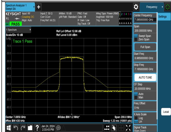
NTNV-11AX40MIMO-Ant3-7085-PASS
