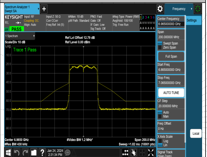
NTNV-11AX40MIMO-Ant4-6965-PASS
