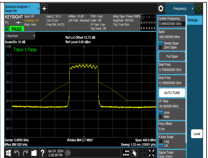
NTNV-11AX80MIMO-Ant4-5985-PASS
