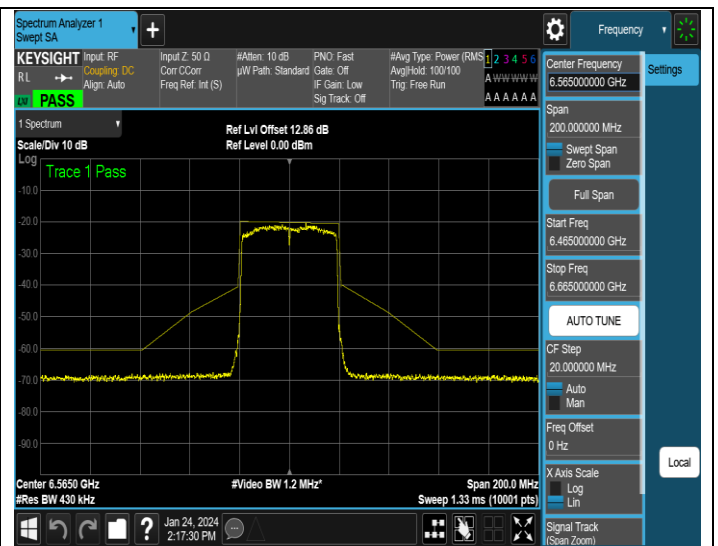
NTNV-11AX40MIMO-Ant2-6565-PASS
