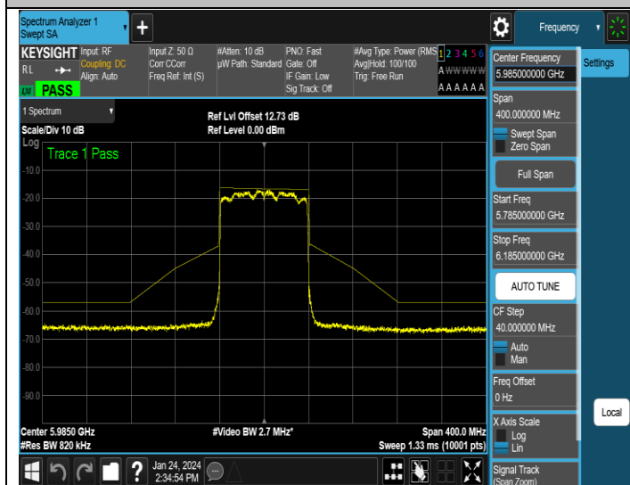
NTNV-11AX80MIMO-Ant1-5985-PASS
