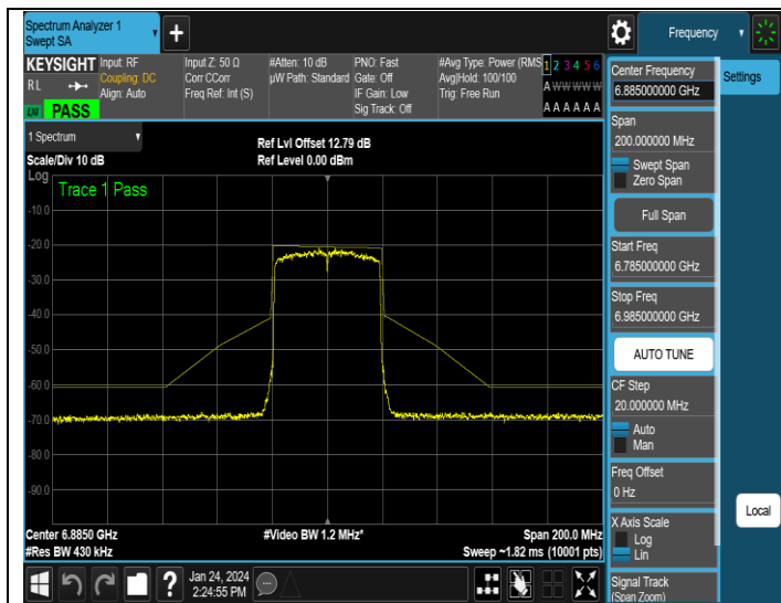
NTNV-11AX40MIMO-Ant1-6885-PASS
