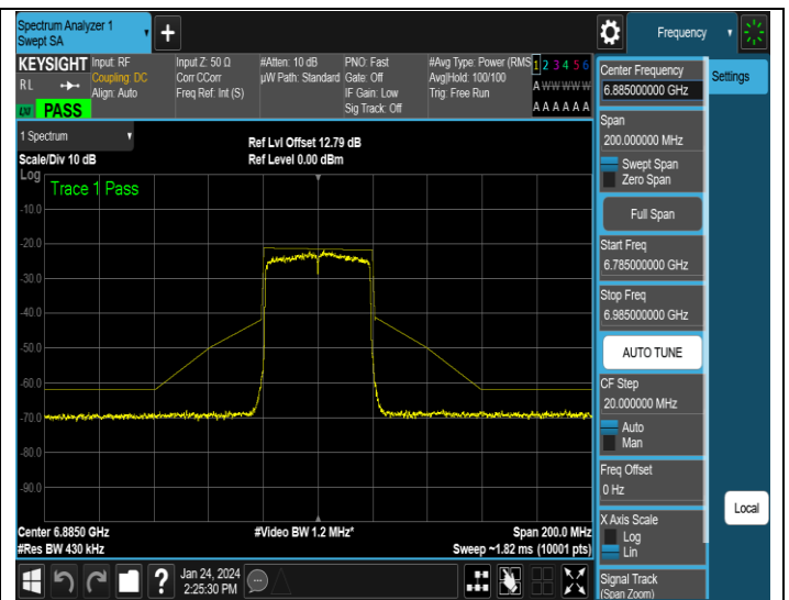
NTNV-11AX40MIMO-Ant2-6885-PASS
