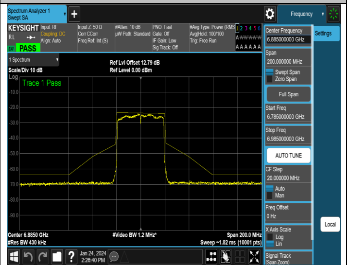
NTNV-11AX40MIMO-Ant4-6885-PASS
