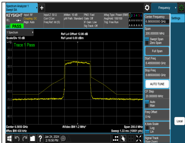
NTNV-11AX40MIMO-Ant1-6565-PASS
