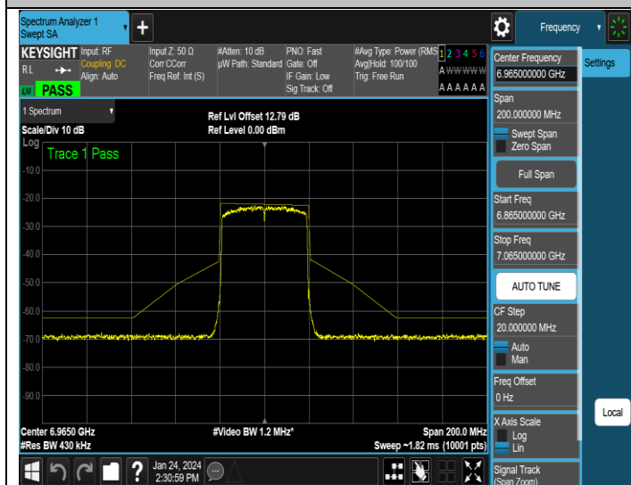
NTNV-11AX40MIMO-Ant3-6965-PASS
