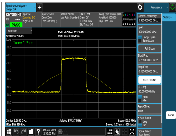
NTNV-11AX80MIMO-Ant3-5985-PASS
