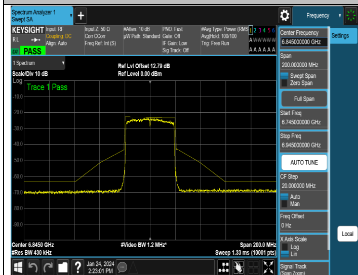
NTNV-11AX40MIMO-Ant3-6845-PASS
