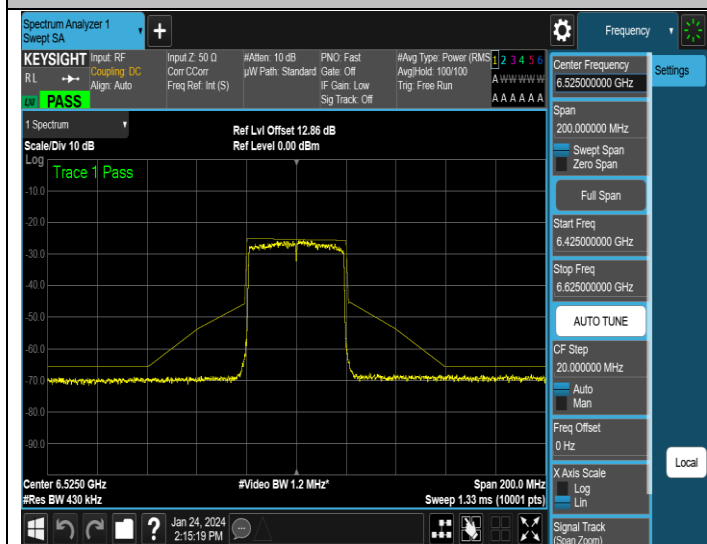
NTNV-11AX40MIMO-Ant3-6525-PASS
