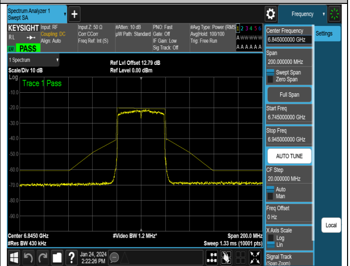
NTNV-11AX40MIMO-Ant2-6845-PASS
