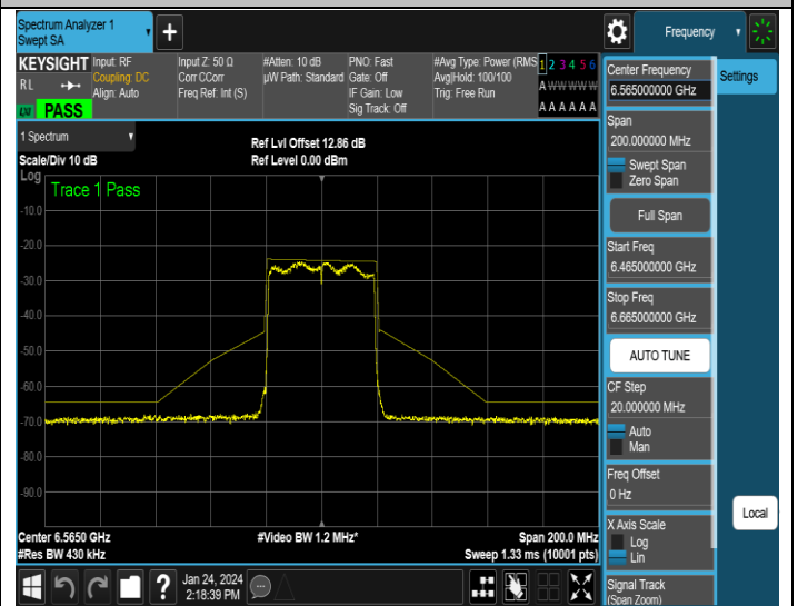
NTNV-11AX40MIMO-Ant4-6565-PASS
