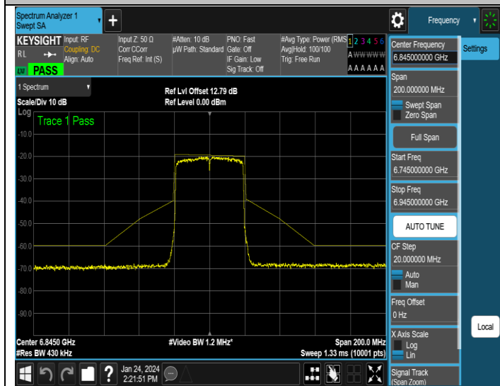
NTNV-11AX40MIMO-Ant1-6845-PASS
