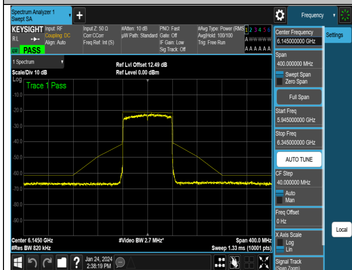
NTNV-11AX80MIMO-Ant3-6145-PASS
