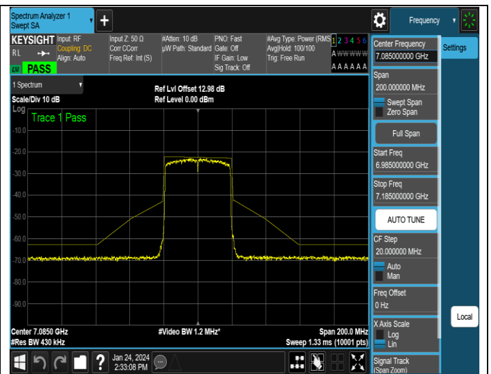
NTNV-11AX40MIMO-Ant2-7085-PASS
