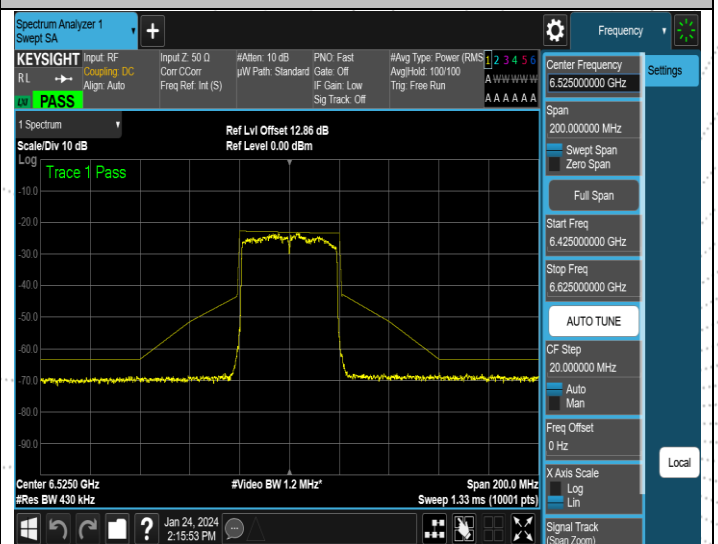
NTNV-11AX40MIMO-Ant4-6525-PASS
