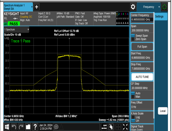
NTNV-11AX40MIMO-Ant2-6965-PASS
