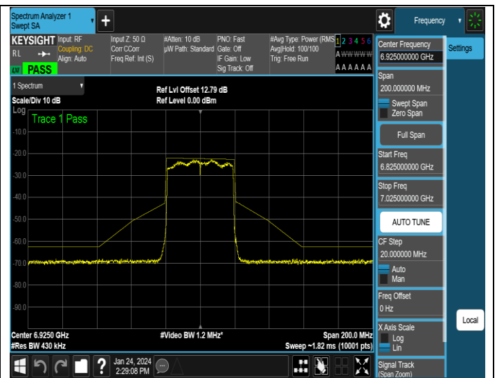
NTNV-11AX40MIMO-Ant4-6925-PASS
