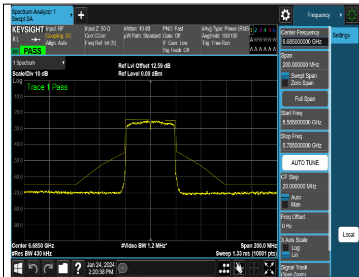
NTNV-11AX40MIMO-Ant3-6685-PASS
