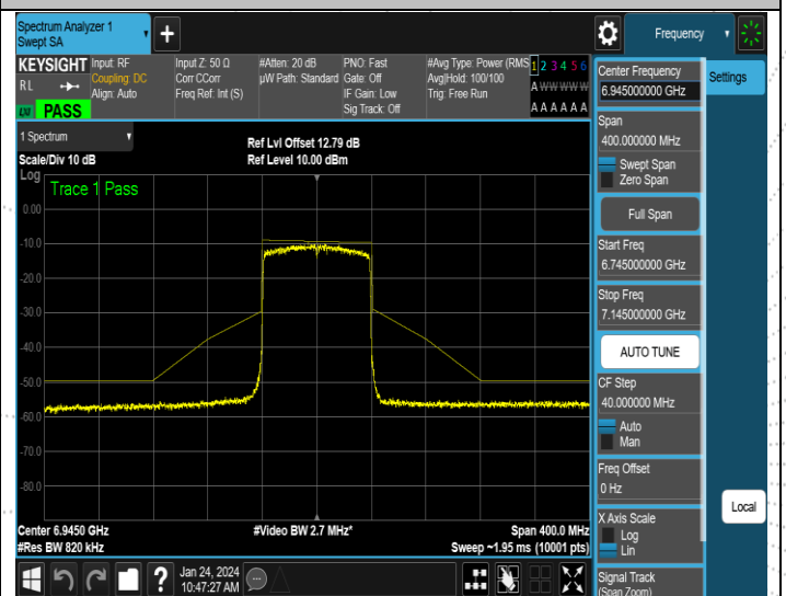
NTNV-11AX80ISO-Ant4-6945-PASS
