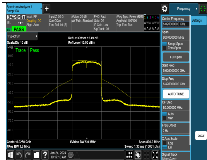
NTNV-11AX160SISO-Ant3-6025-PASS
