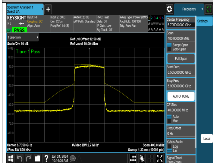
NTNV-11AX80ISO-Ant3-6705-PASS
