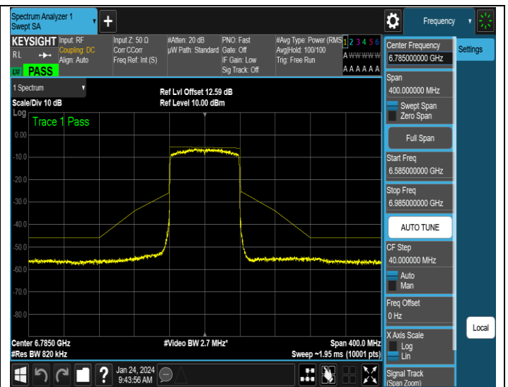
NTNV-11AX80ISO-Ant2-6785-PASS
