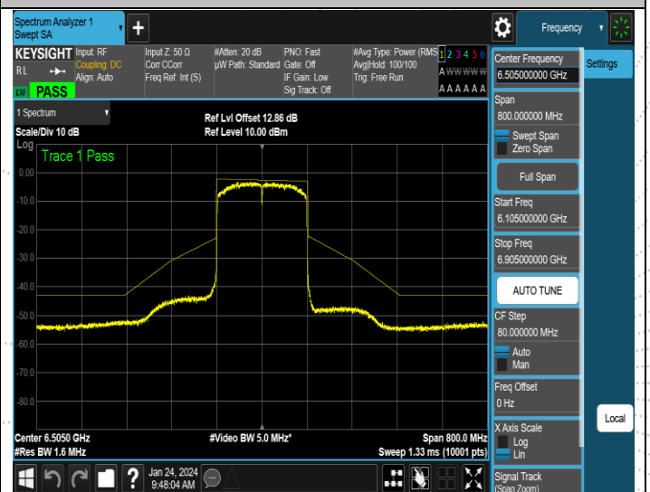
NTNV-11AX160SISO-Ant2-6505-PASS
