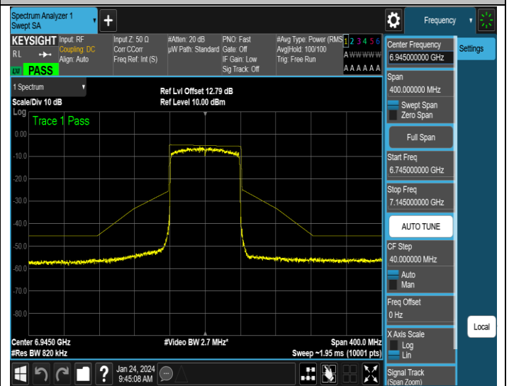
NTNV-11AX80ISO-Ant2-6945-PASS
