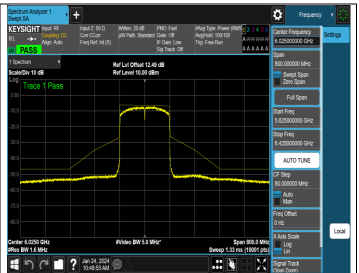
NTNV-11AX160SISO-Ant4-6025-PASS
