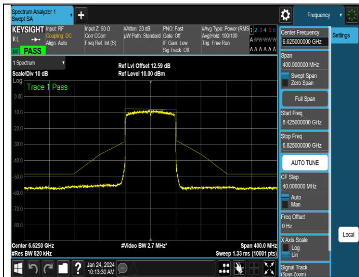
NTNV-11AX80ISO-Ant3-6625-PASS
