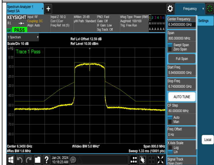
NTNV-11AX160SISO-Ant3-6345-PASS
