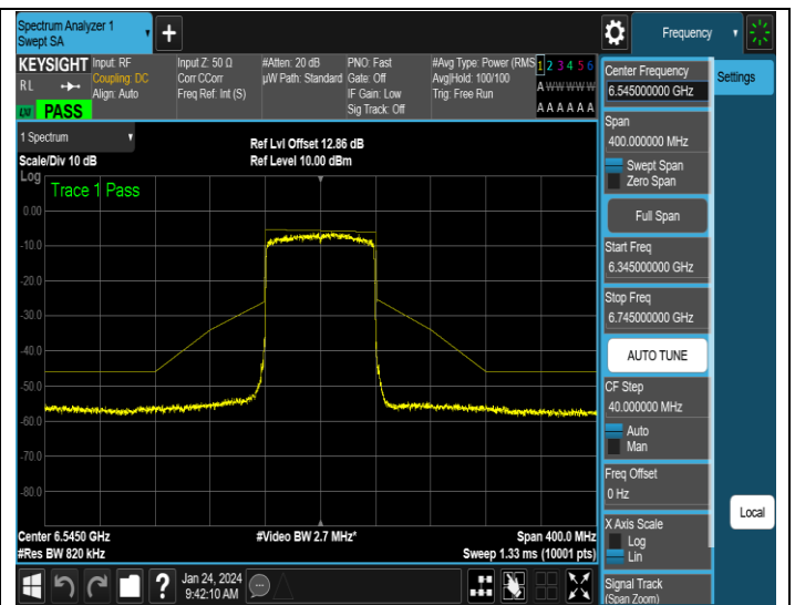
NTNV-11AX80ISO-Ant2-6545-PASS
