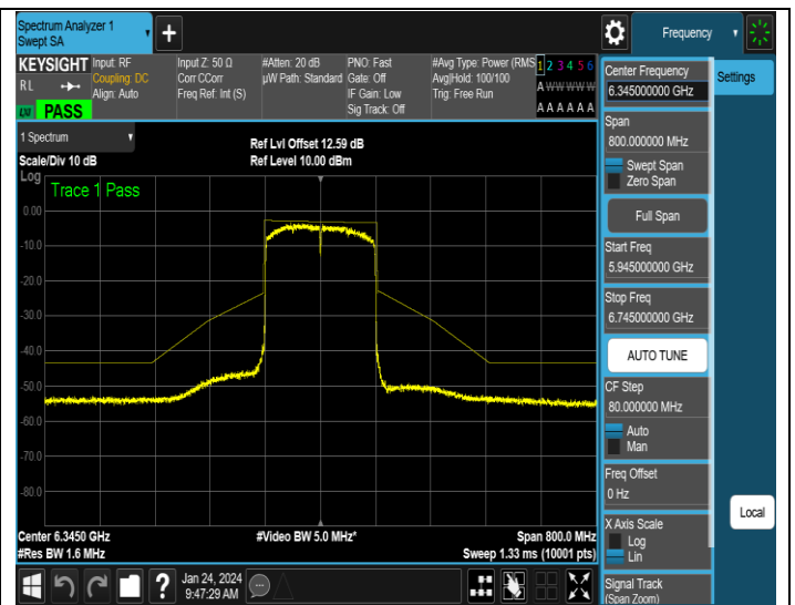
NTNV-11AX160SISO-Ant2-6345-PASS
