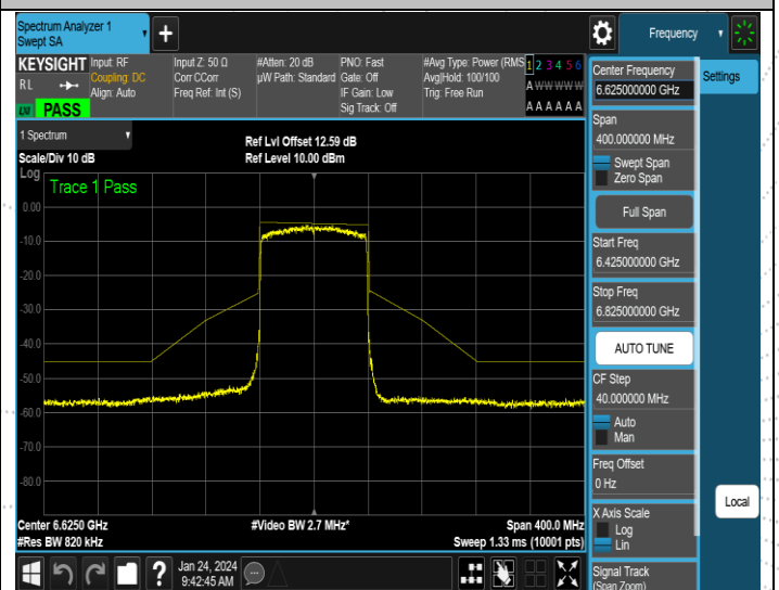
NTNV-11AX80ISO-Ant2-6625-PASS
