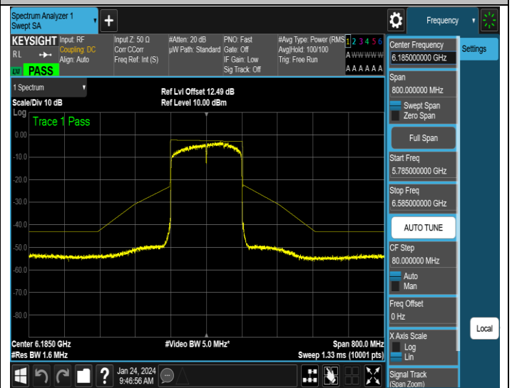
NTNV-11AX160SISO-Ant2-6185-PASS
