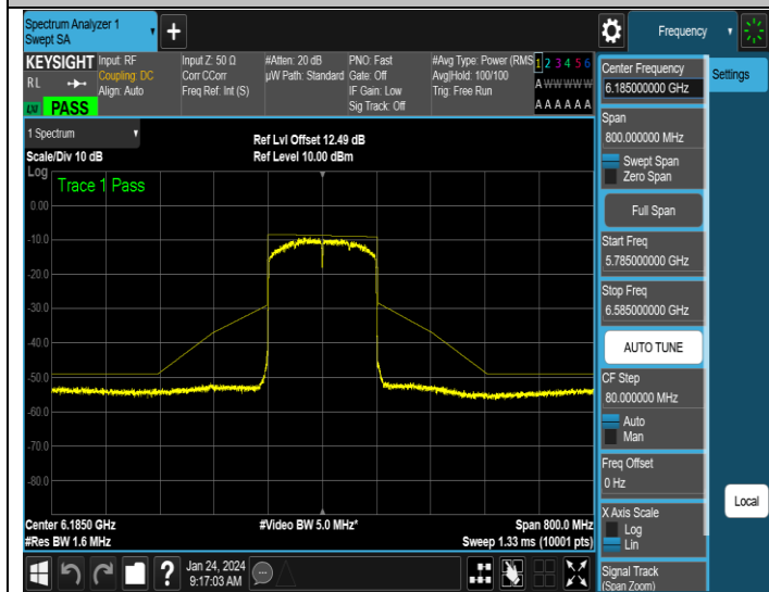
NTNV-11AX160SISO-Ant1-6185-PASS
