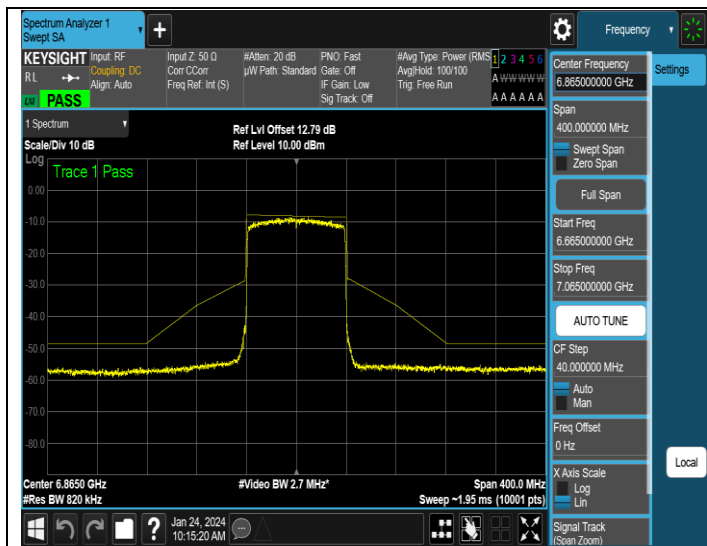
NTNV-11AX80ISO-Ant3-6865-PASS
