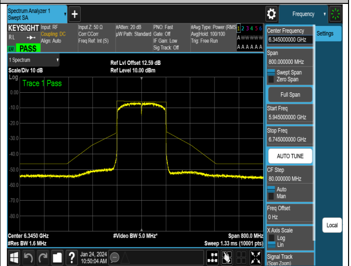
NTNV-11AX160SISO-Ant4-6345-PASS
