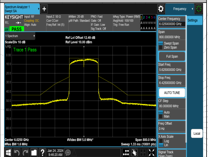
NTNV-11AX160SISO-Ant2-6025-PASS
