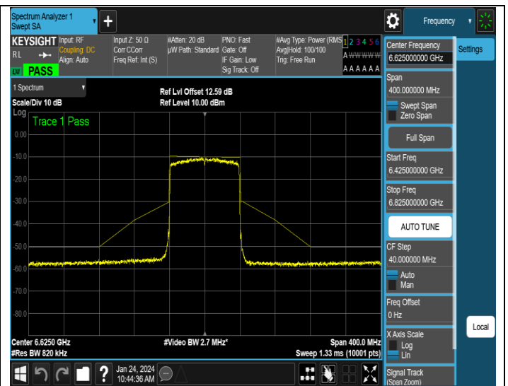
NTNV-11AX80ISO-Ant4-6625-PASS
