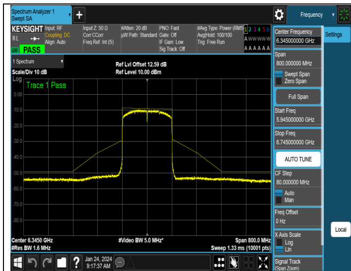
NTNV-11AX160SISO-Ant1-6345-PASS
