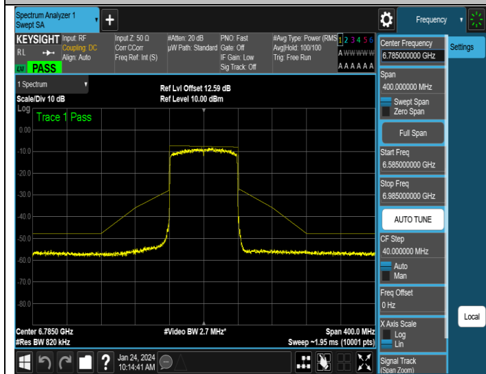
NTNV-11AX80ISO-Ant3-6785-PASS
