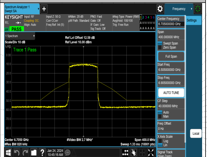
NTNV-11AX80ISO-Ant4-6705-PASS
