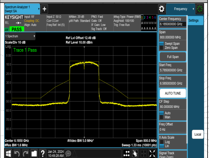
NTNV-11AX160SISO-Ant4-6185-PASS
