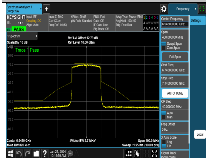
NTNV-11AX80ISO-Ant3-6945-PASS
