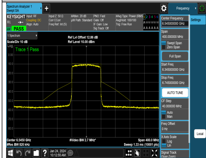
NTNV-11AX80ISO-Ant3-6545-PASS
