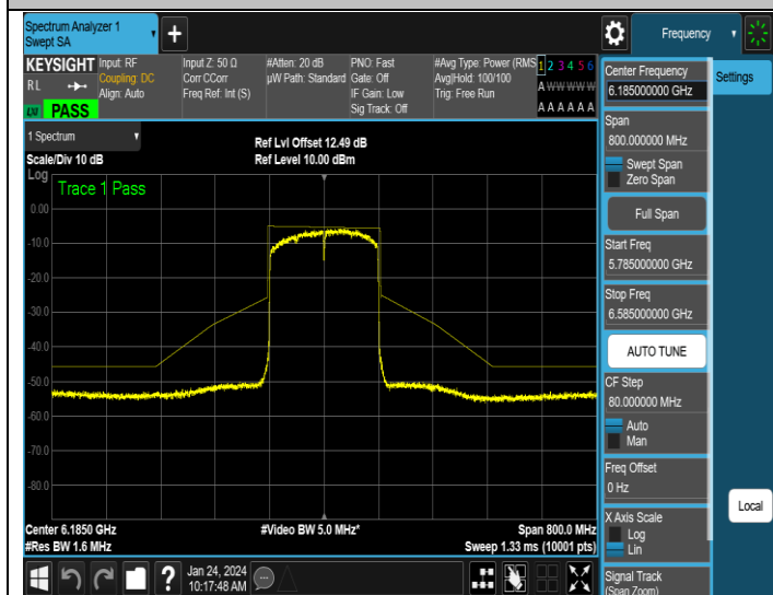
NTNV-11AX160SISO-Ant3-6185-PASS
