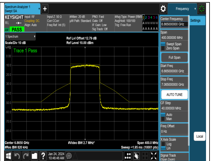
NTNV-11AX80ISO-Ant4-6865-PASS
