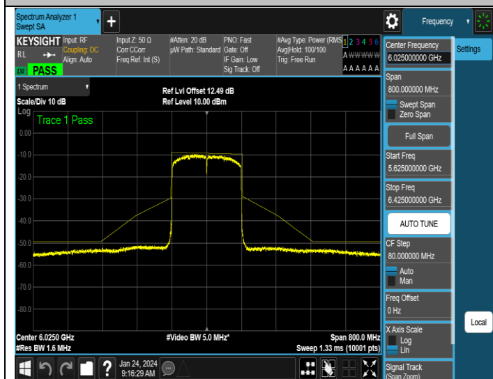
NTNV-11AX160SISO-Ant1-6025-PASS
