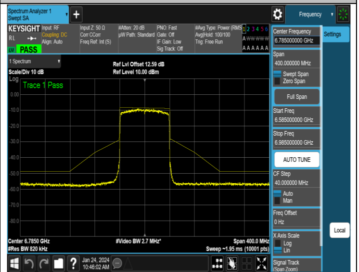
NTNV-11AX80ISO-Ant4-6785-PASS
