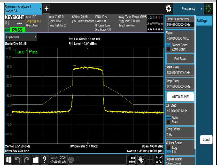
NTNV-11AX80ISO-Ant4-6545-PASS
