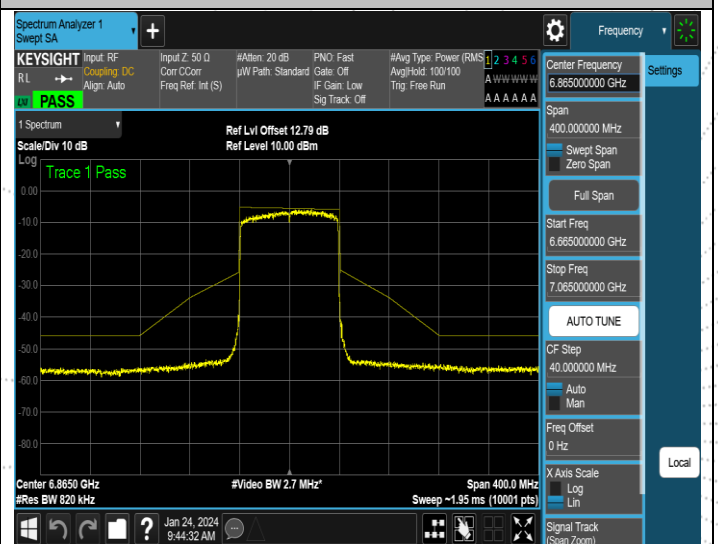
NTNV-11AX80ISO-Ant2-6865-PASS
