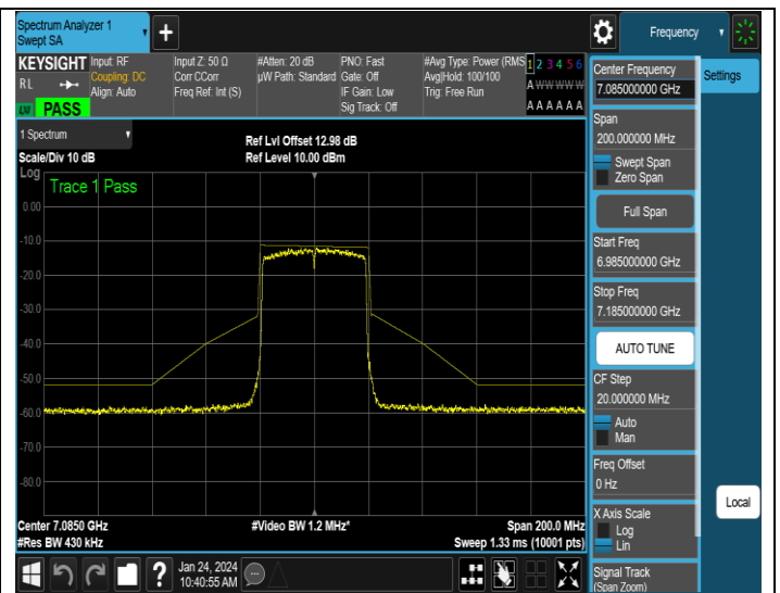
NTNV-11AX40SISO-Ant4-7085-PASS
