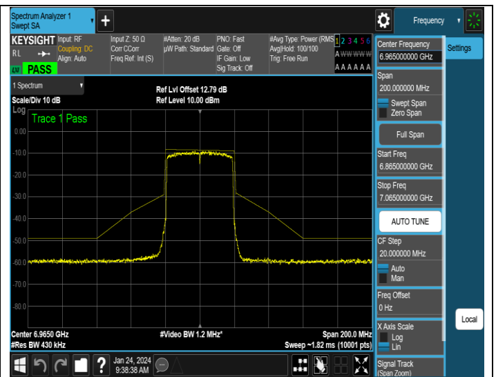
NTNV-11AX40ISO-Ant2-6965-PASS
