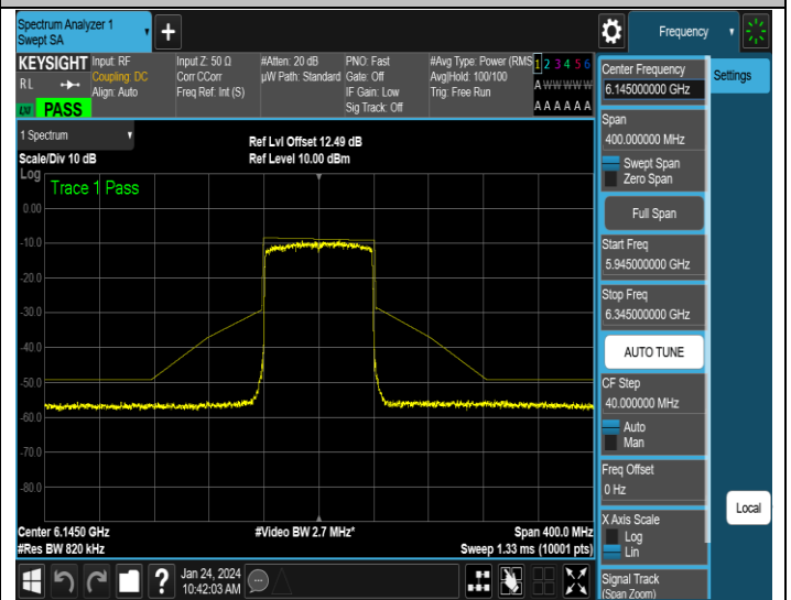
NTNV-11AX80ISO-Ant4-6145-PASS
