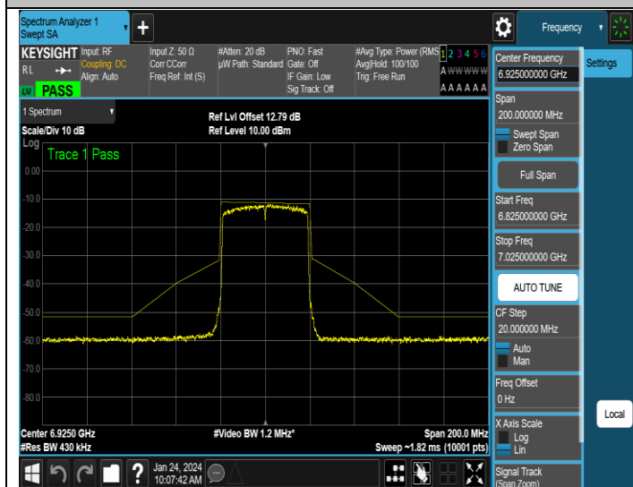
NTNV-11AX40ISO-Ant3-6925-PASS
