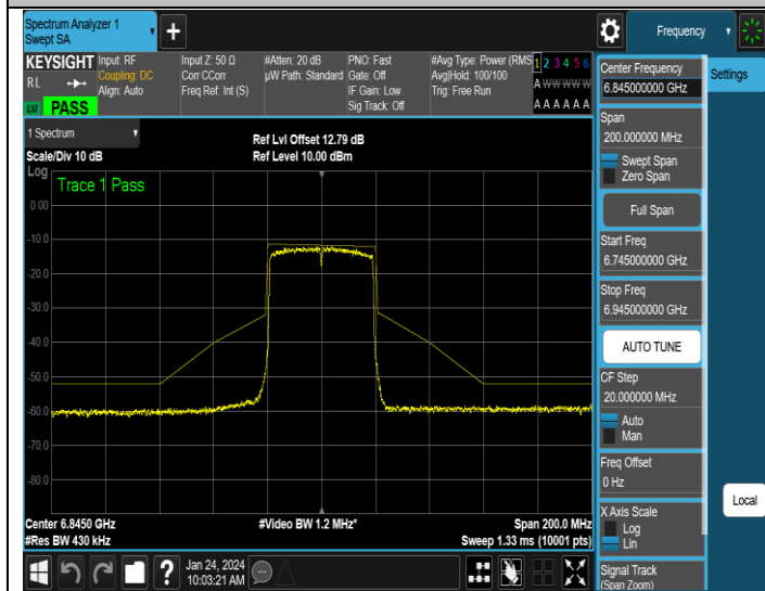
NTNV-11AX40SISO-Ant3-6845-PASS
