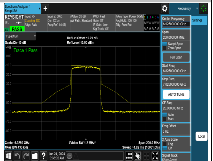
NTNV-11AX40ISO-Ant2-6925-PASS
