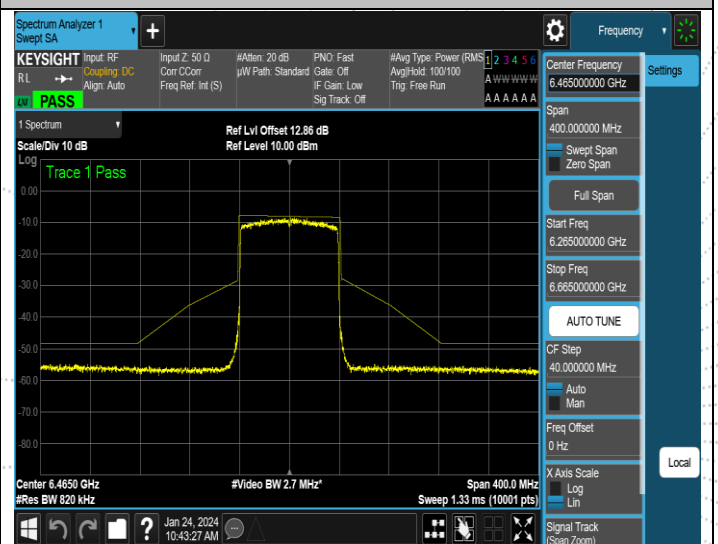
NTNV-11AX80ISO-Ant4-6465-PASS
