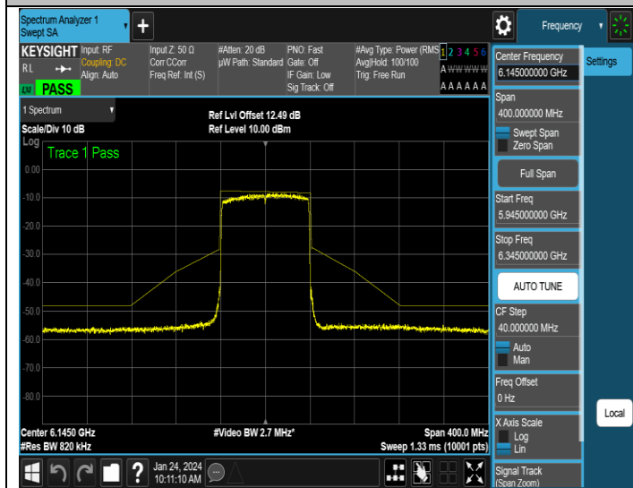
NTNV-11AX80ISO-Ant3-6145-PASS
