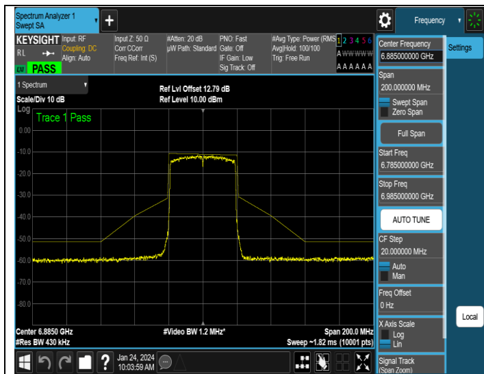
NTNV-11AX40ISO-Ant3-6885-PASS
