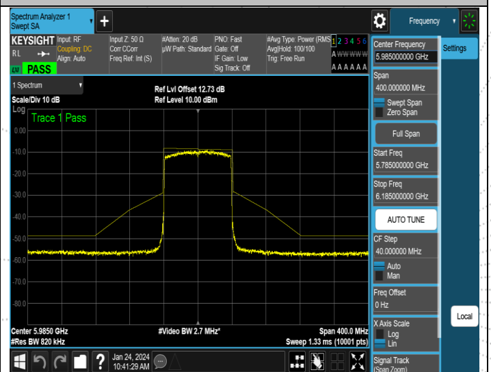
NTNV-11AX80SISO-Ant4-5985-PASS
