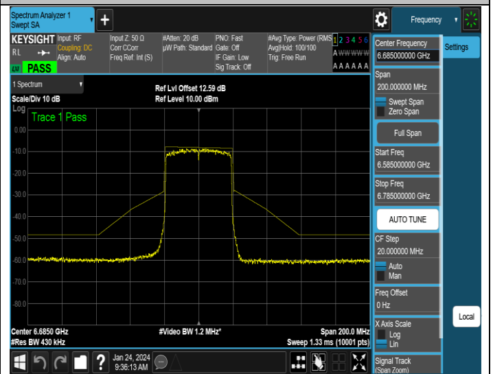
NTNV-11AX40ISO-Ant2-6685-PASS
