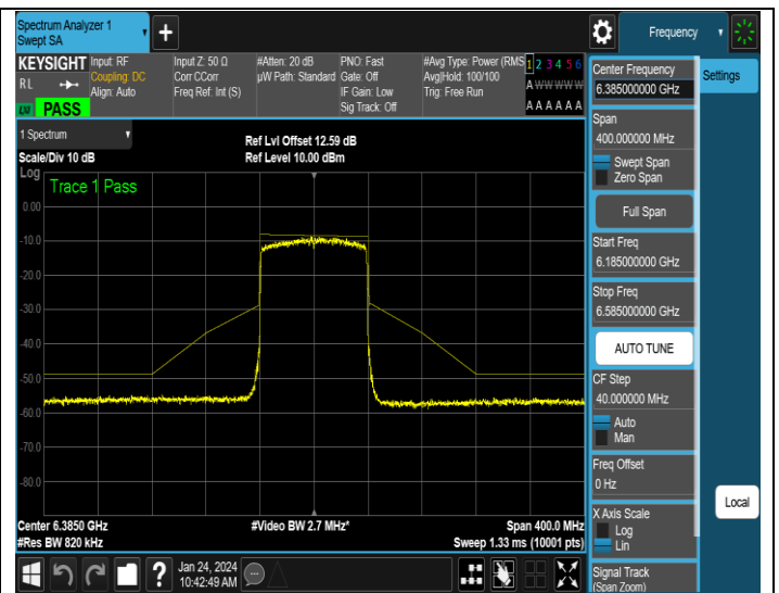
NTNV-11AX80ISO-Ant4-6385-PASS
