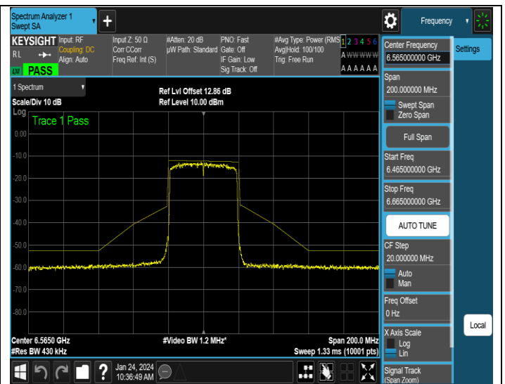
NTNV-11AX40ISO-Ant4-6565-PASS
