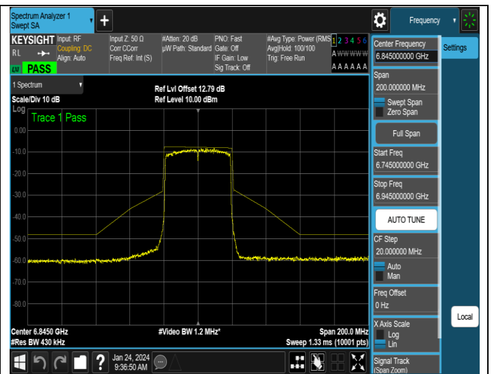
NTNV-11AX40SISO-Ant2-6845-PASS
