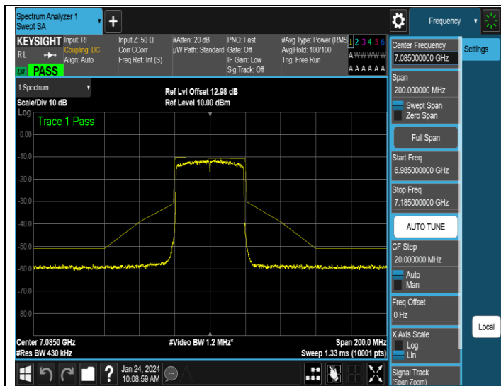
NTNV-11AX40SISO-Ant3-7085-PASS
