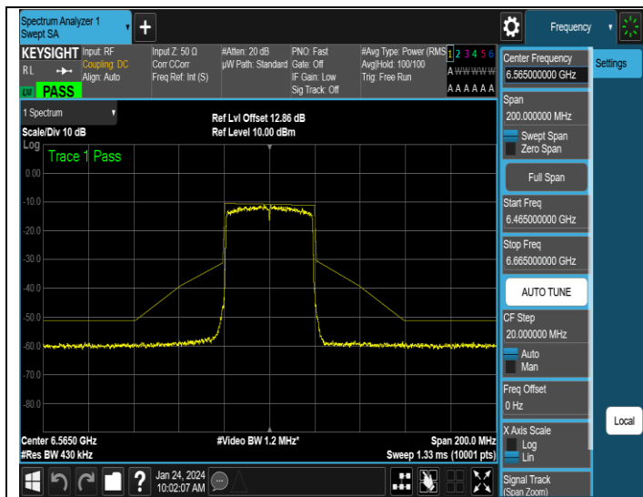
NTNV-11AX40ISO-Ant3-6565-PASS
