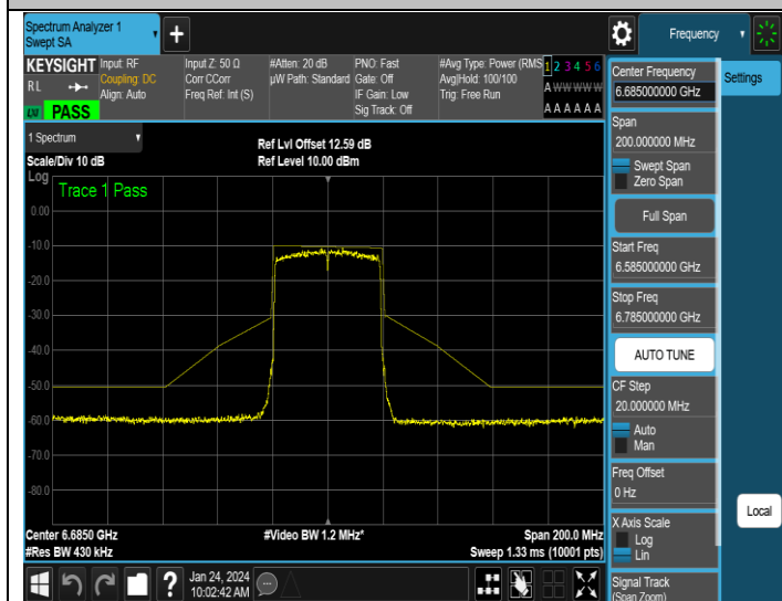
NTNV-11AX40ISO-Ant3-6685-PASS
