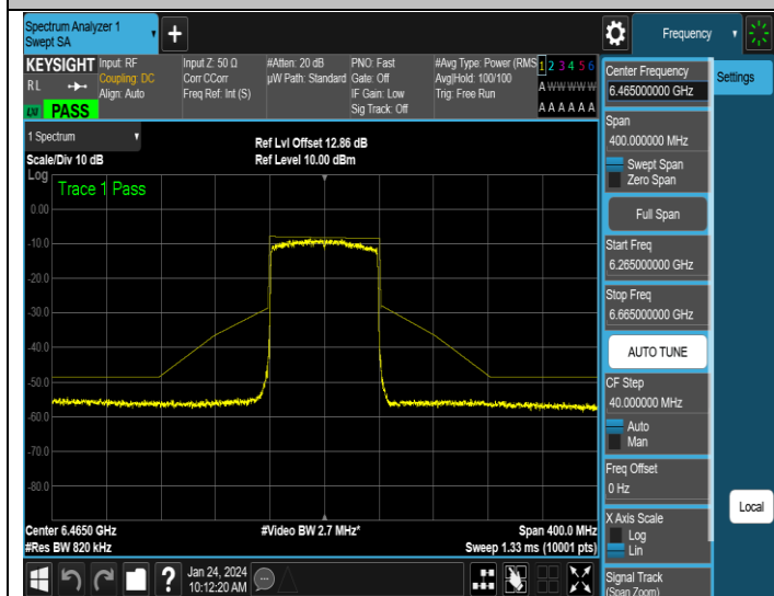
NTNV-11AX80ISO-Ant3-6465-PASS
