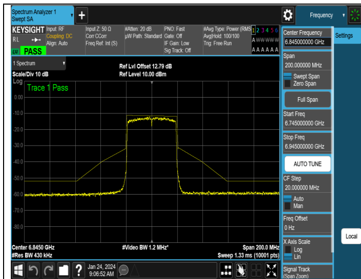
NTNV-11AX40SISO-Ant1-6845-PASS
