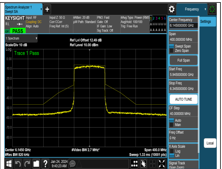
NTNV-11AX80ISO-Ant2-6145-PASS
