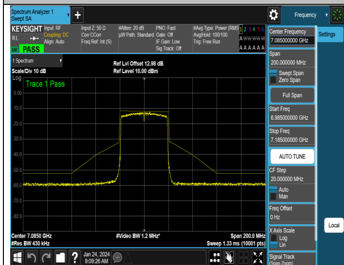
NTNV-11AX40ISO-Ant1-7085-PASS
