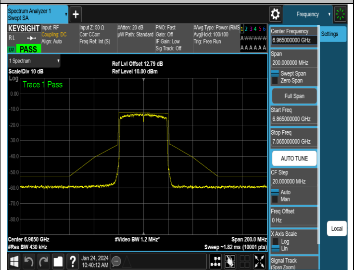
NTNV-11AX40ISO-Ant4-6965-PASS
