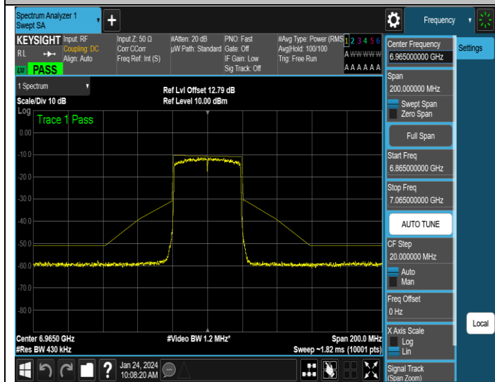
NTNV-11AX40ISO-Ant3-6965-PASS
