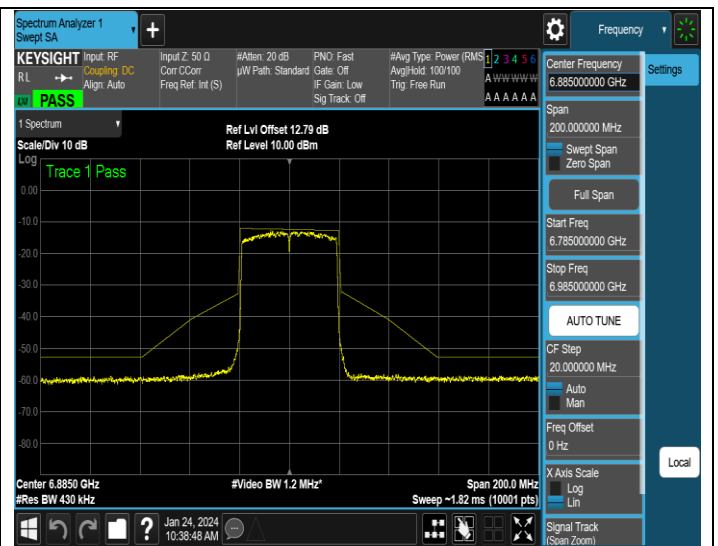
NTNV-11AX40ISO-Ant4-6885-PASS
