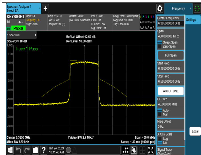
NTNV-11AX80ISO-Ant3-6385-PASS
