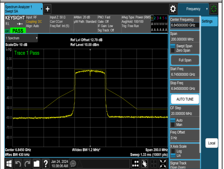
NTNV-11AX40SISO-Ant4-6845-PASS
