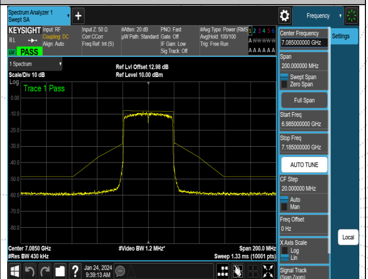
NTNV-11AX40ISO-Ant2-7085-PASS
