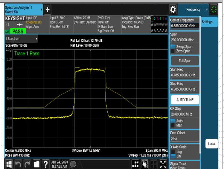
NTNV-11AX40SISO-Ant2-6885-PASS
