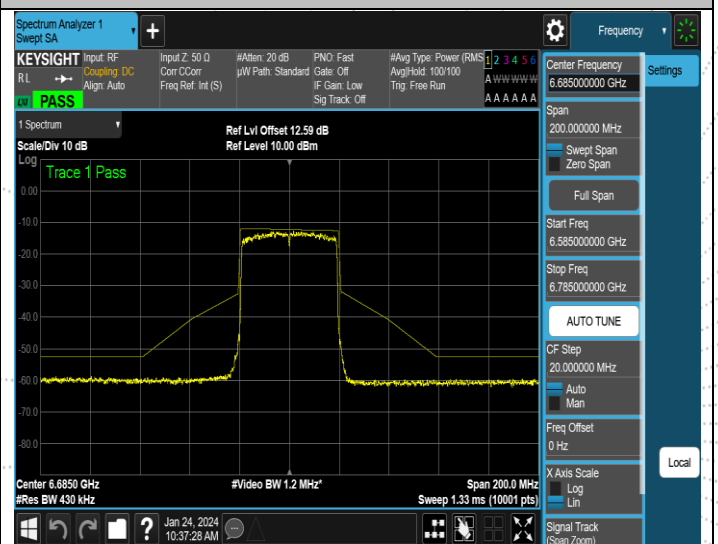
NTNV-11AX40ISO-Ant4-6685-PASS
