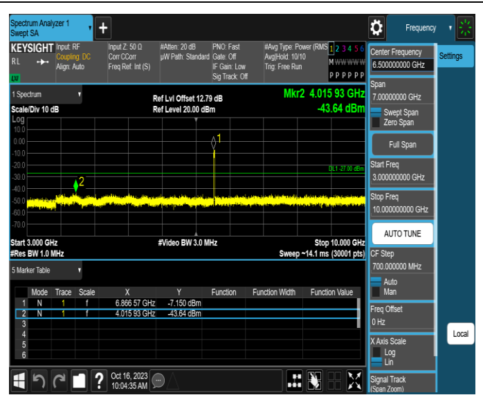
11AX20MIMO-Ant1-6875-3000~10000-PASS
