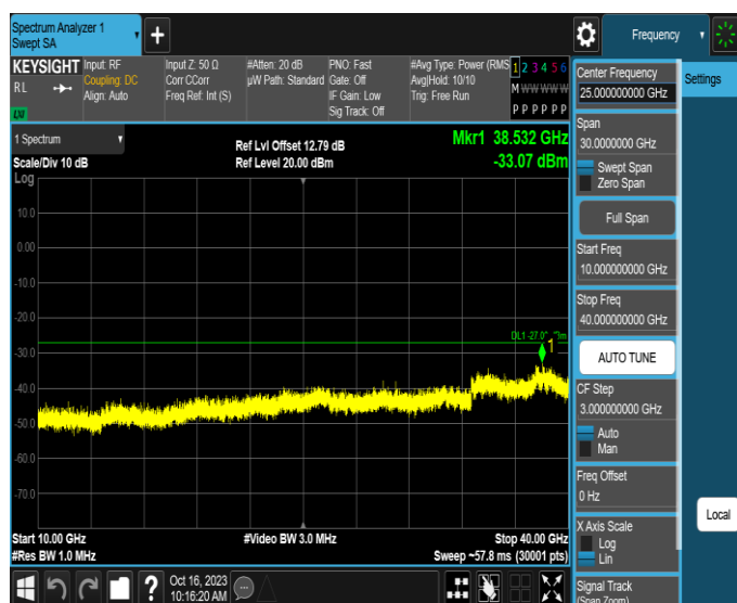
11AX20MIMO-Ant3-6875-10000~40000-PASS
