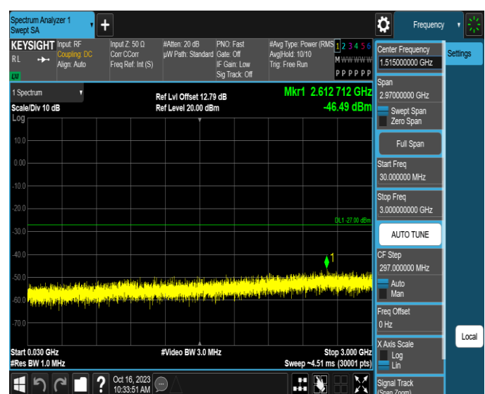
11AX20MIMO-Ant2-6895-30~3000-PASS
