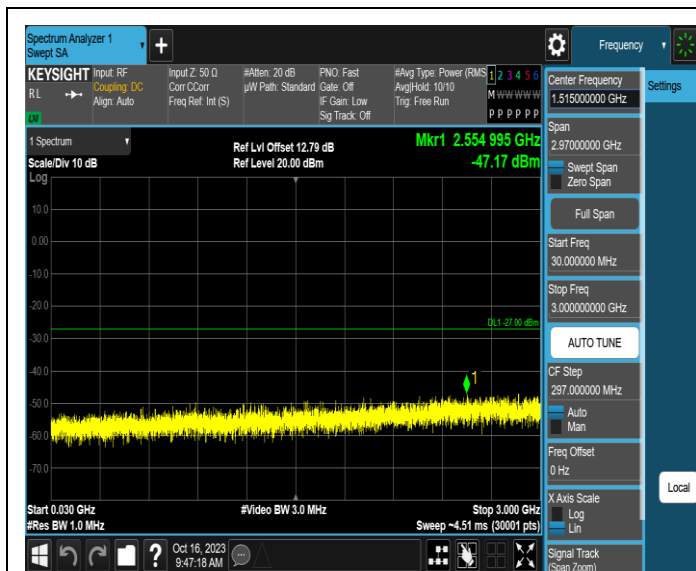
11AX20MIMO-Ant3-6855-30~3000-PASS
