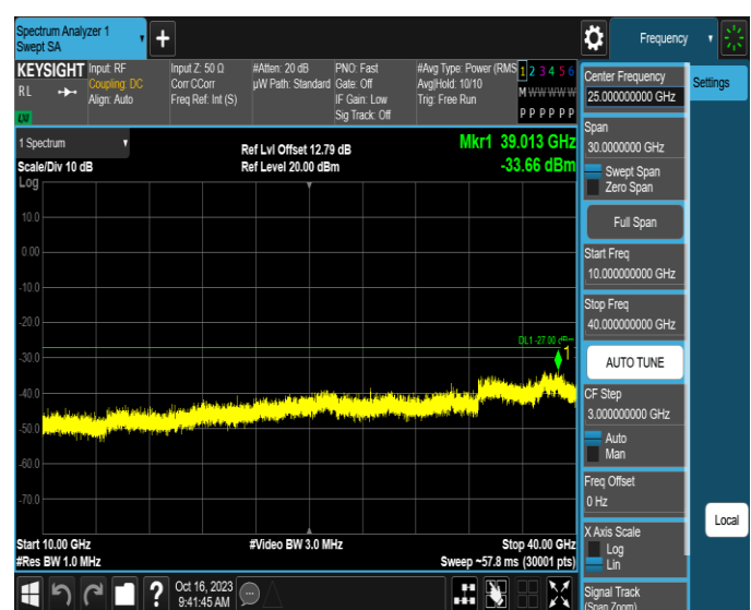
11AX20MIMO-Ant2-6855-10000~40000-PASS
