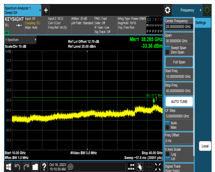
11AX20MIMO-Ant2-6875-10000~40000-PASS
