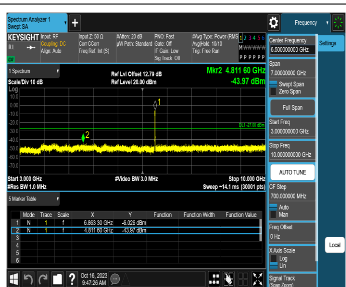
11AX20MIMO-Ant3-6855-3000~10000-PASS
