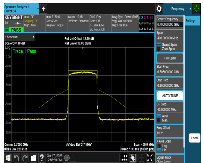
NTNV-11AX80MIMO-Ant4-6705-PASS
