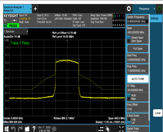
NTNV-11AX80MIMO-Ant4-6865-PASS
