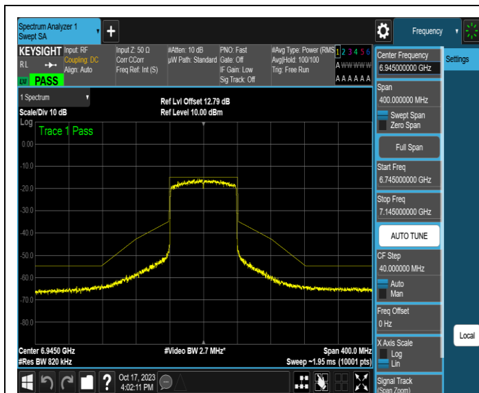
NTNV-11AX80MIMO-Ant1-6945-PASS
