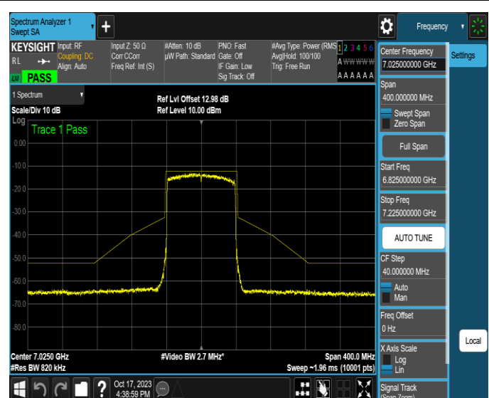
NTNV-11AX80MIMO-Ant2-7025-PASS
