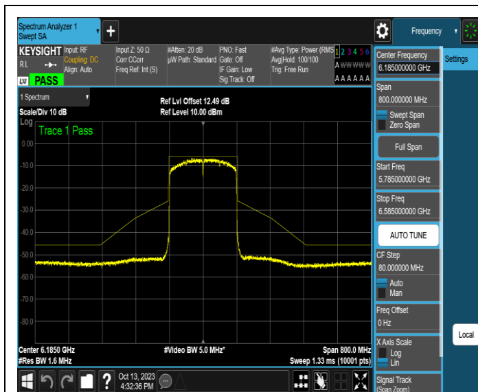
NTNV-11AX160SISO-Ant1-6185-PASS
