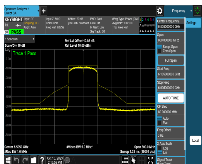
NTNV-11AX160SISO-Ant4-6505-PASS
