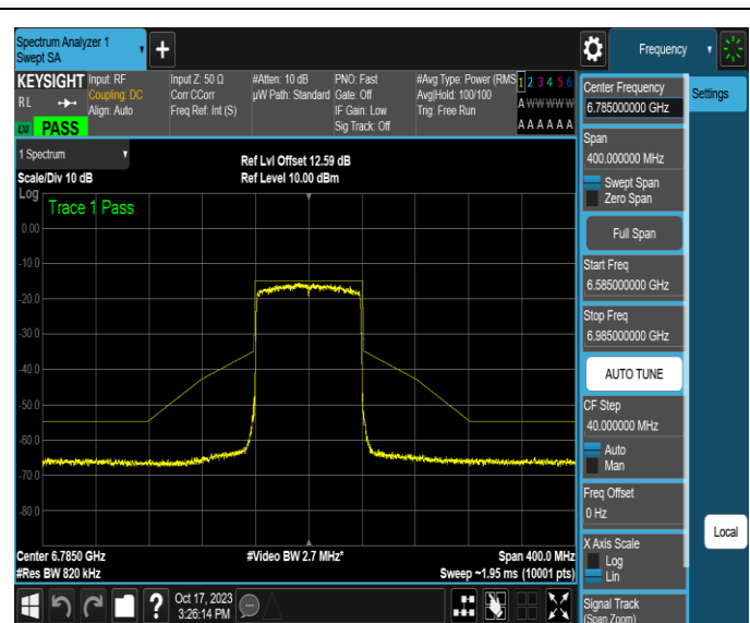
NTNV-11AX80MIMO-Ant4-6785-PASS
