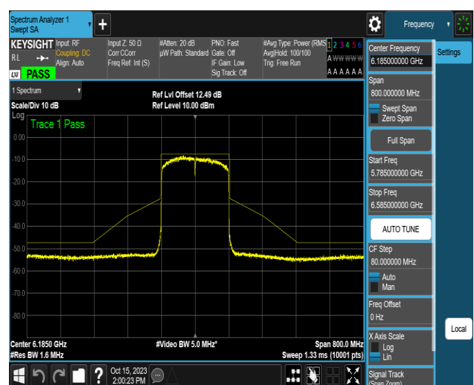
NTNV-11AX160SISO-Ant4-6185-PASS
