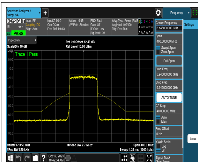
NTNV-11AX80MIMO-Ant3-6145-PASS
