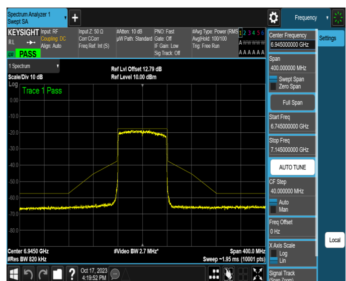
NTNV-11AX80MIMO-Ant4-6945-PASS
