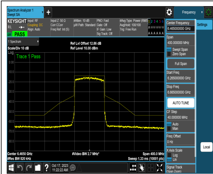
NTNV-11AX80MIMO-Ant1-6465-PASS
