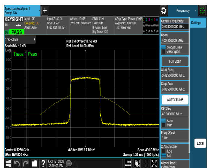
NTNV-11AX80MIMO-Ant4-6625-PASS
