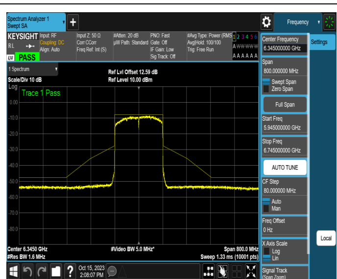
NTNV-11AX160SISO-Ant4-6345-PASS
