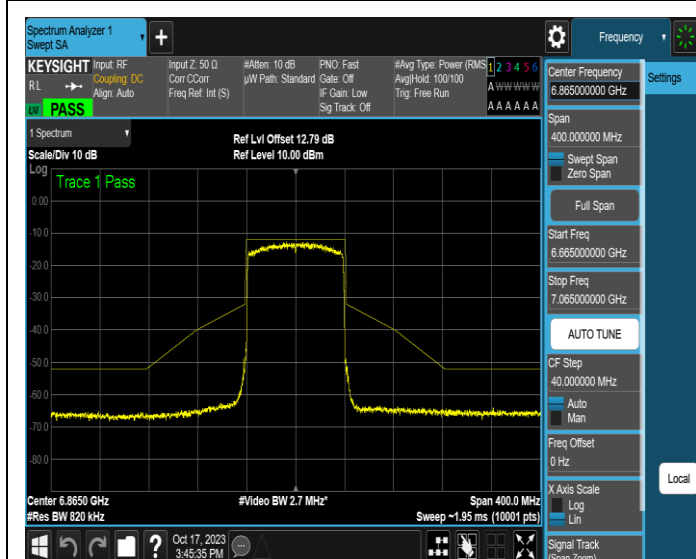
NTNV-11AX80MIMO-Ant3-6865-PASS
