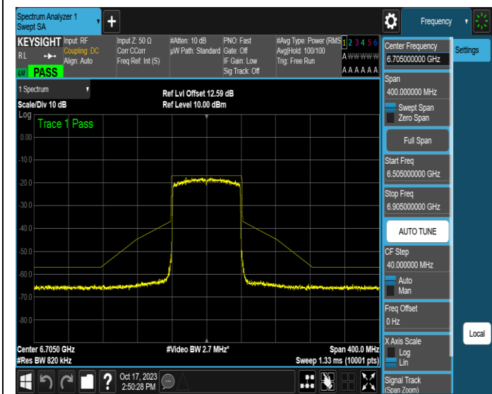
NTNV-11AX80MIMO-Ant3-6705-PASS
