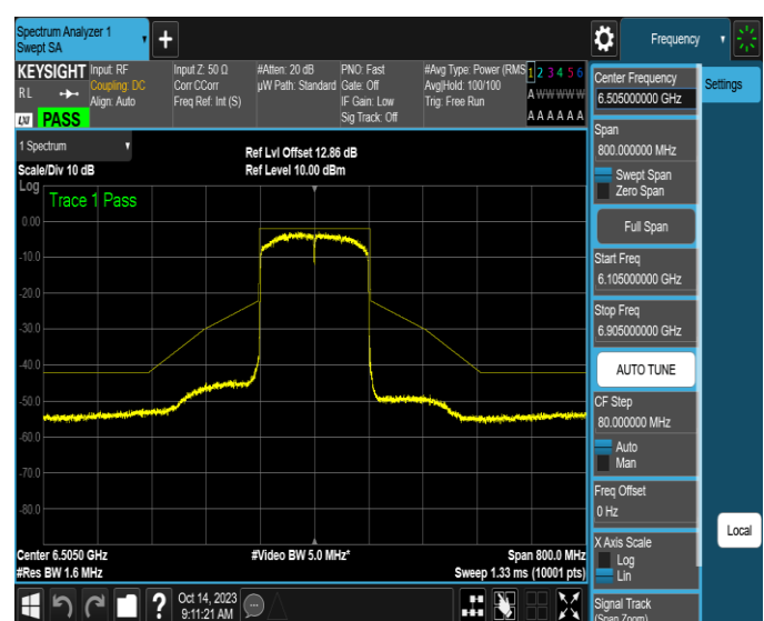
NTNV-11AX160SISO-Ant2-6505-PASS
