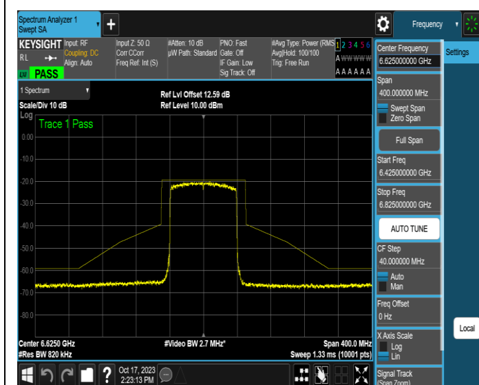
NTNV-11AX80MIMO-Ant3-6625-PASS
