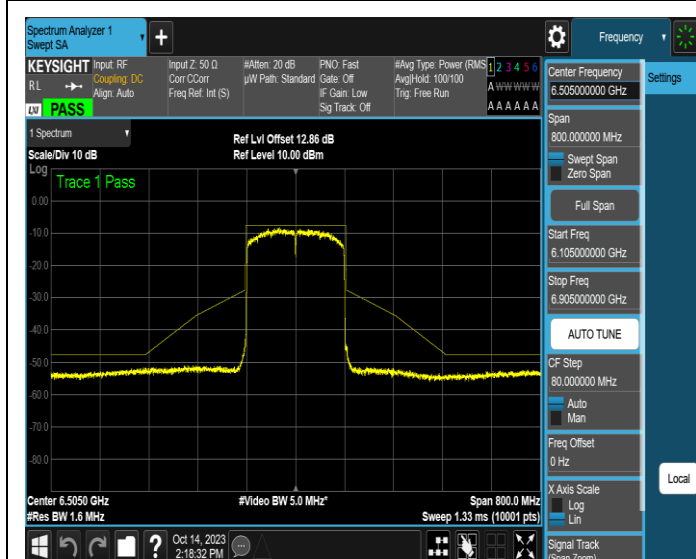
NTNV-11AX160SISO-Ant3-6505-PASS
