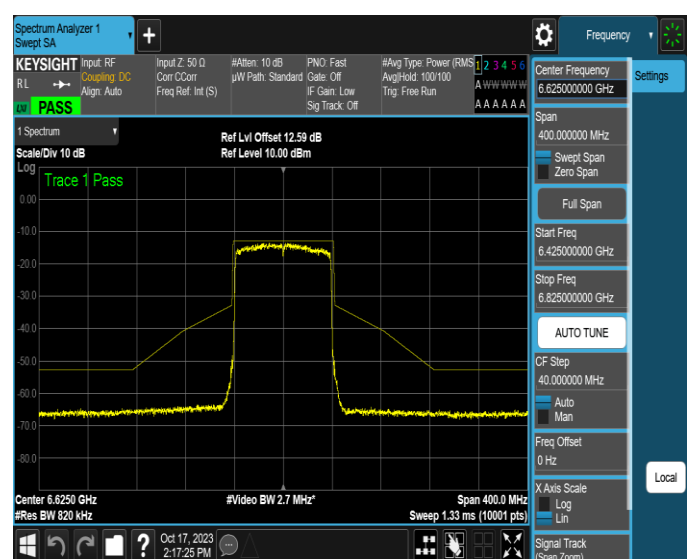
NTNV-11AX80MIMO-Ant2-6625-PASS
