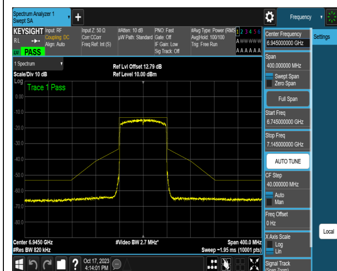
NTNV-11AX80MIMO-Ant3-6945-PASS
