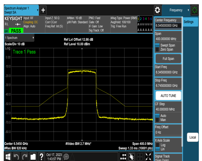
NTNV-11AX80MIMO-Ant2-6545-PASS
