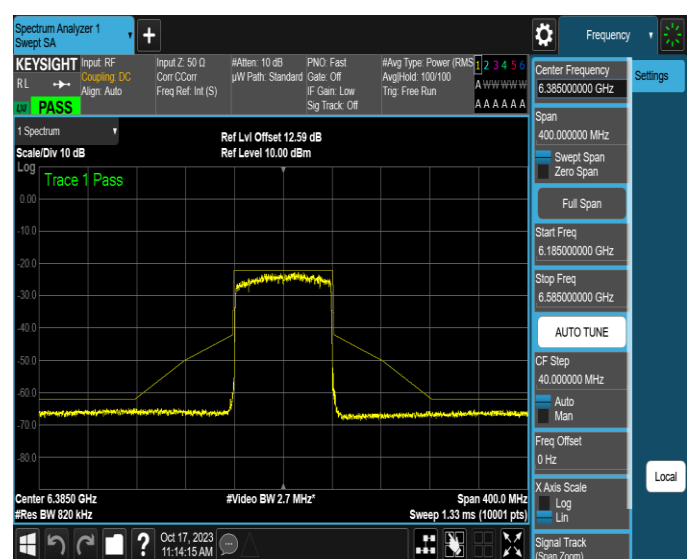
NTNV-11AX80MIMO-Ant4-6385-PASS
