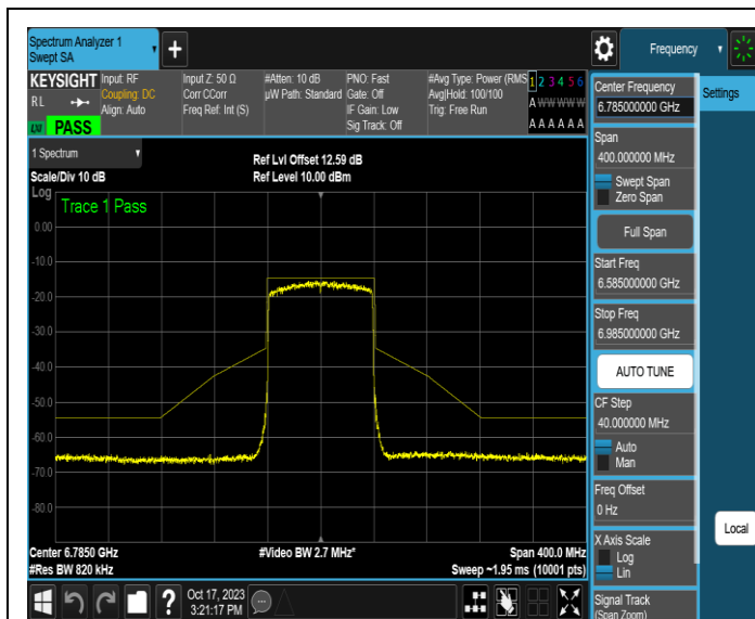
NTNV-11AX80MIMO-Ant3-6785-PASS
