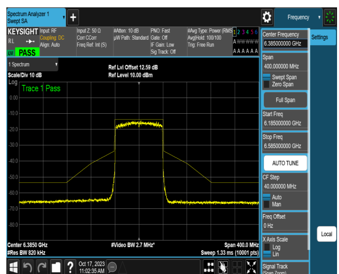
NTNV-11AX80MIMO-Ant2-6385-PASS
