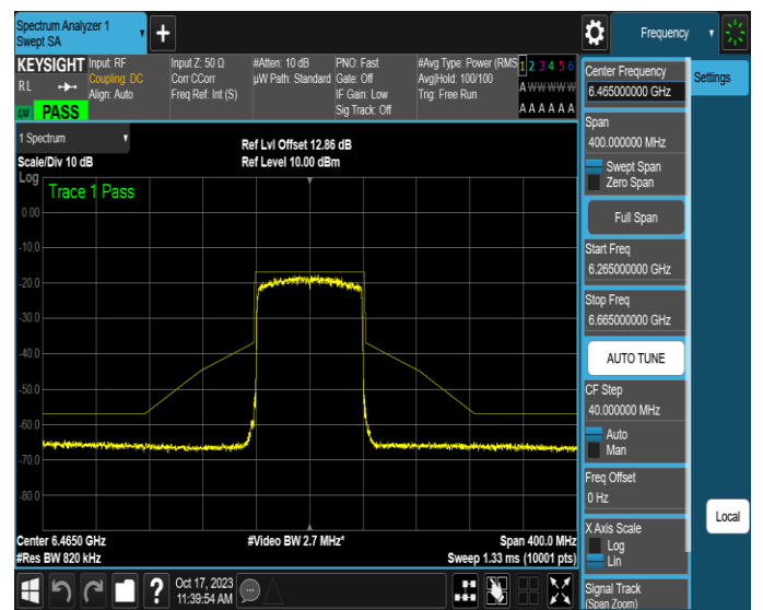
NTNV-11AX80MIMO-Ant4-6465-PASS
