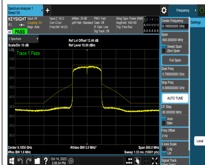
NTNV-11AX160SISO-Ant3-6185-PASS
