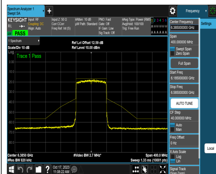
NTNV-11AX80MIMO-Ant3-6385-PASS
