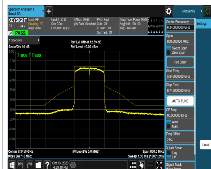
NTNV-11AX160SISO-Ant1-6345-PASS
