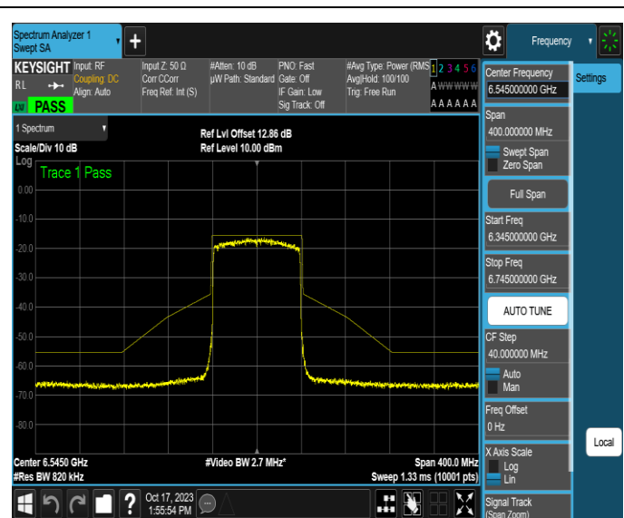
NTNV-11AX80MIMO-Ant4-6545-PASS
