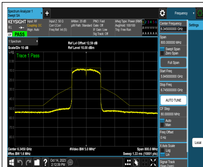
NTNV-11AX160SISO-Ant3-6345-PASS
