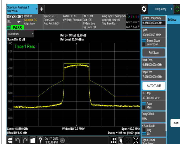
NTNV-11AX80MIMO-Ant1-6865-PASS
