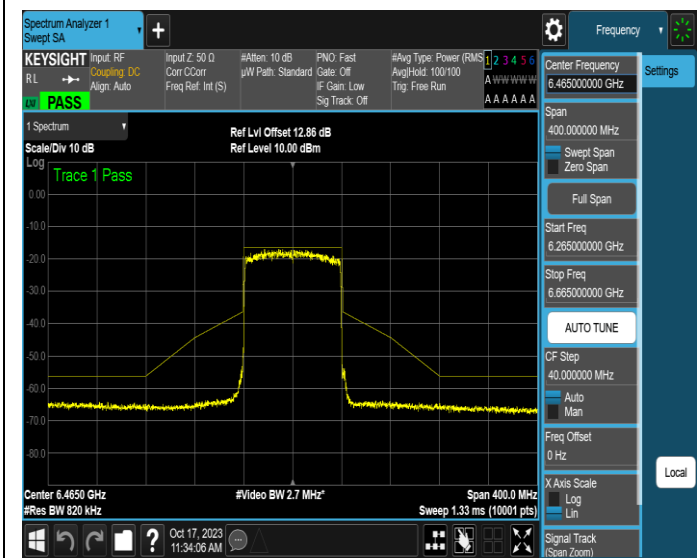
NTNV-11AX80MIMO-Ant3-6465-PASS
