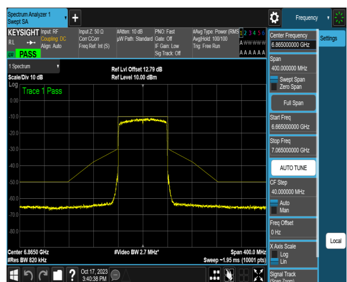
NTNV-11AX80MIMO-Ant2-6865-PASS
