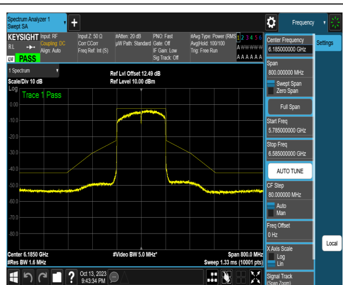
NTNV-11AX160SISO-Ant2-6185-PASS
