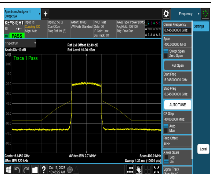
NTNV-11AX80MIMO-Ant4-6145-PASS
