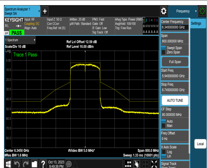
NTNV-11AX160SISO-Ant2-6345-PASS
