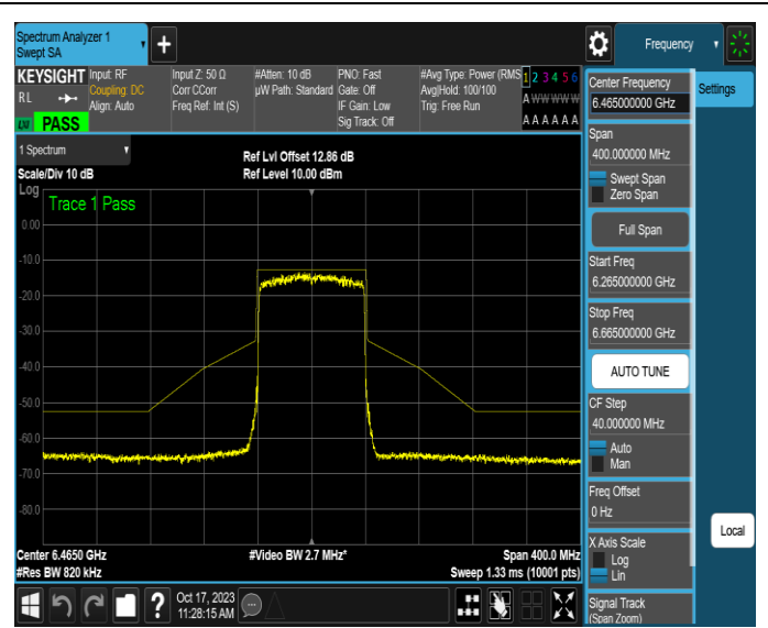
NTNV-11AX80MIMO-Ant2-6465-PASS
