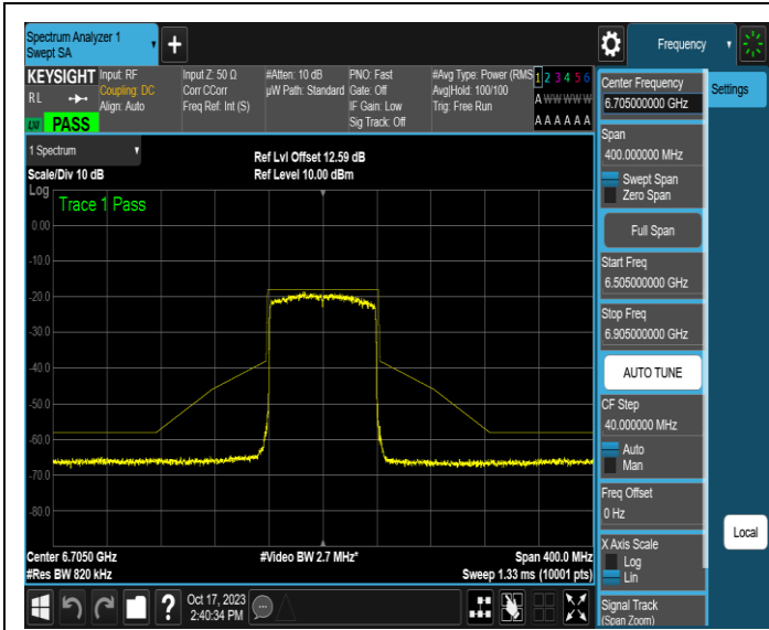
NTNV-11AX80MIMO-Ant1-6705-PASS
