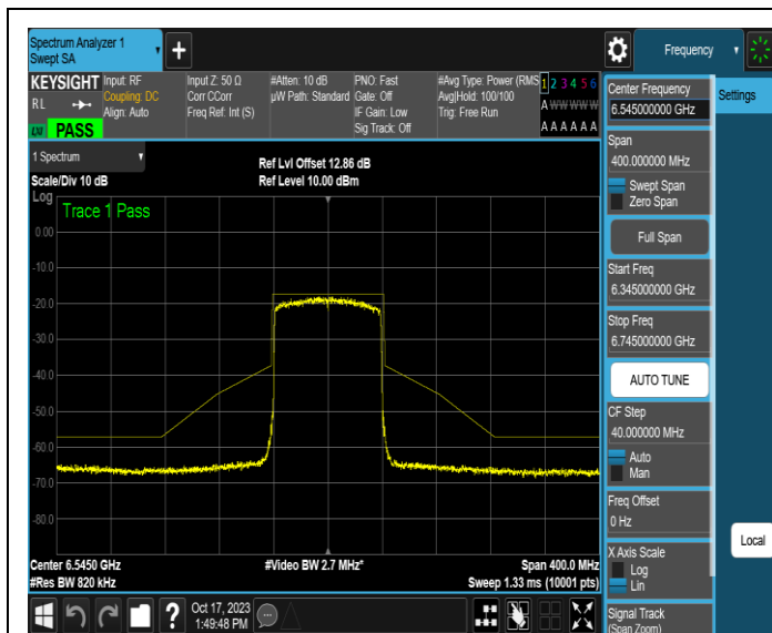
NTNV-11AX80MIMO-Ant3-6545-PASS
