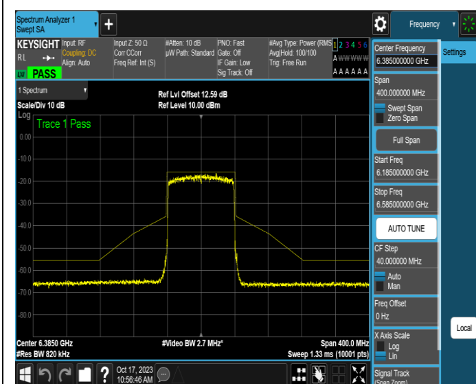
NTNV-11AX80MIMO-Ant1-6385-PASS
