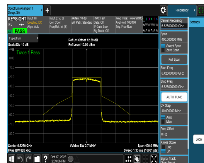
NTNV-11AX80MIMO-Ant1-6625-PASS
