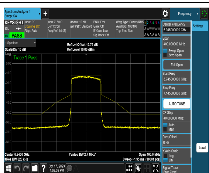
NTNV-11AX80MIMO-Ant2-6945-PASS
