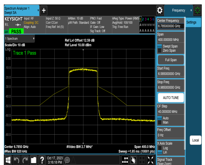
NTNV-11AX80MIMO-Ant2-6785-PASS
