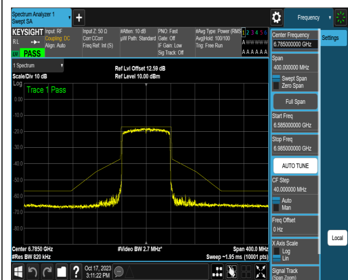
NTNV-11AX80MIMO-Ant1-6785-PASS
