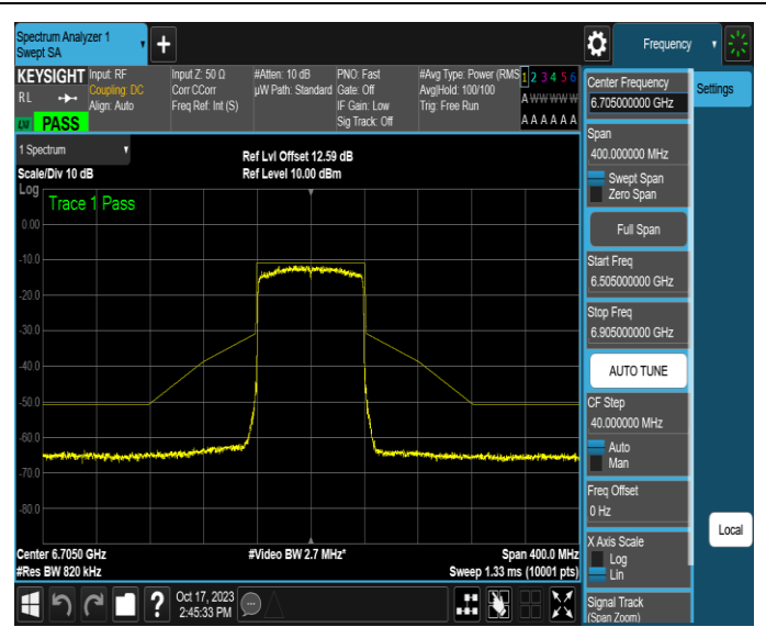
NTNV-11AX80MIMO-Ant2-6705-PASS
