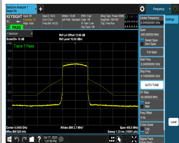
NTNV-11AX80MIMO-Ant1-6545-PASS
