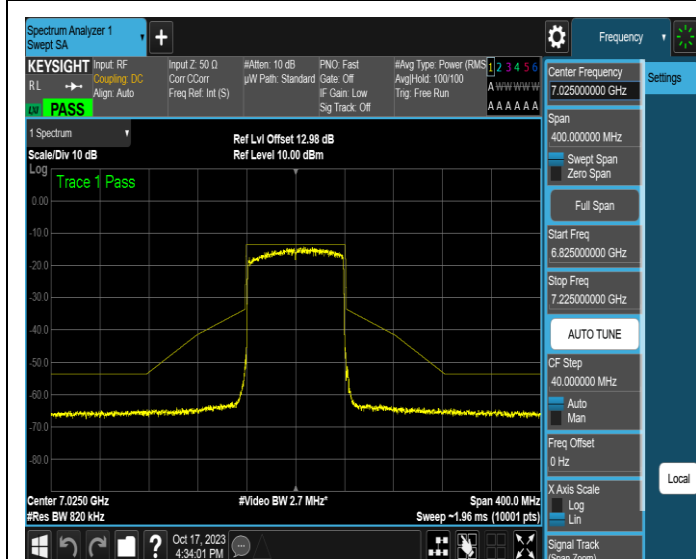
NTNV-11AX80MIMO-Ant1-7025-PASS
