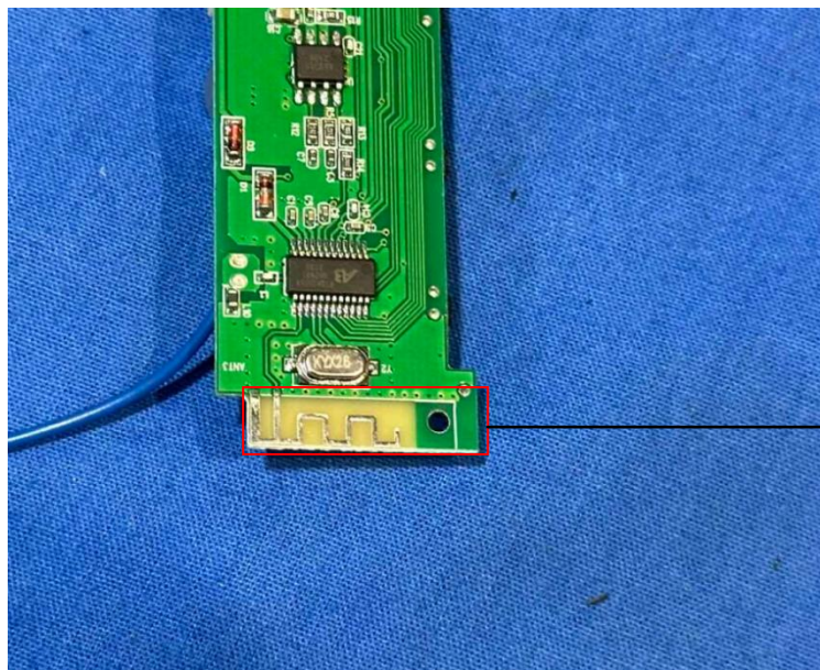
BT Antenna
