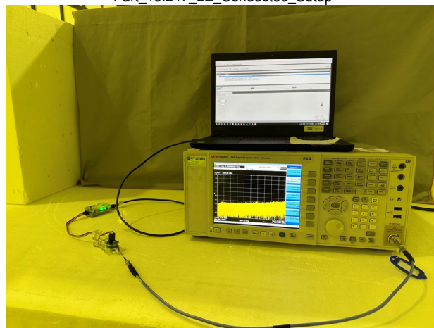
Part_15.247_LE_Conducted_Setup
