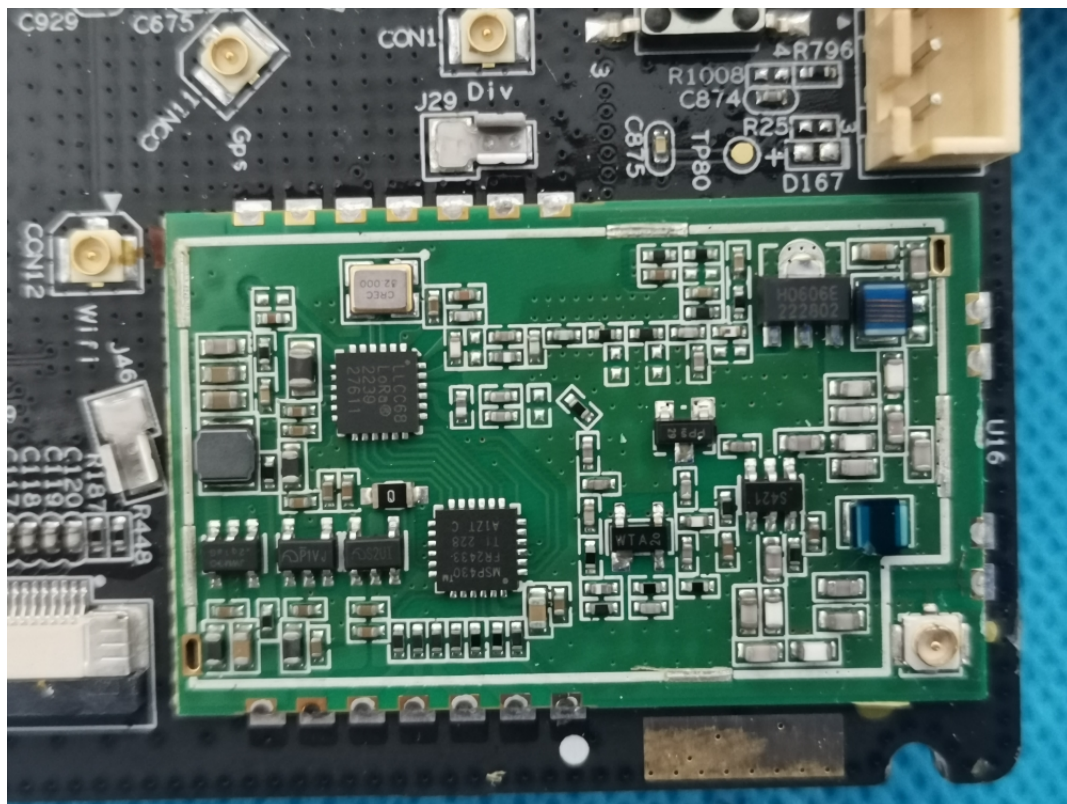
LoRa Module unshielded
