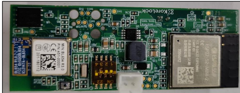
KL-PCB-550 PCB with Shield front side
