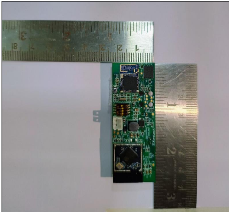
PCB Dimensional View
