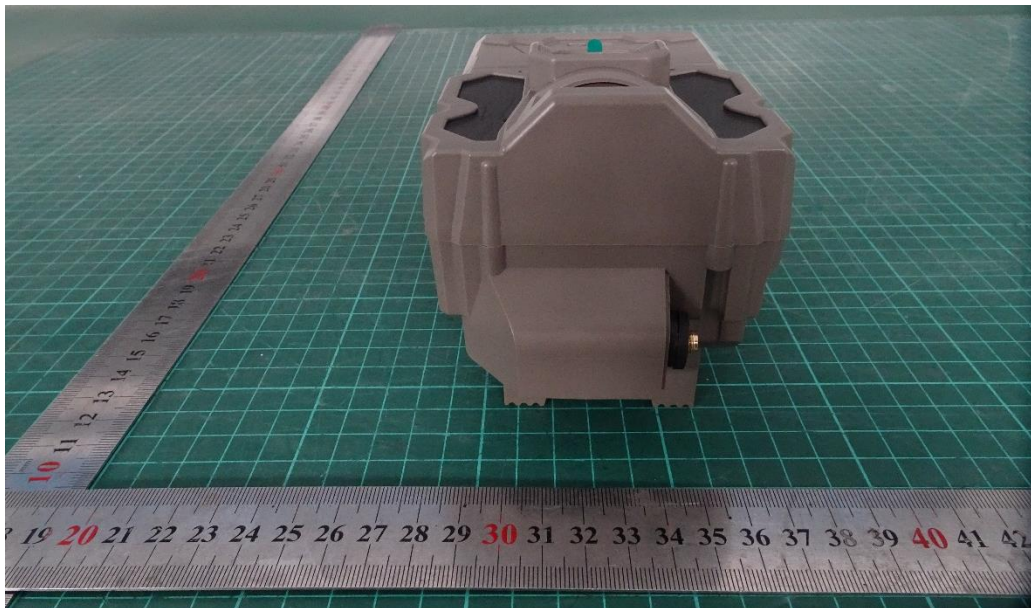
Picture 1: Constituents of EUT
