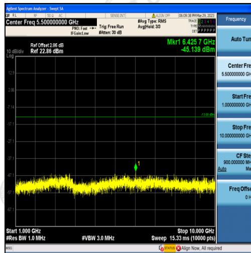
Band17-5MHz-16QAM-23755-25RB#0-Range2:1000~10000MHz
