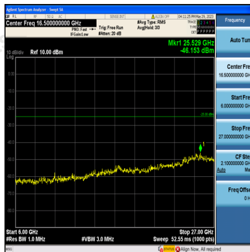
Band7-15MHz-QPSK-20825-75RB#0-Range3:6000~27000MHz
