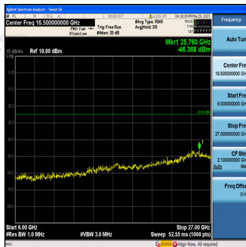
Band7-15MHz-QPSK-21375-75RB#0-Range3:6000~27000MHz
