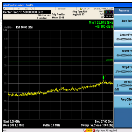
Band7-15MHz-16QAM-21375-75RB#0-Range3:6000~27000MHz
