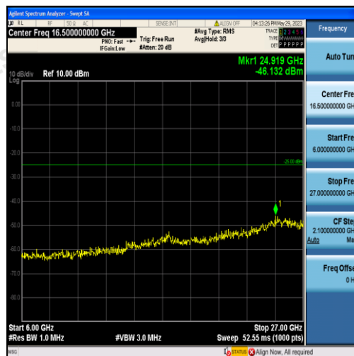
Band7-15MHz-16QAM-20825-75RB#0-Range3:6000~27000MHz
