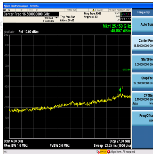
Band7-15MHz-QPSK-21100-75RB#0-Range3:6000~27000MHz
