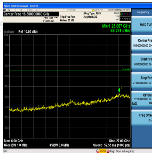
Band7-15MHz-16QAM-21100-75RB#0-Range3:6000~27000MHz
