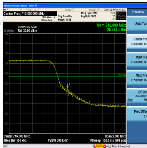
Band17-5MHz-QPSK-23825-25RB#0
