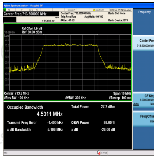
Band17-5MHz-16QAM-23825-25RB#0-4.5011
