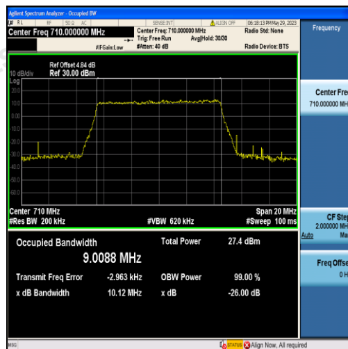
Band17-10MHz-16QAM-23790-50RB#0-9.0088
