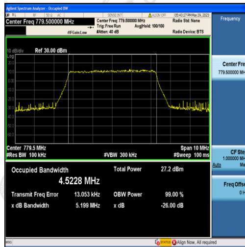
Band13-5MHz-16QAM-23205-25RB#0-4.5228
