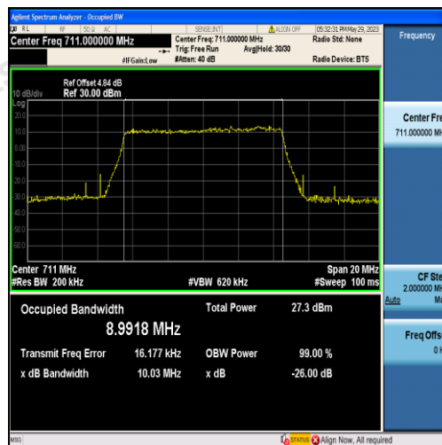
Band12-10MHz-16QAM-23130-50RB#0-8.9918
