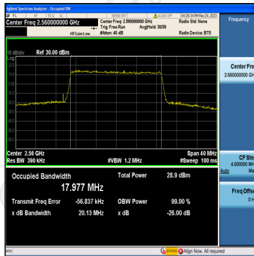
Band7-20MHz-QPSK-21350-100RB#0-17.977
