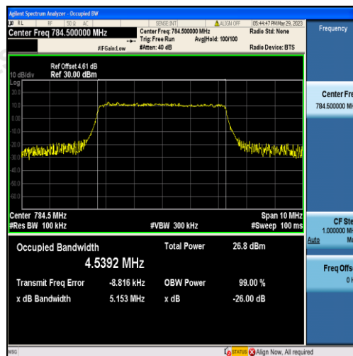
Band13-5MHz-16QAM-23255-25RB#0-4.5392
