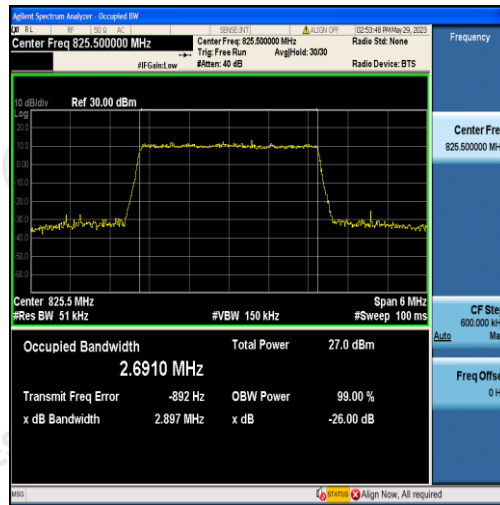
Band5-3MHz-QPSK-20415-15RB#0-2.6910
