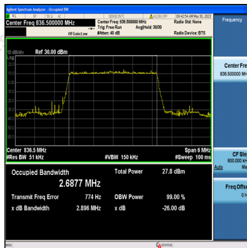
Band5-3MHz-QPSK-20525-15RB#0-2.6877
