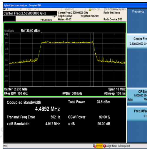
Band7-5MHz-QPSK-21100-25RB#0-4.4892
