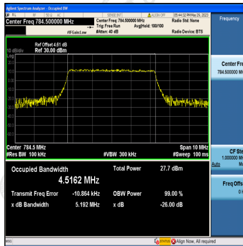
Band13-5MHz-QPSK-23255-25RB#0-4.5162
