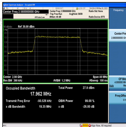
Band7-20MHz-16QAM-21350-100RB#0-17.962
