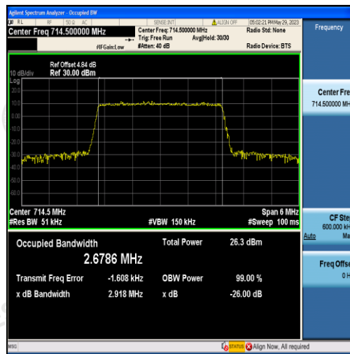
Band12-3MHz-16QAM-23165-15RB#0-2.6786
