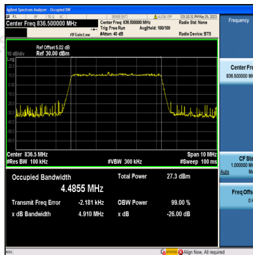
Band5-5MHz-16QAM-20525-25RB#0-4.4855
