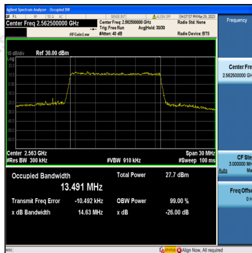
Band7-15MHz-16QAM-21375-75RB#0-13.491
