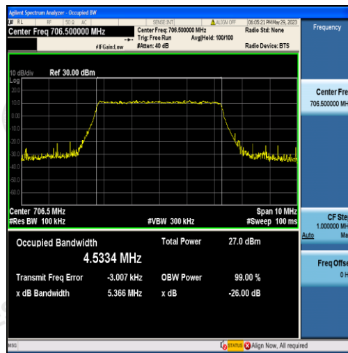
Band17-5MHz-16QAM-23755-25RB#0-4.5334
