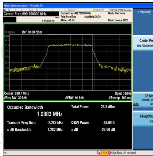
Band12-1.4MHz-QPSK-23017-6RB#0-1.0883
