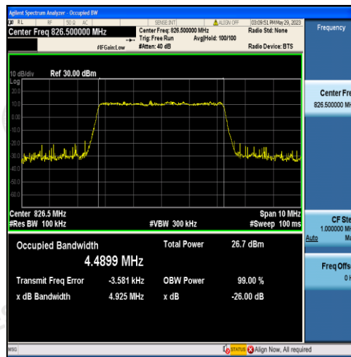
Band5-5MHz-16QAM-20425-25RB#0-4.4899
