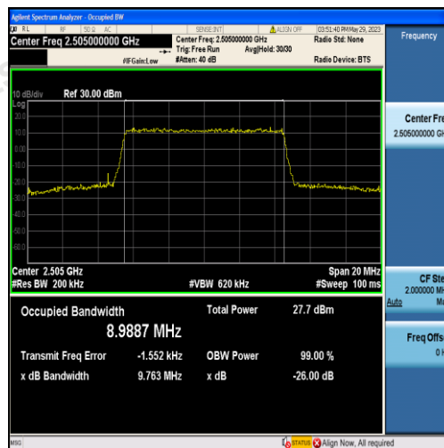
Band7-10MHz-16QAM-20800-50RB#0-8.9887
