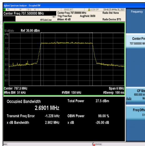
Band12-3MHz-QPSK-23095-15RB#0-2.6901
