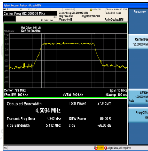
Band13-5MHz-16QAM-23230-25RB#0-4.5084
