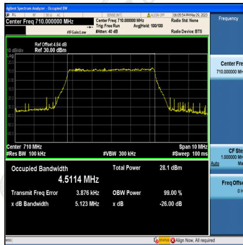
Band17-5MHz-QPSK-23790-25RB#0-4.5114
