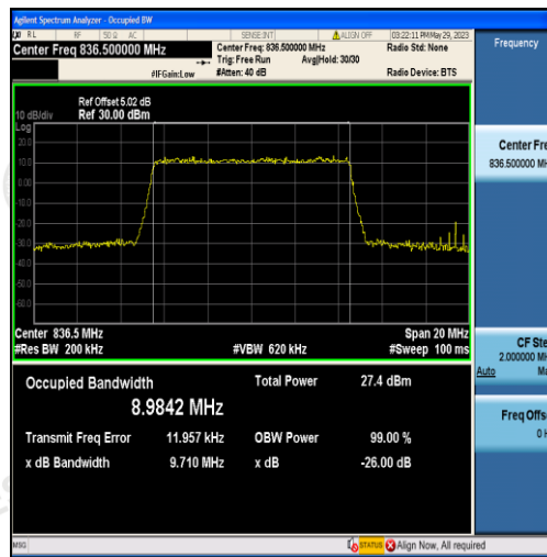
Band5-10MHz-16QAM-20525-50RB#0-8.9842
