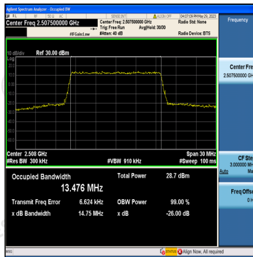
Band7-15MHz-QPSK-20825-75RB#0-13.476
