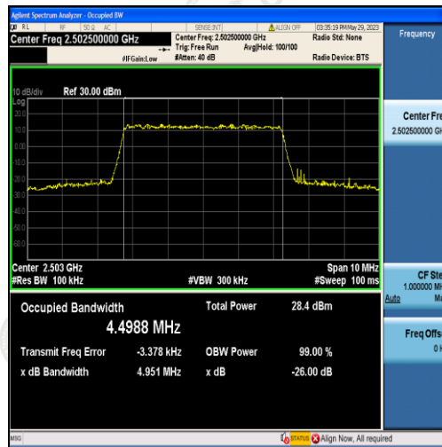
Band7-5MHz-QPSK-20775-25RB#0-4.4988
