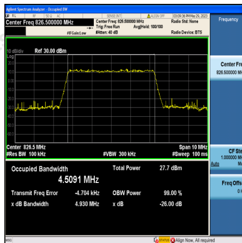
Band5-5MHz-QPSK-20425-25RB#0-4.5091
