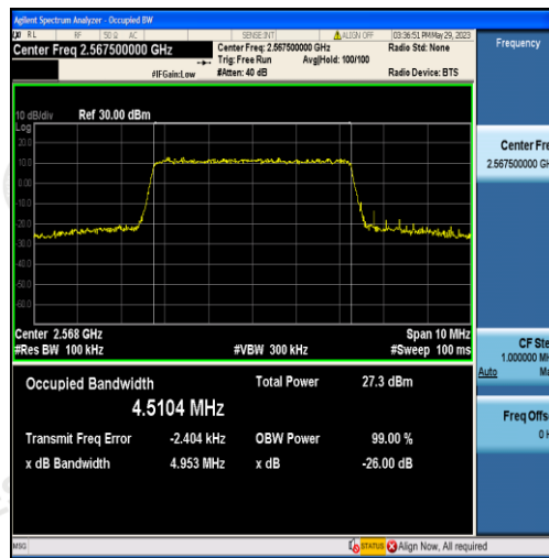
Band7-5MHz-16QAM-21425-25RB#0-4.5104
