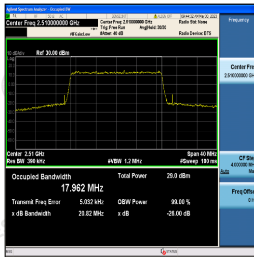
Band7-20MHz-QPSK-20850-100RB#0-17.962
