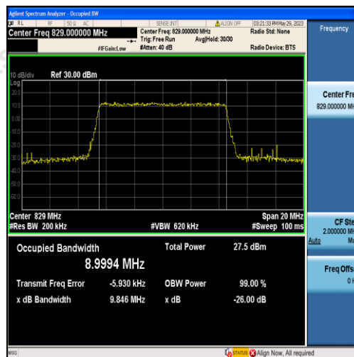
Band5-10MHz-QPSK-20450-50RB#0-8.9994
