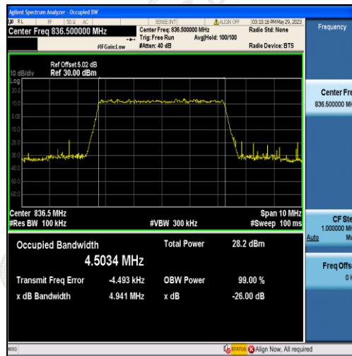
Band5-5MHz-QPSK-20525-25RB#0-4.5034
