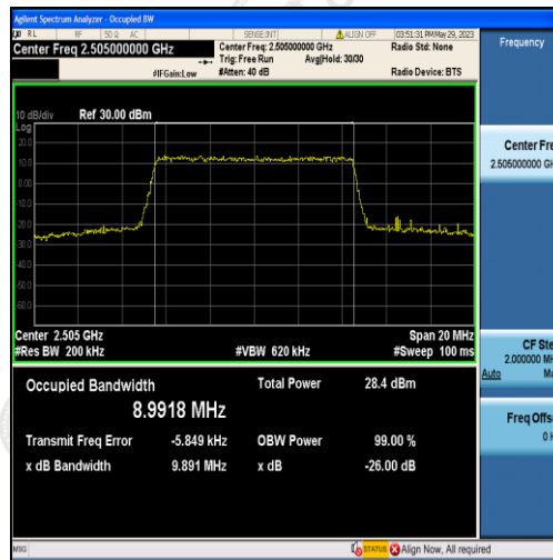
Band7-10MHz-QPSK-20800-50RB#0-8.9918
