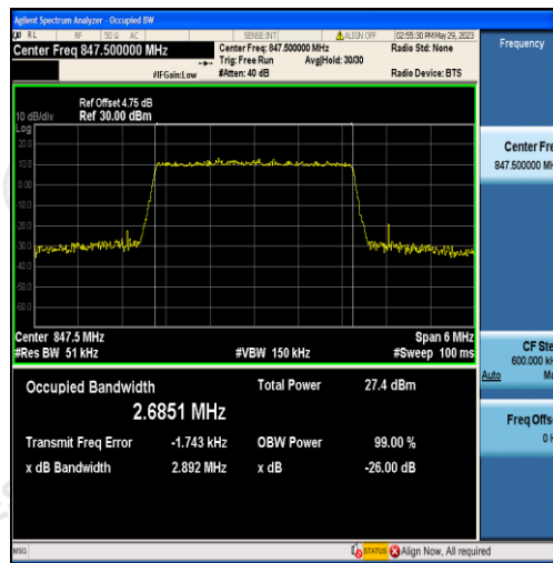
Band5-3MHz-QPSK-20635-15RB#0-2.6851
