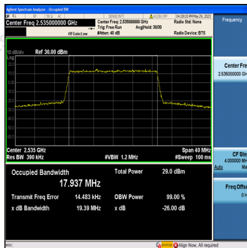
Band7-20MHz-QPSK-21100-100RB#0-17.937
