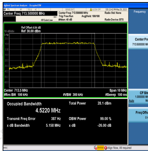
Band12-5MHz-QPSK-23155-25RB#0-4.5220
