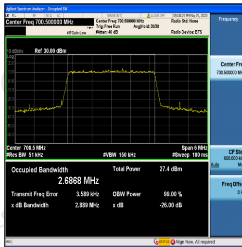
Band12-3MHz-QPSK-23025-15RB#0-2.6868
