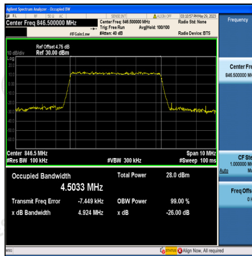
Band5-5MHz-QPSK-20625-25RB#0-4.5033
