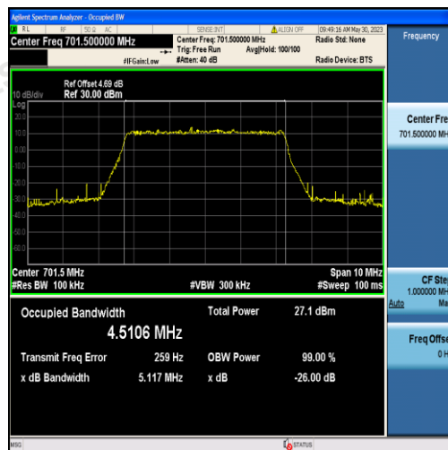
Band12-5MHz-16QAM-23035-25RB#0-4.5106
