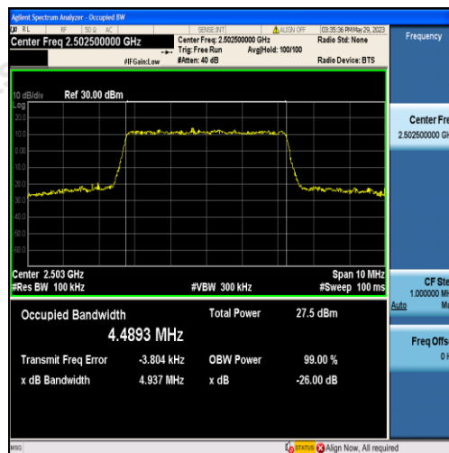
Band7-5MHz-16QAM-20775-25RB#0-4.4893
