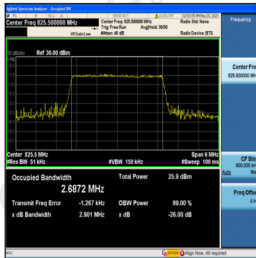
Band5-3MHz-16QAM-20415-15RB#0-2.6872
