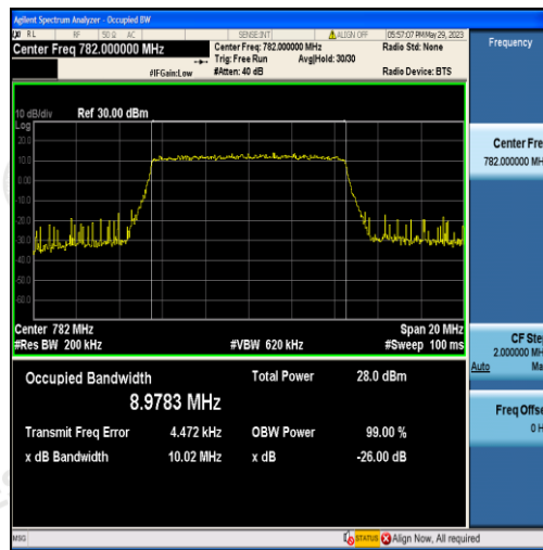
Band13-10MHz-QPSK-23230-50RB#0-8.9783
