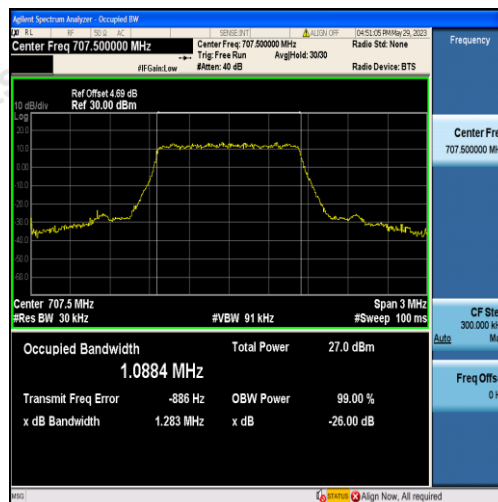
Band12-1.4MHz-QPSK-23095-6RB#0-1.0884
