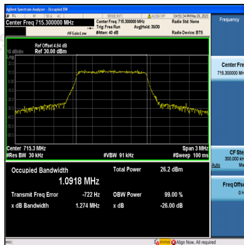
Band12-1.4MHz-16QAM-23173-6RB#0-1.0918
