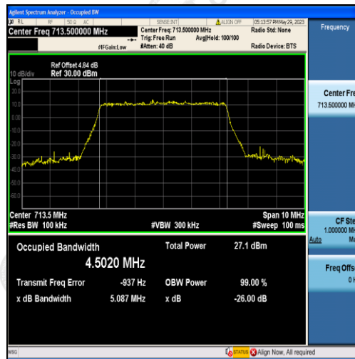
Band12-5MHz-16QAM-23155-25RB#0-4.5020
