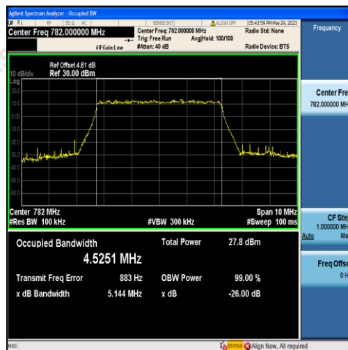
Band13-5MHz-QPSK-23230-25RB#0-4.5251
