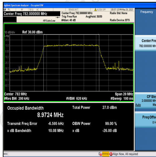
Band13-10MHz-16QAM-23230-50RB#0-8.9724
