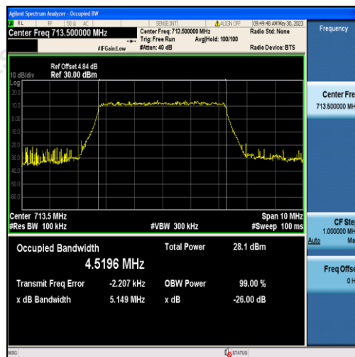
Band17-5MHz-QPSK-23825-25RB#0-4.5196
