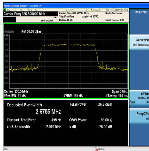
Band5-3MHz-16QAM-20525-15RB#0-2.6755
