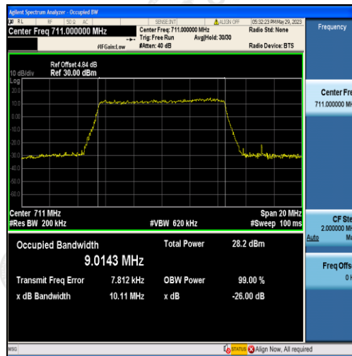
Band12-10MHz-QPSK-23130-50RB#0-9.0143
