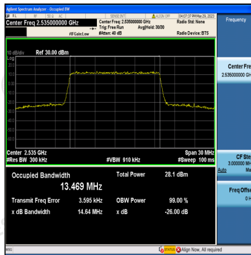
Band7-15MHz-16QAM-21100-75RB#0-13.469
