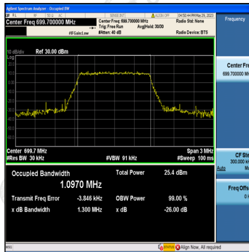
Band12-1.4MHz-16QAM-23017-6RB#0-1.0970
