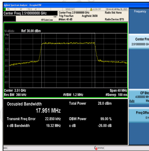
Band7-20MHz-16QAM-20850-100RB#0-17.951
