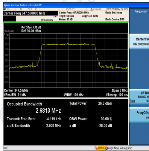
Band5-3MHz-16QAM-20635-15RB#0-2.6813
