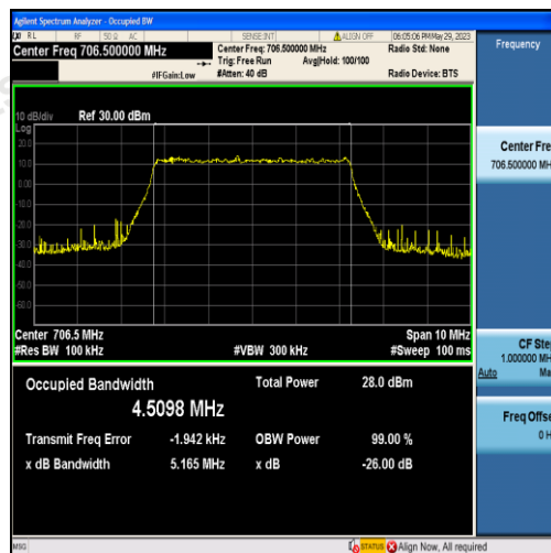
Band17-5MHz-QPSK-23755-25RB#0-4.5098
