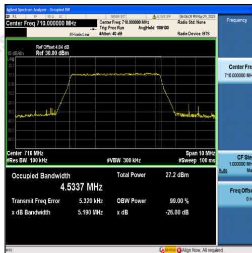
Band17-5MHz-16QAM-23790-25RB#0-4.5337
