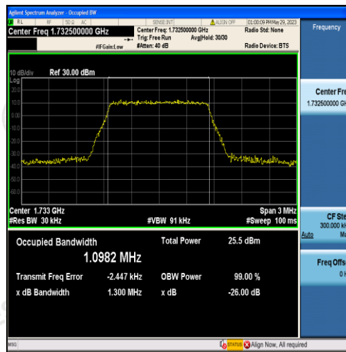
Band4-1.4MHz-16QAM-20175-6RB#0-1.0982
