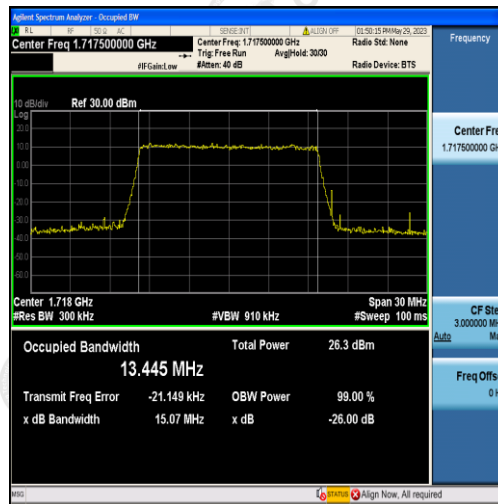
Band4-15MHz-16QAM-20025-75RB#0-13.445
