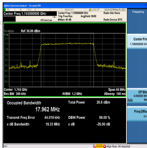
Band4-20MHz-16QAM-20300-100RB#0-17.962
