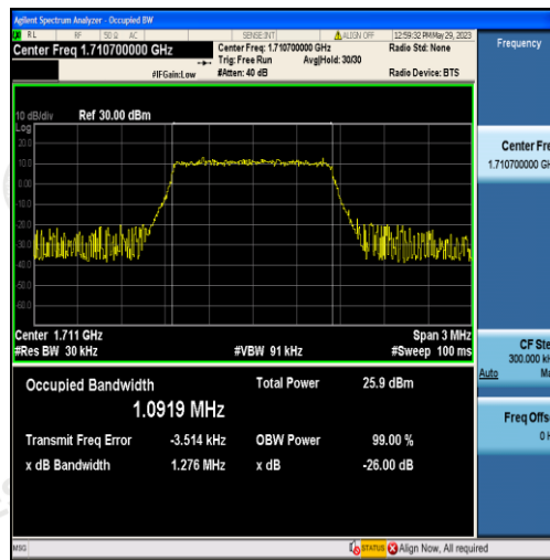
Band4-1.4MHz-QPSK-19957-6RB#0-1.0919
