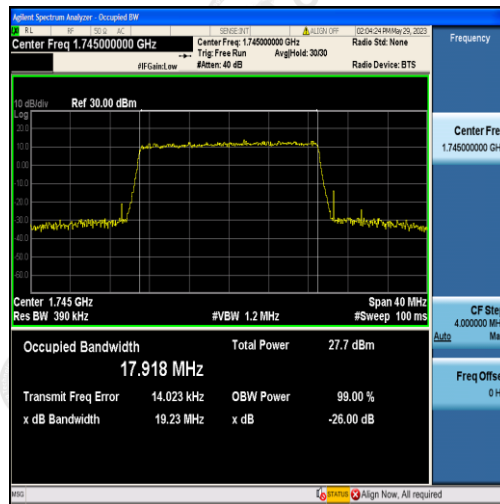
Band4-20MHz-QPSK-20300-100RB#0-17.918
