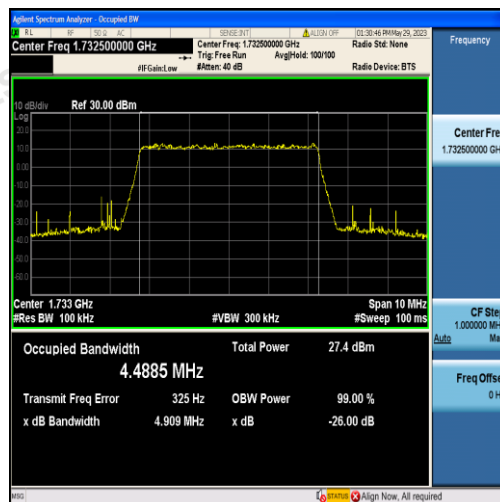
Band4-5MHz-QPSK-20175-25RB#0-4.4885
