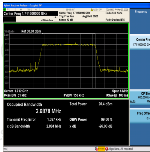
Band4-3MHz-QPSK-19965-15RB#0-2.6878
