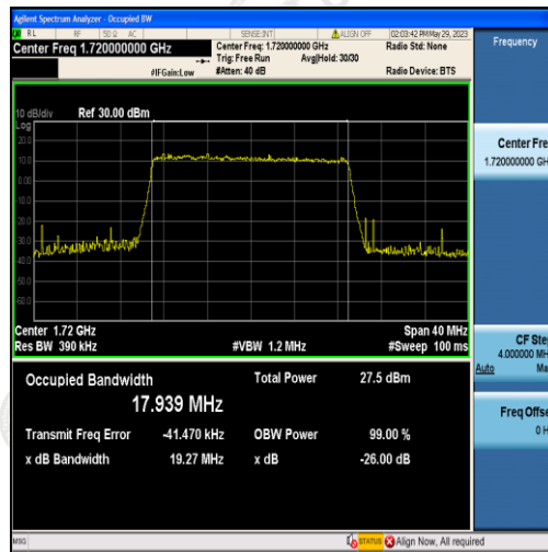
Band4-20MHz-QPSK-20050-100RB#0-17.939
