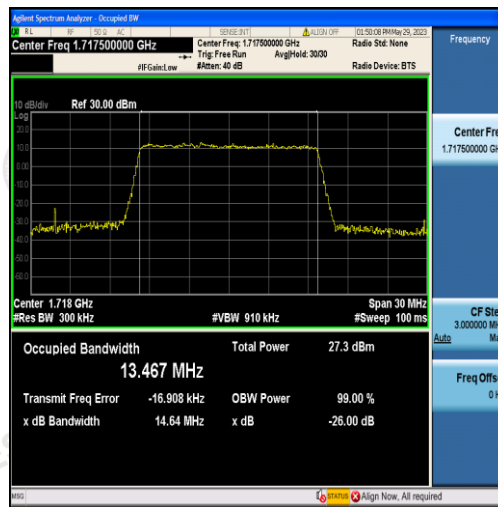
Band4-15MHz-QPSK-20025-75RB#0-13.467
