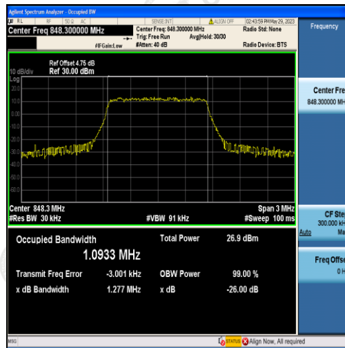
Band5-1.4MHz-QPSK-20643-6RB#0-1.0933
