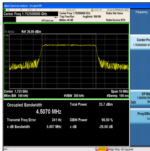
Band4-5MHz-16QAM-20375-25RB#0-4.5070
