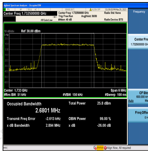
Band4-3MHz-16QAM-20175-15RB#0-2.6801
