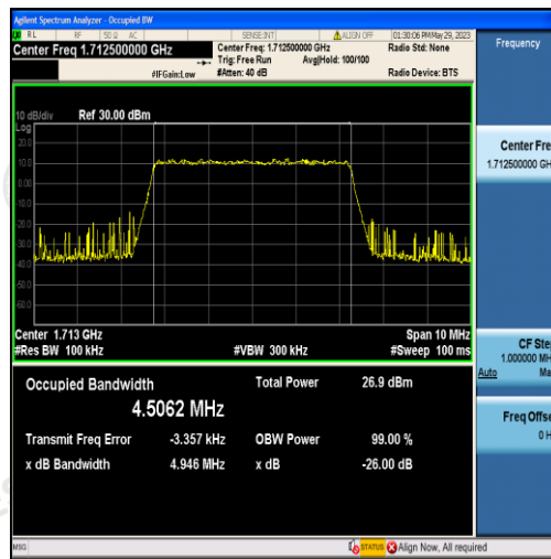
Band4-5MHz-QPSK-19975-25RB#0-4.5062
