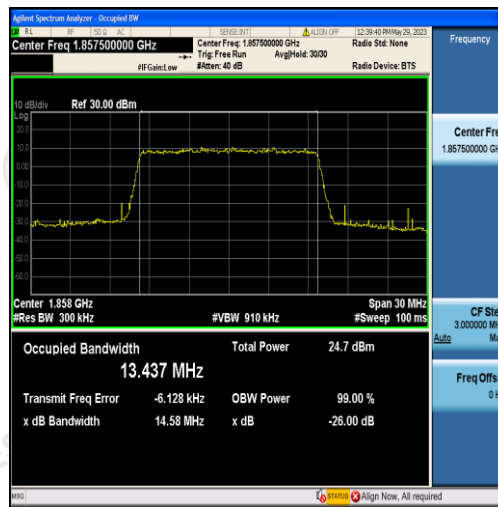
Band2-15MHz-QPSK-18675-75RB#0-13.437
