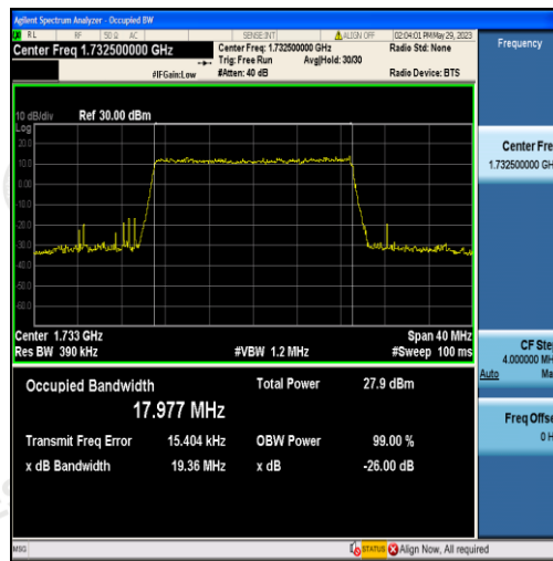
Band4-20MHz-QPSK-20175-100RB#0-17.977
