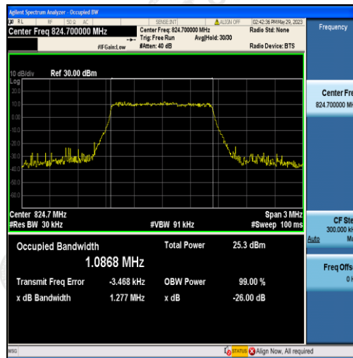
Band5-1.4MHz-16QAM-20407-6RB#0-1.0868
