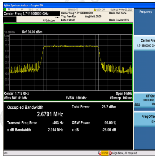
Band4-3MHz-16QAM-19965-15RB#0-2.6791
