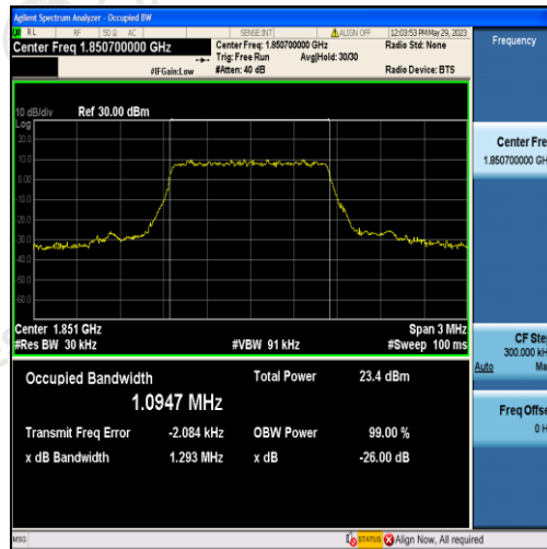
Band2-1.4MHz-QPSK-18607-6RB#0-1.0947
