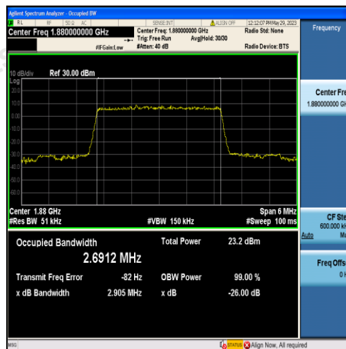
Band2-3MHz-QPSK-18900-15RB#0-2.6912
