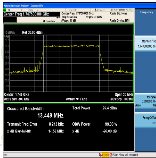
Band4-15MHz-16QAM-20325-75RB#0-13.449
