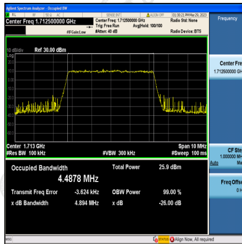
Band4-5MHz-16QAM-19975-25RB#0-4.4878
