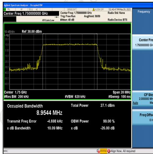
Band4-10MHz-QPSK-20350-50RB#0-8.9544
