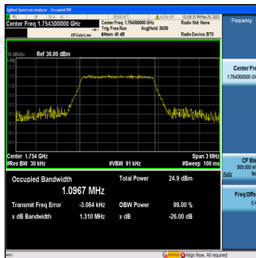
Band4-1.4MHz-16QAM-20393-6RB#0-1.0967
