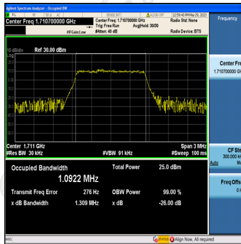
Band4-1.4MHz-16QAM-19957-6RB#0-1.0922
