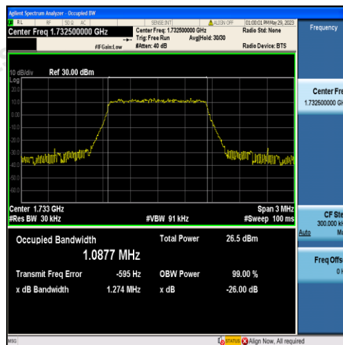
Band4-1.4MHz-QPSK-20175-6RB#0-1.0877
