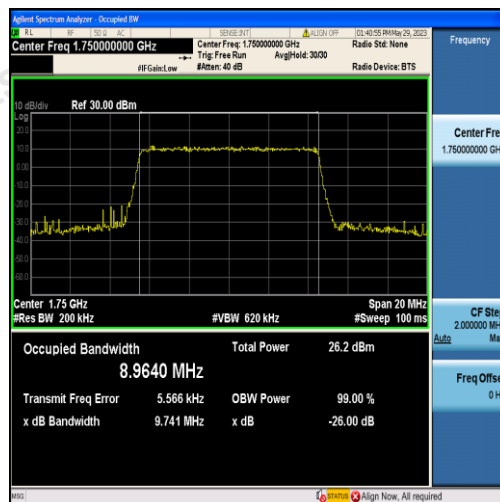
Band4-10MHz-16QAM-20350-50RB#0-8.9640
