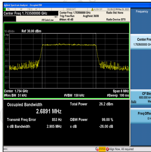
Band4-3MHz-QPSK-20385-15RB#0-2.6891
