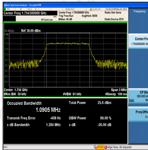
Band4-1.4MHz-QPSK-20393-6RB#0-1.0905
