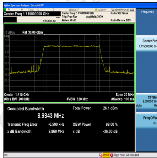
Band4-10MHz-16QAM-20000-50RB#0-8.9843
