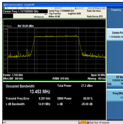
Band4-15MHz-QPSK-20325-75RB#0-13.453
