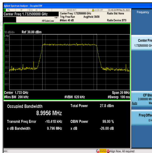
Band4-10MHz-QPSK-20175-50RB#0-8.9956
