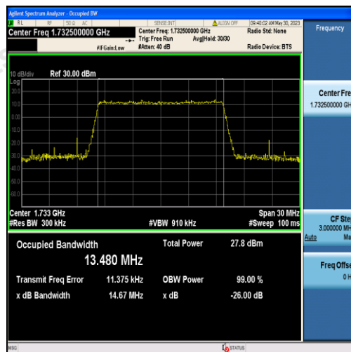
Band4-15MHz-QPSK-20175-75RB#0-13.480
