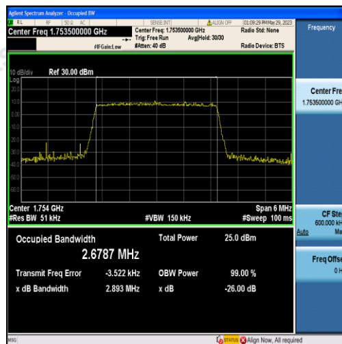
Band4-3MHz-16QAM-20385-15RB#0-2.6787
