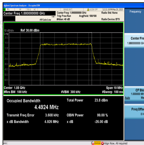
Band2-5MHz-QPSK-18900-25RB#0-4.4924
