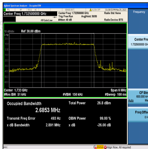
Band4-3MHz-QPSK-20175-15RB#0-2.6853
