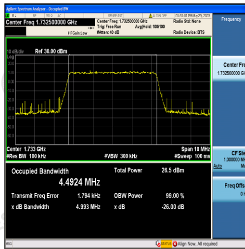
Band4-5MHz-16QAM-20175-25RB#0-4.4924
