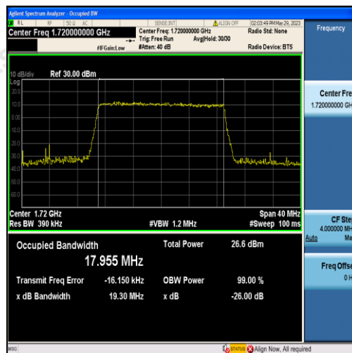
Band4-20MHz-16QAM-20050-100RB#0-17.955
