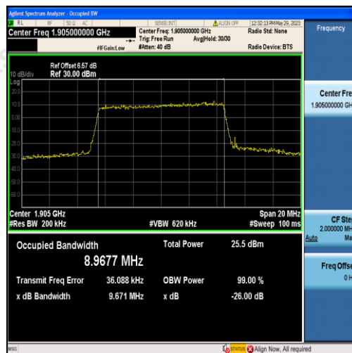
Band2-10MHz-16QAM-19150-50RB#0-8.9677
