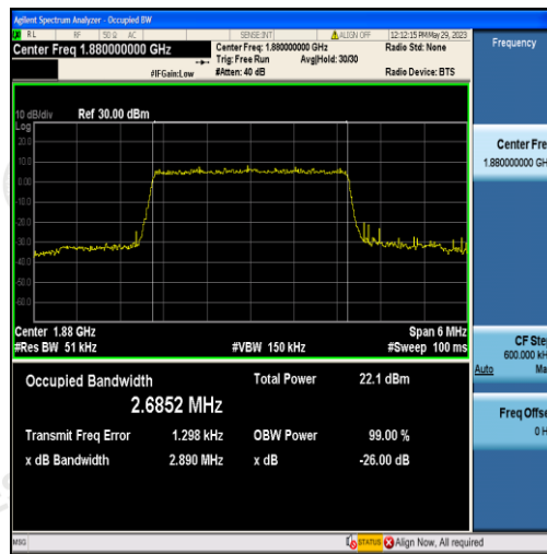
Band2-3MHz-16QAM-18900-15RB#0-2.6852
