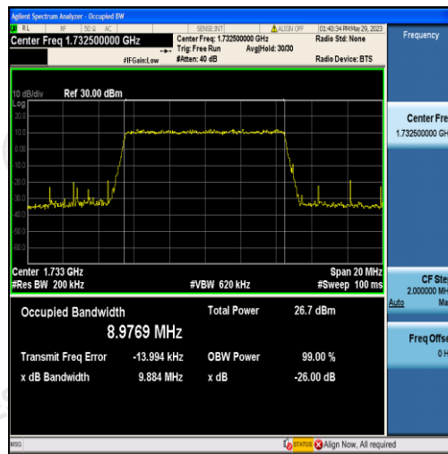
Band4-10MHz-16QAM-20175-50RB#0-8.9769
