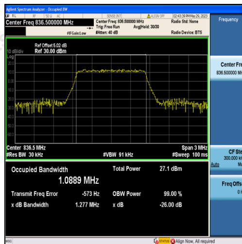
Band5-1.4MHz-QPSK-20525-6RB#0-1.0889
