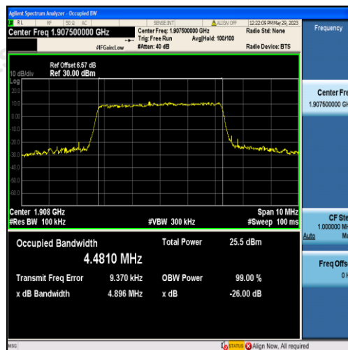
Band2-5MHz-16QAM-19175-25RB#0-4.4810
