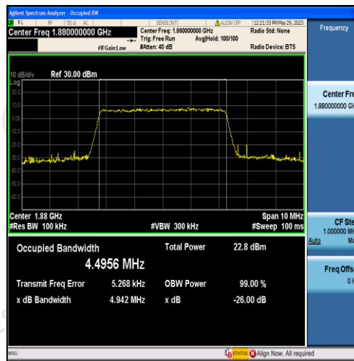
Band2-5MHz-16QAM-18900-25RB#0-4.4956
