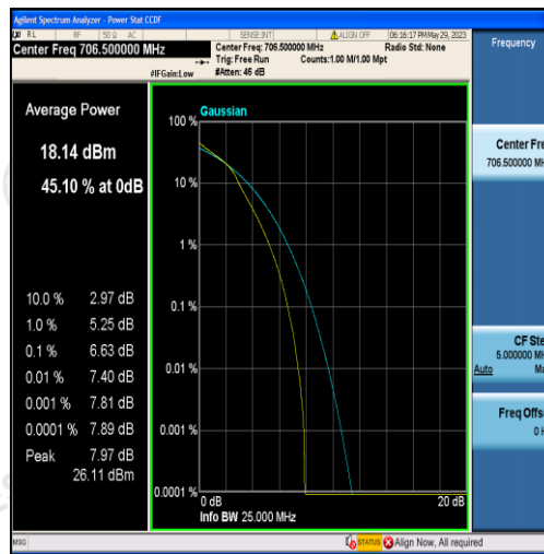
Band17-5MHz-16QAM-23755-25RB#0
