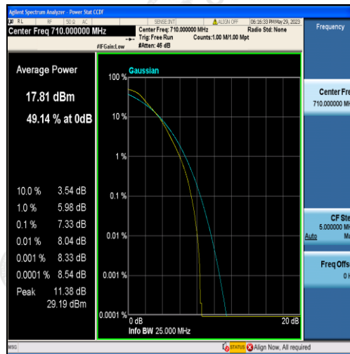
Band17-5MHz-QPSK-23790-25RB#0
