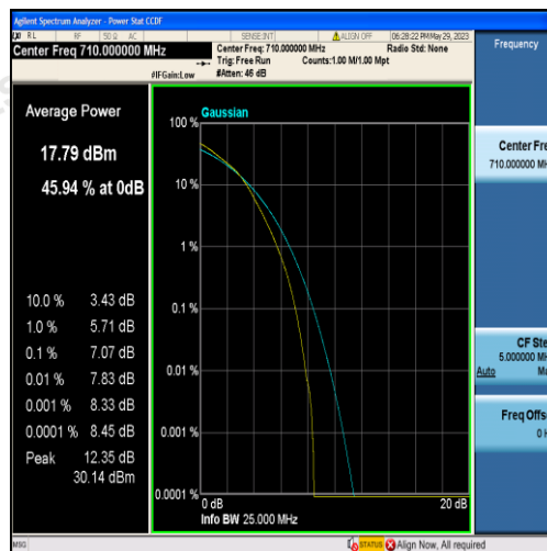
Band17-10MHz-16QAM-23790-50RB#0
