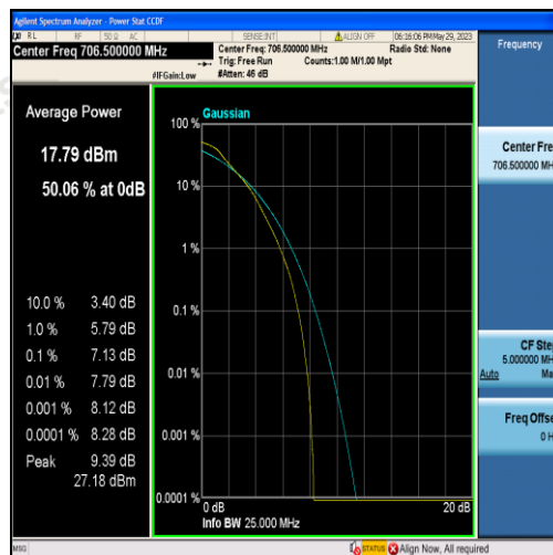
Band17-5MHz-QPSK-23755-25RB#0
