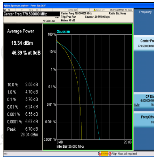
Band13-5MHz-QPSK-23205-25RB#0
