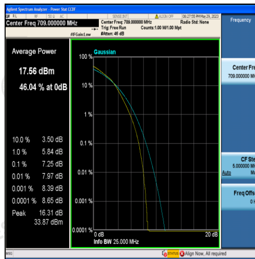
Band17-10MHz-16QAM-23780-50RB#0
