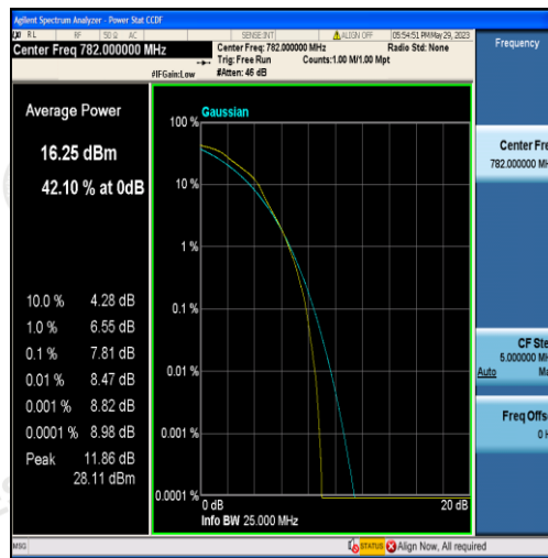
Band13-5MHz-16QAM-23230-25RB#0
