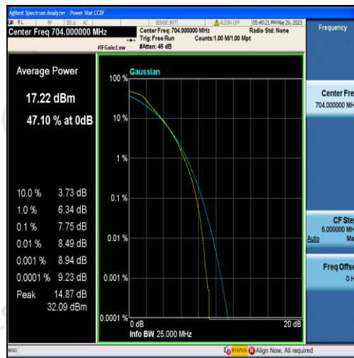
Band12-10MHz-QPSK-23060-50RB#0
