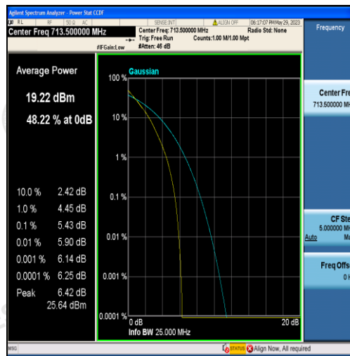
Band17-5MHz-QPSK-23825-25RB#0
