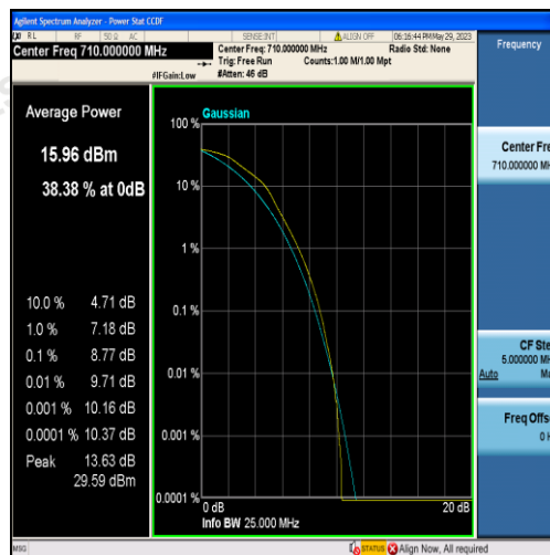
Band17-5MHz-16QAM-23790-25RB#0
