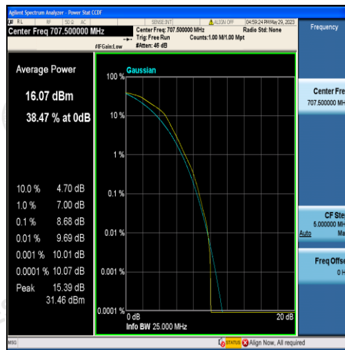
Band12-1.4MHz-16QAM-23095-6RB#0
