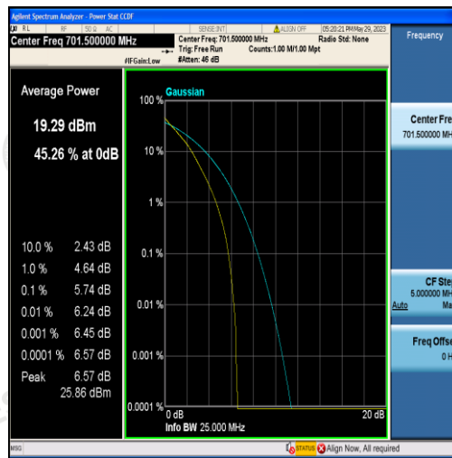
Band12-5MHz-QPSK-23035-25RB#0
