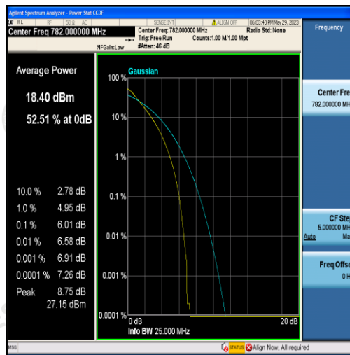
Band13-10MHz-QPSK-23230-50RB#0
