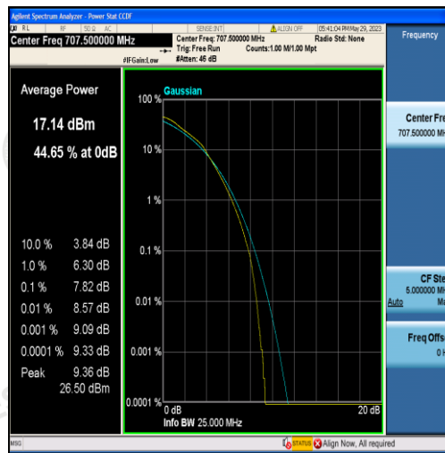
Band12-10MHz-16QAM-23095-50RB#0
