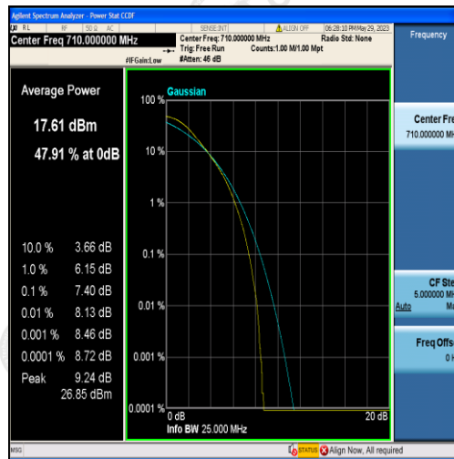
Band17-10MHz-QPSK-23790-50RB#0
