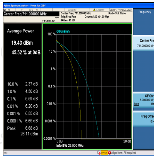
Band17-10MHz-QPSK-23800-50RB#0
