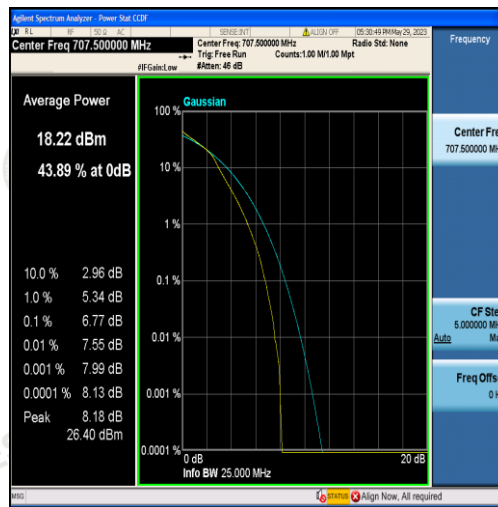
Band12-5MHz-16QAM-23095-25RB#0
