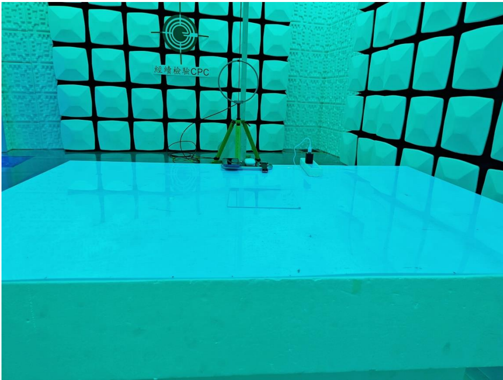
Setup Photo FCC ID: 2BBMP-D301
