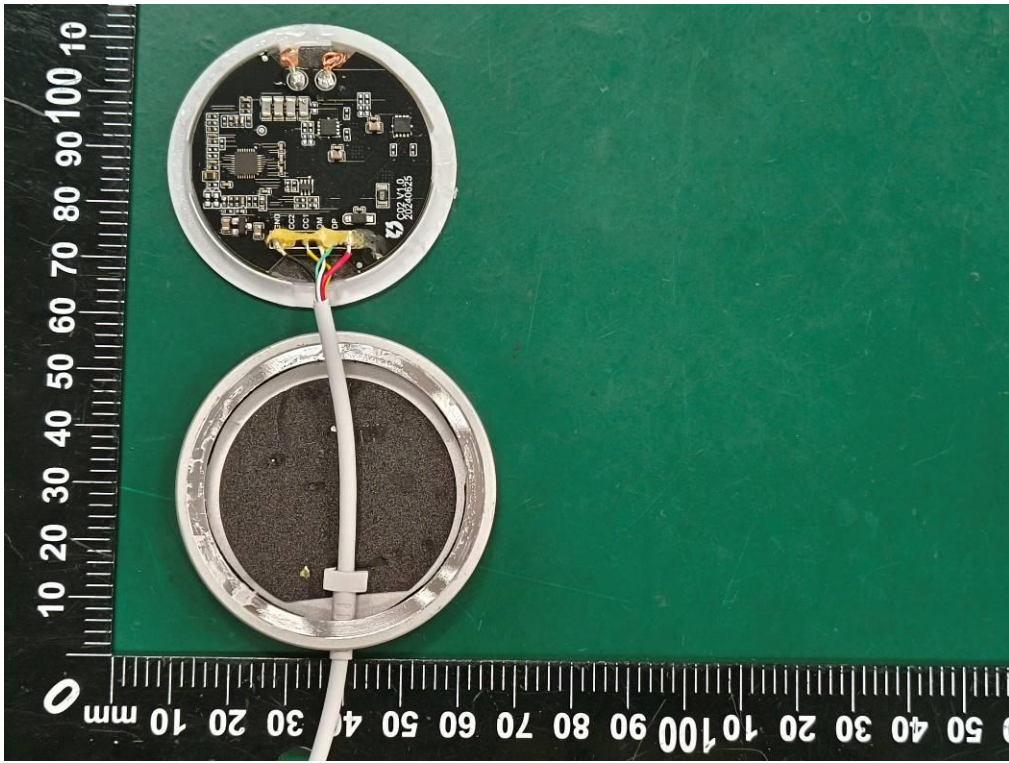
Internal Photo FCC ID: 2BBMP-C0102
