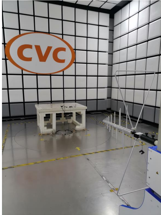
(2) Radiated emission Test Setup (Below 1GHz)
