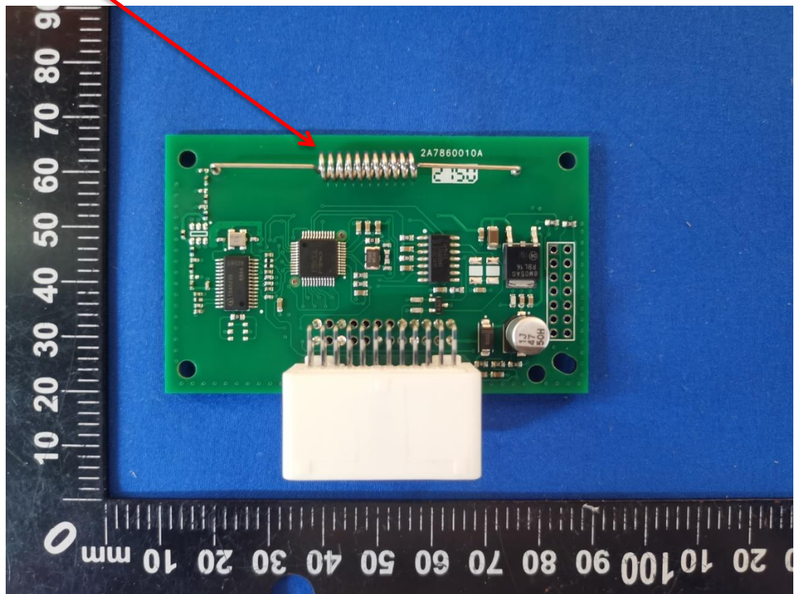
Receive Antenna
