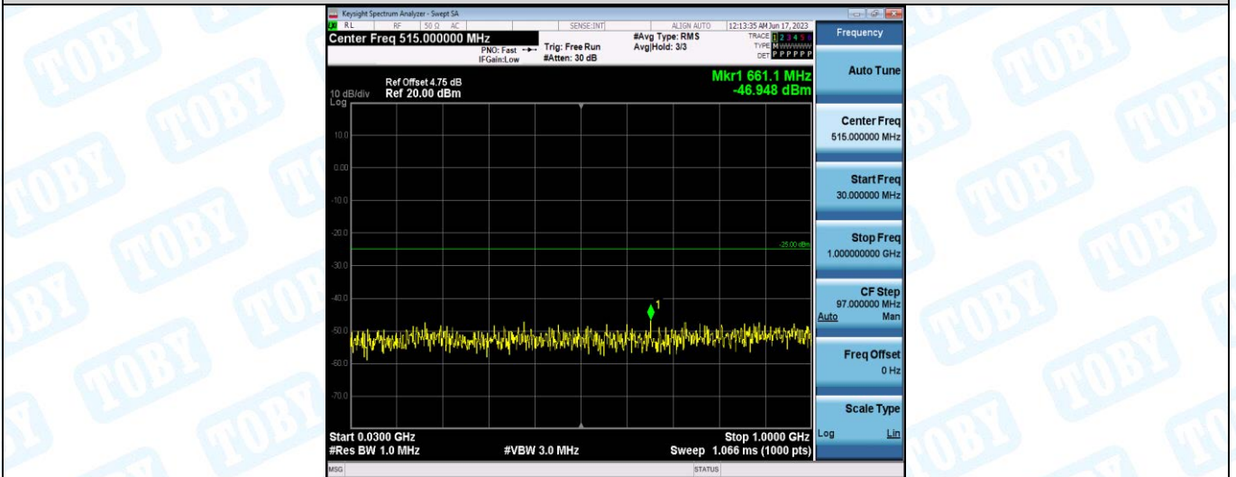
Band41-5MHz-QPSK-41215-1RB#0-Range3:30~1000MHz
