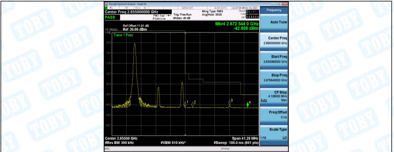
Band41-15MHz-QPSK-41165-1RB#74
