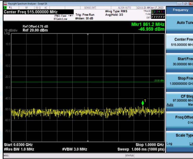
Band41-5MHz-16QAM-40215-1RB#0-Range1:30~1000MHz
