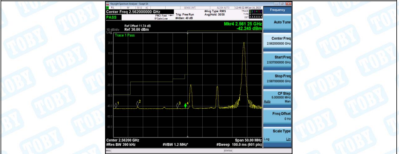
Band41-20MHz-QPSK-40410-100RB#0
