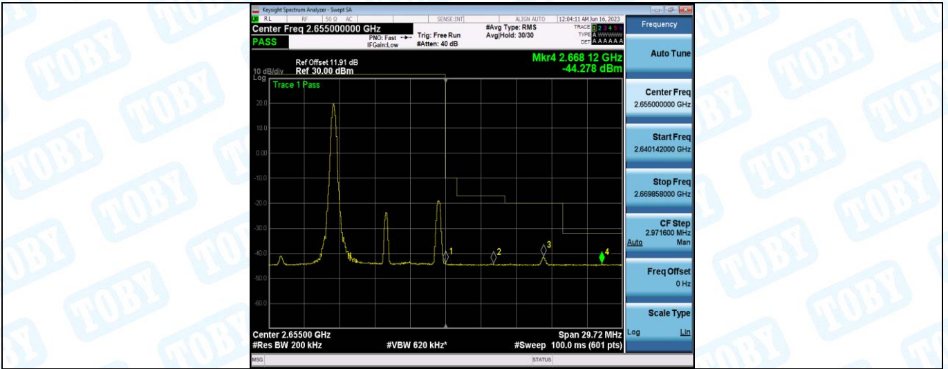
Band41-10MHz-QPSK-41190-1RB#49
