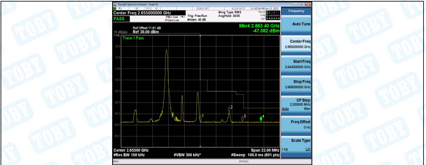
Band41-5MHz-16QAM-41215-1RB#24
