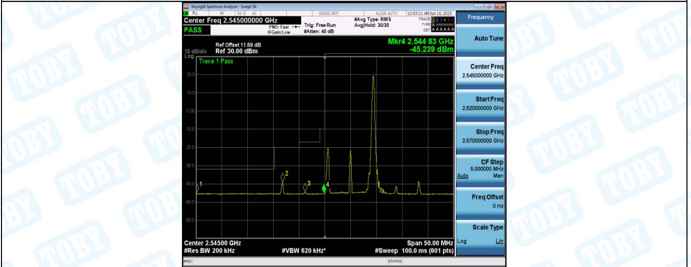
Band41-10MHz-16QAM-40190-50RB#0
