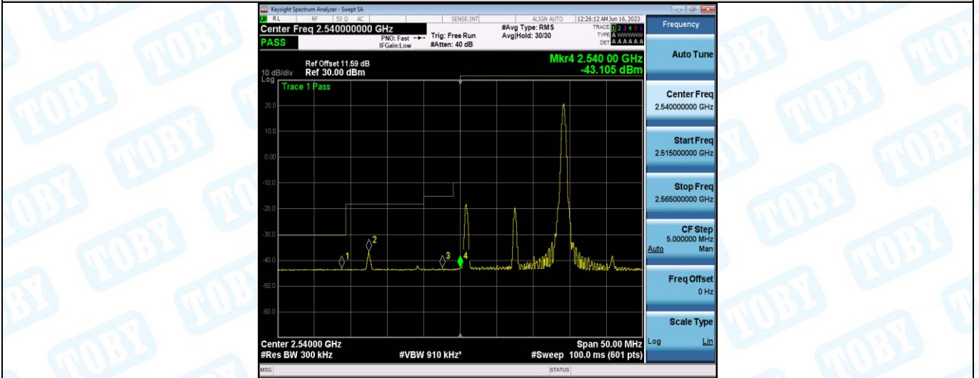
Band41-15MHz-QPSK-40165-75RB#0
