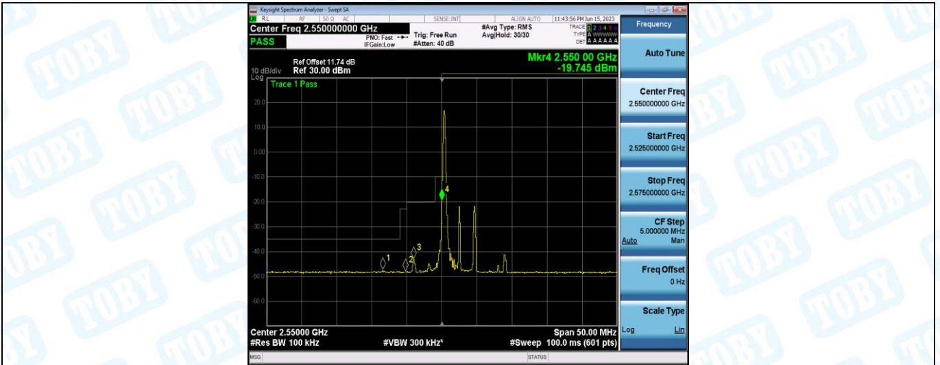
Band41-5MHz-16QAM-40215-1RB#24
