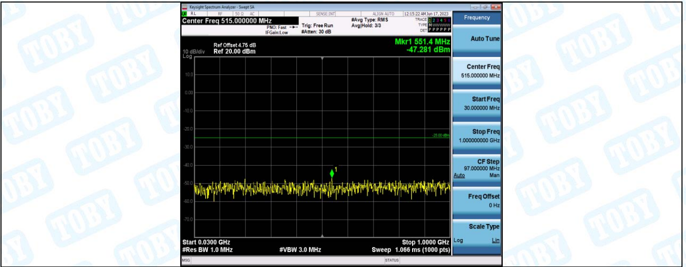
Band41-10MHz-QPSK-40190-1RB#0-Range1:30~1000MHz
