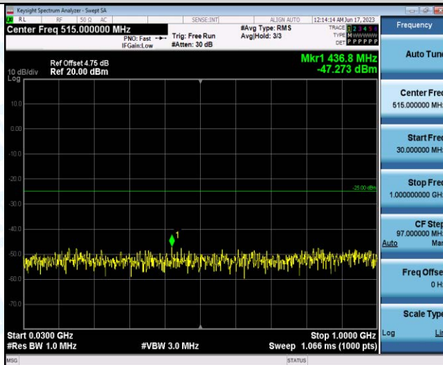
Band41-5MHz-16QAM-41215-1RB#0-Range3:30~1000MHz
