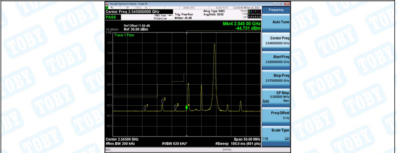
Band41-10MHz-QPSK-40190-50RB#0
