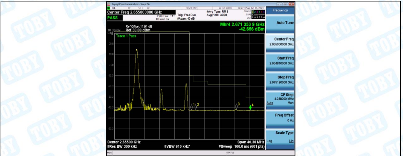
Band41-15MHz-16QAM-41165-1RB#74
