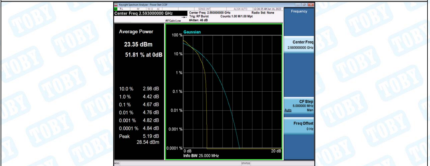
Band41-15MHz-QPSK-40620-75RB#0
