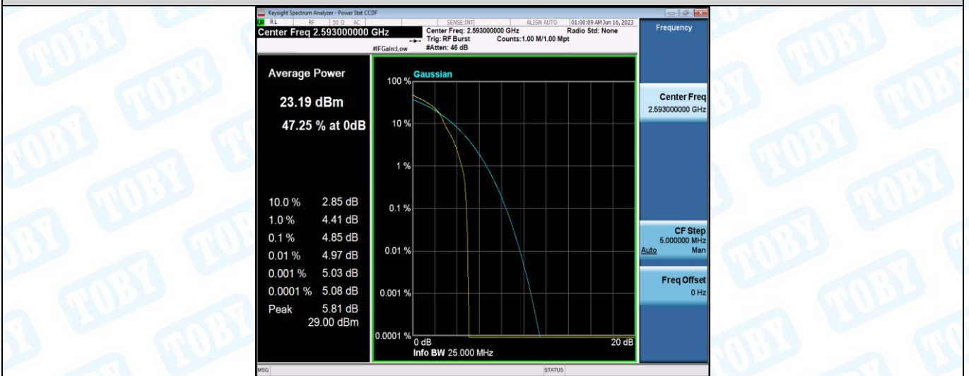
Band41-20MHz-16QAM-40620-100RB#0
