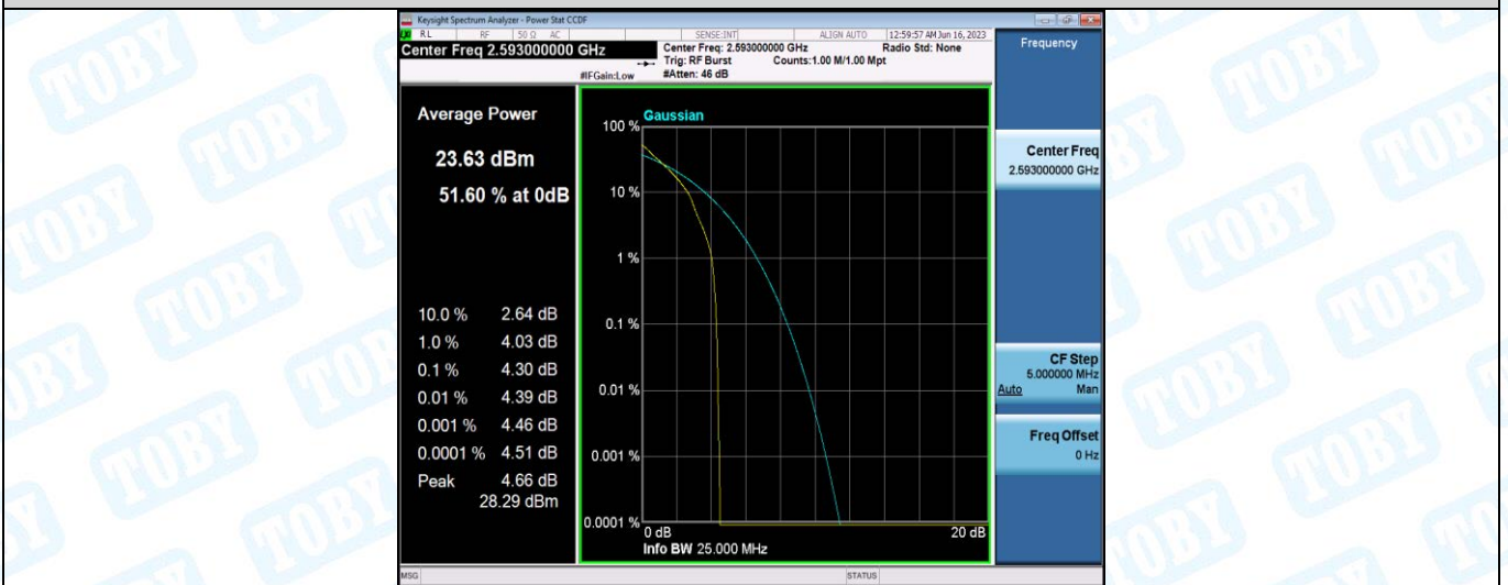
Band41-20MHz-QPSK-40620-100RB#0
