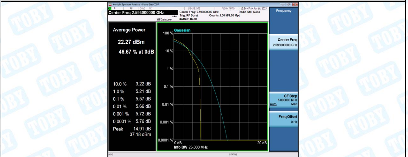
Band41-15MHz-16QAM-40620-75RB#0
