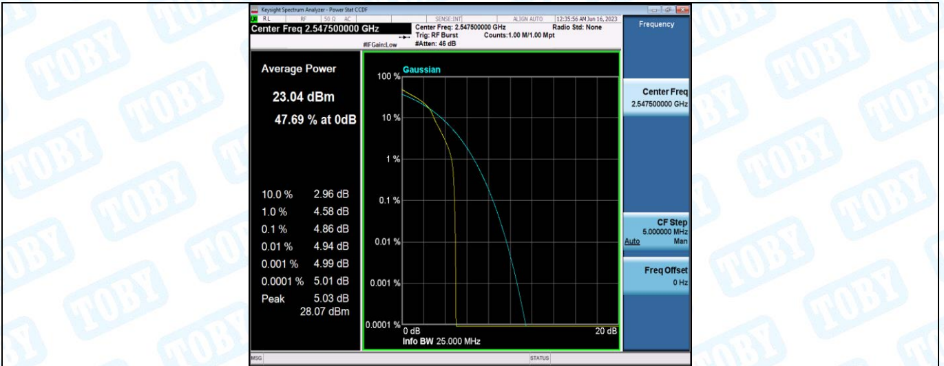
Band41-15MHz-16QAM-40165-75RB#0
