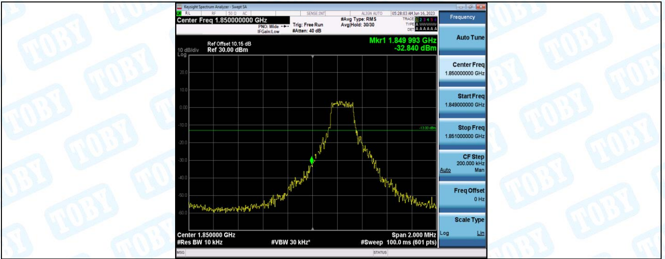
Band25-3MHz-QPSK-26055-1RB#14
