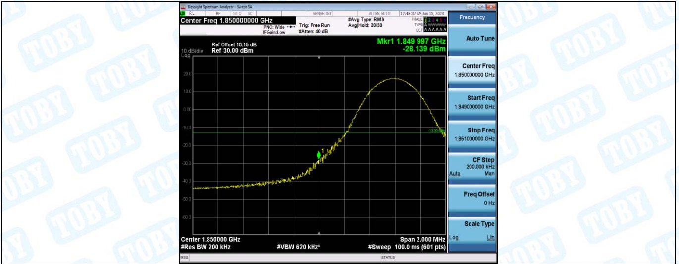
Band25-10MHz-QPSK-26090-1RB#49
