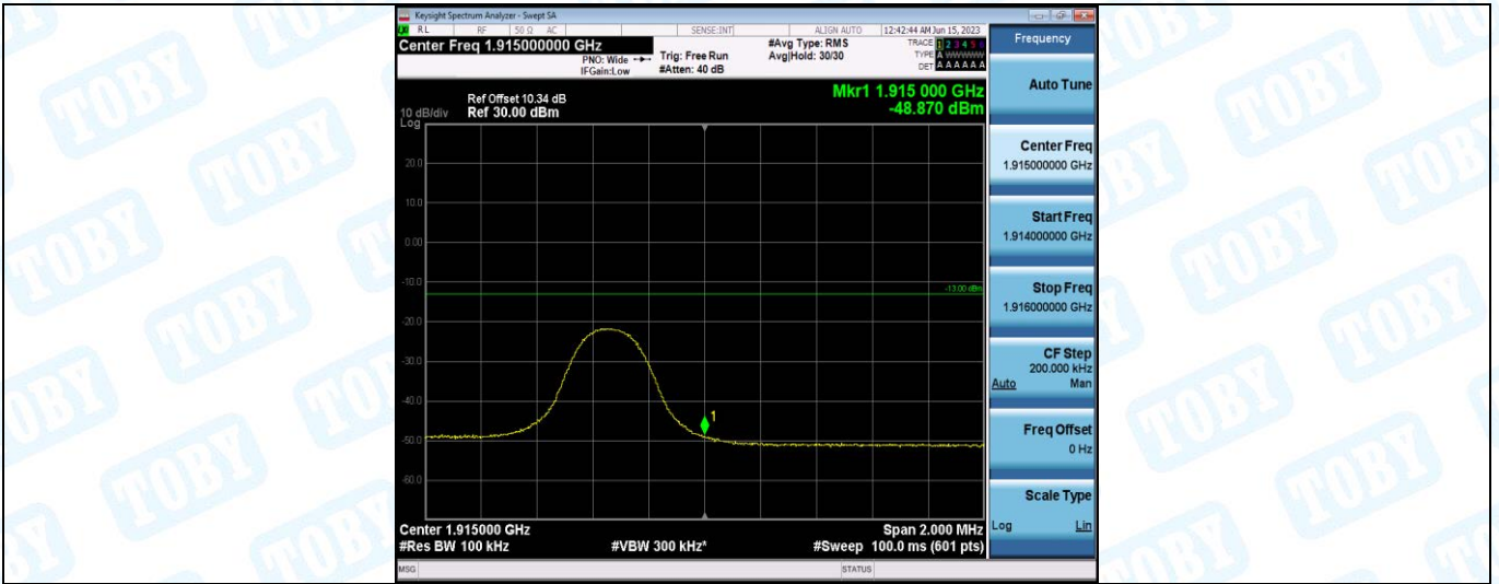
Band25-5MHz-16QAM-26665-1RB#24
