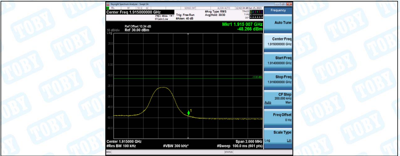
Band25-5MHz-QPSK-26665-1RB#24
