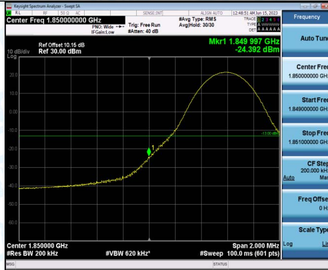
Band25-10MHz-16QAM-26090-1RB#49
