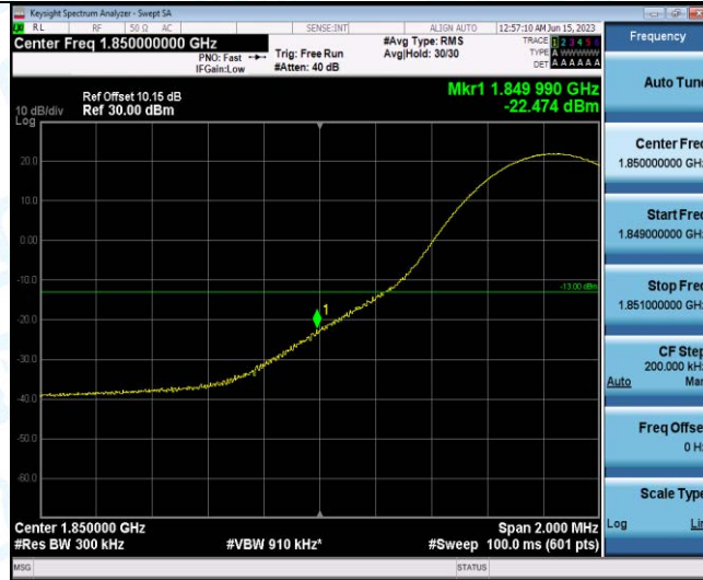
Band25-15MHz-16QAM-26115-1RB#74
