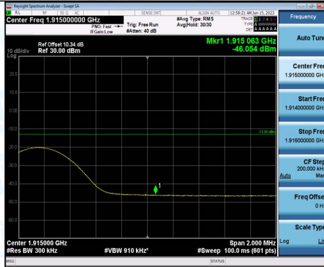
Band25-15MHz-16QAM-26615-1RB#74
