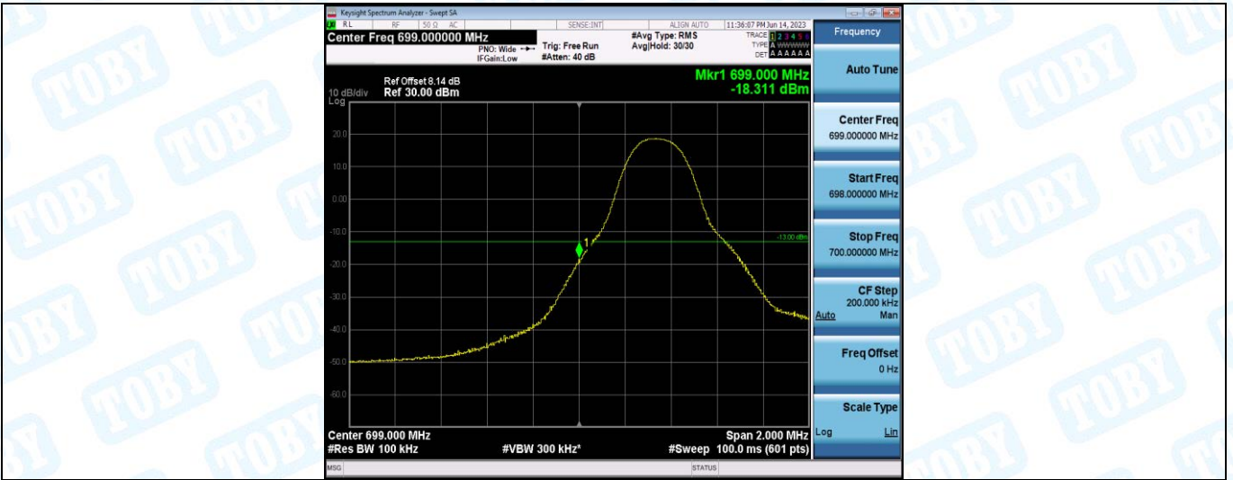
Band12-5MHz-QPSK-23035-1RB#24
