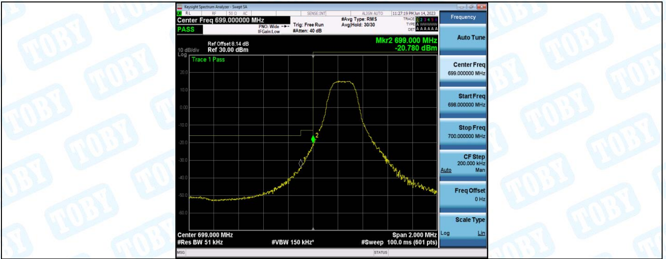
Band12-3MHz-16QAM-23025-1RB#14
