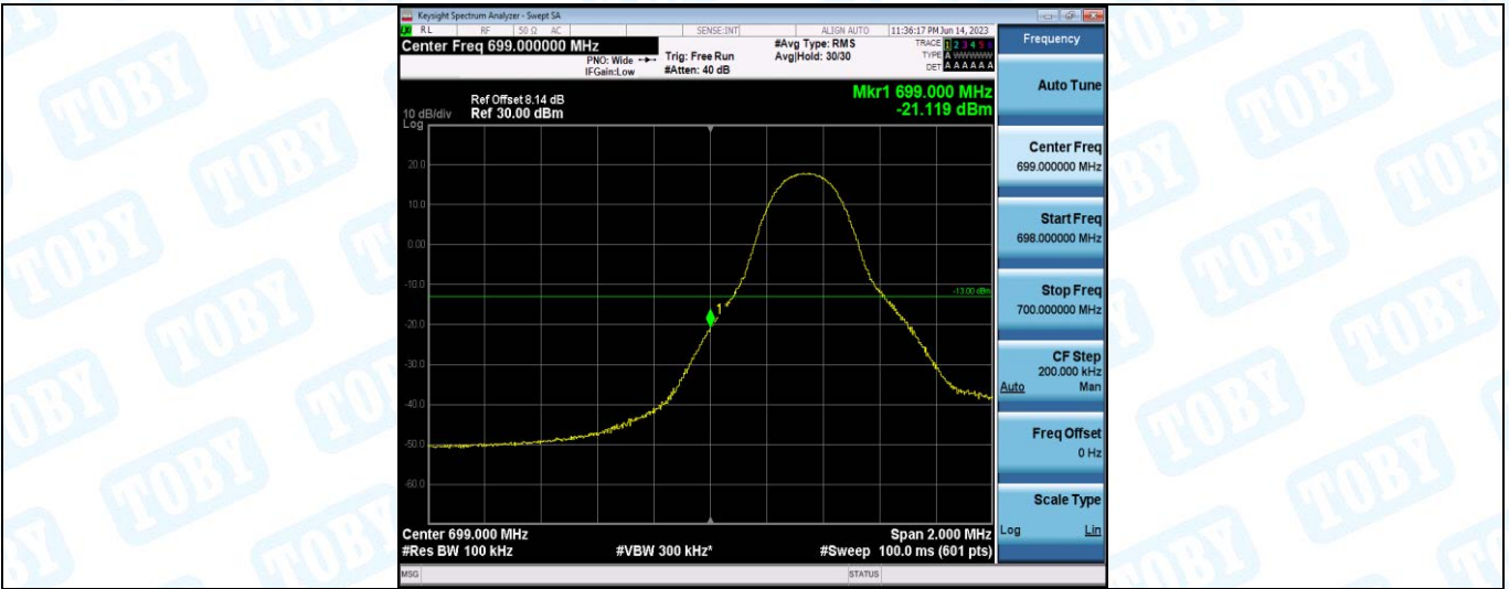
Band12-5MHz-16QAM-23035-1RB#24
