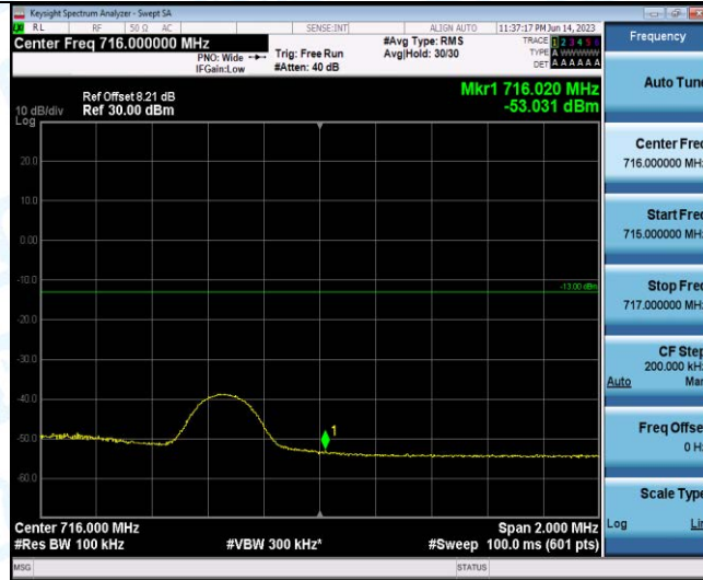
Band12-5MHz-QPSK-23155-1RB#24
