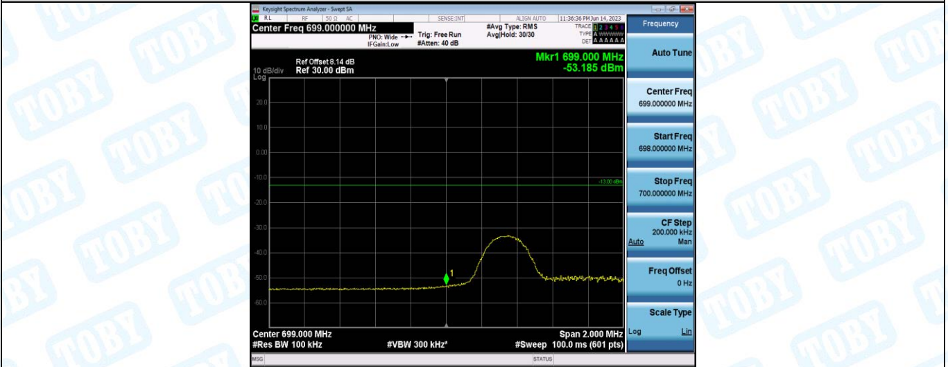
Band12-5MHz-16QAM-23035-25RB#0
