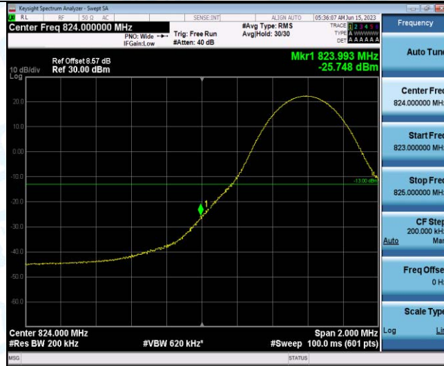
Band5-10MHz-QPSK-20450-1RB#49
