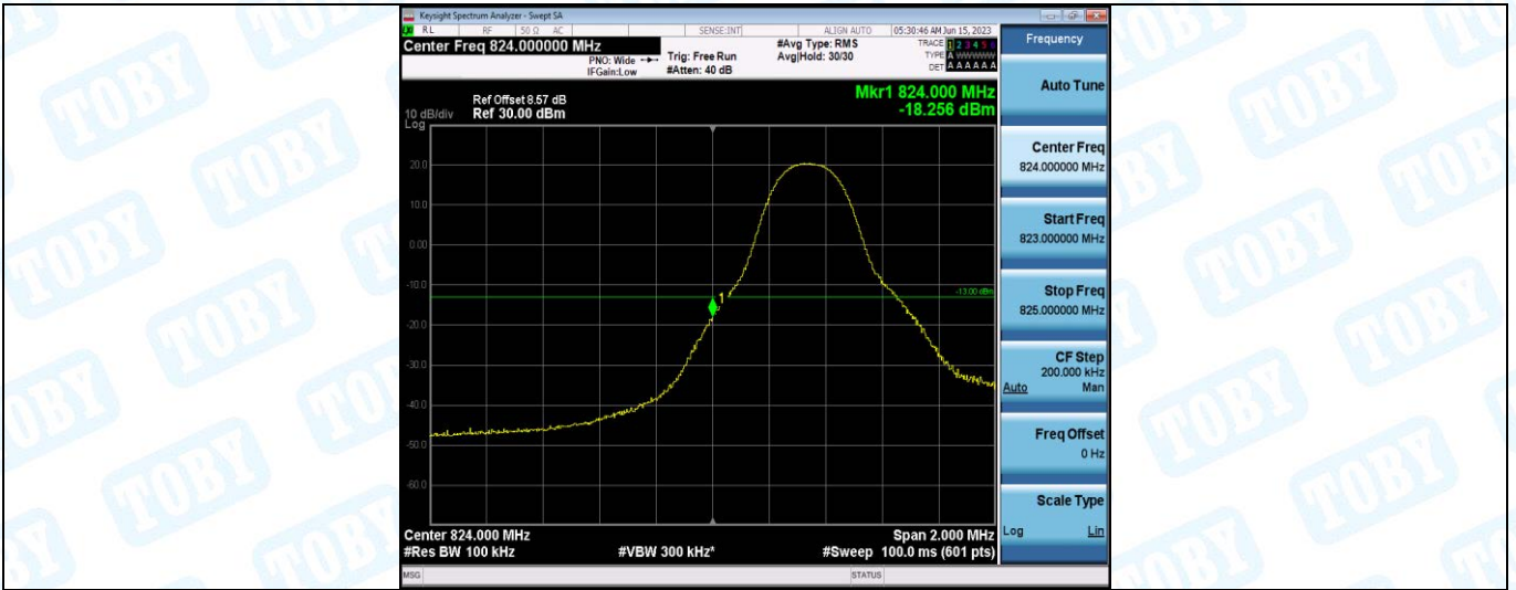
Band5-5MHz-QPSK-20425-1RB#24
