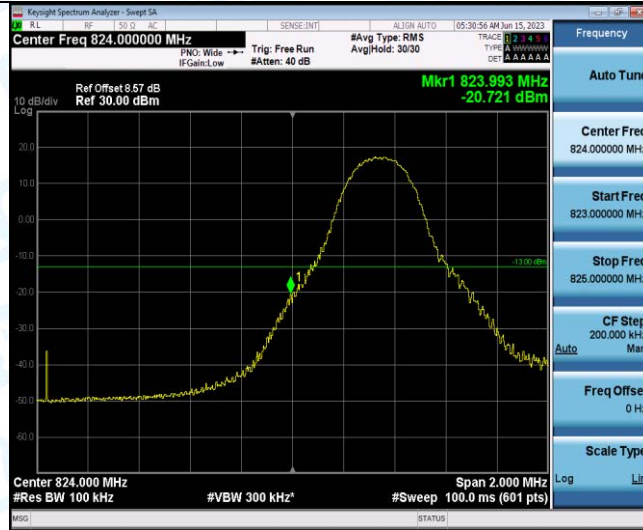
Band5-5MHz-16QAM-20425-1RB#24
