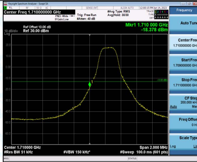
Band4-3MHz-16QAM-19965-1RB#14
