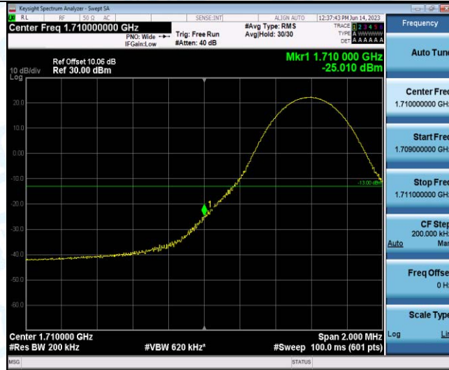
Band4-10MHz-16QAM-20000-1RB#49
