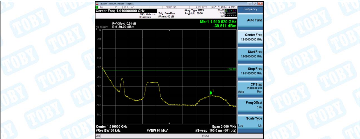
Band2-1.4MHz-16QAM-19193-1RB#5
